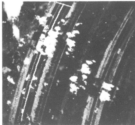
FIGURE 5(a) THE HIGH RESOLUTION ROAD TRACKER FOLLOWING A ROAD IN THE PRESENCE OF CLOUD COVER
