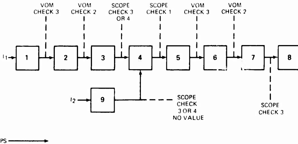
Figure 5. Data Flow Drawing with Optimal Solution and Necessary Test Equipment Indicated
