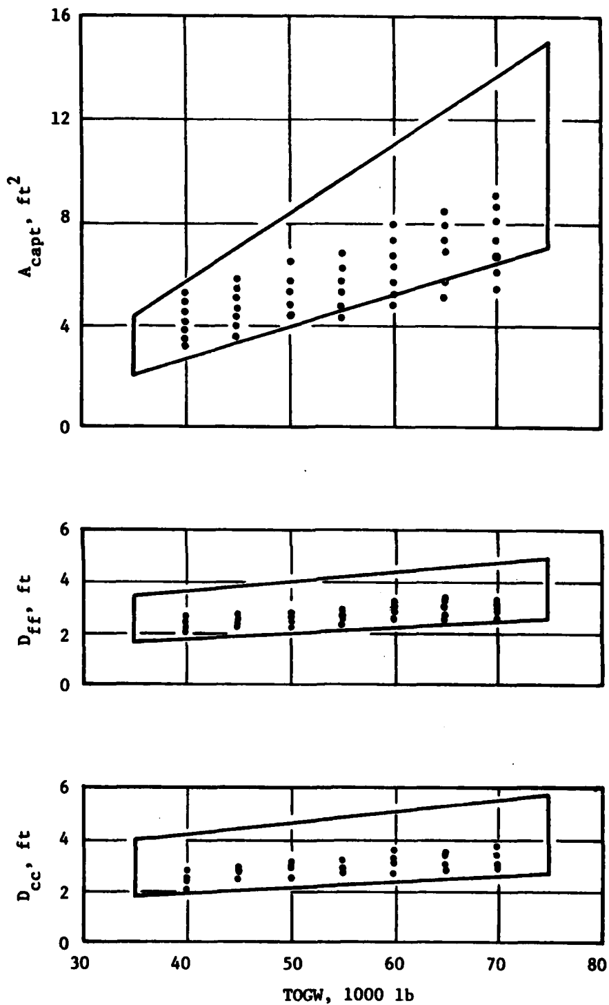
Figure 12. Variation of Engine Geometry Characteristics, RSTEP/ARM Studies.
