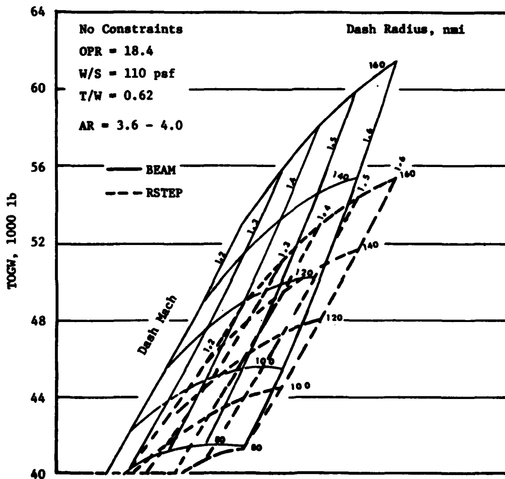
Figure 13. TOGW Sensitivity to Radius and Dash Mach Number, ARES Interrogation Results - Turbojet BEAM/ARES Vs. RSTEP/ARES.
