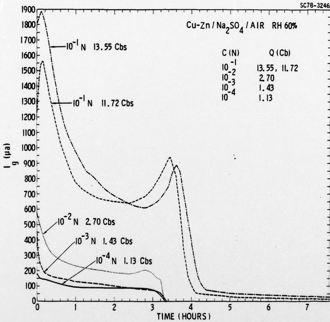
Fig. 31 Current at \Delta E = \pm 30 mV for Cu/zinc during drying out as a function of Na 2 SO 4 concentration. RH = 60%, T = 21 ± 1°C.
