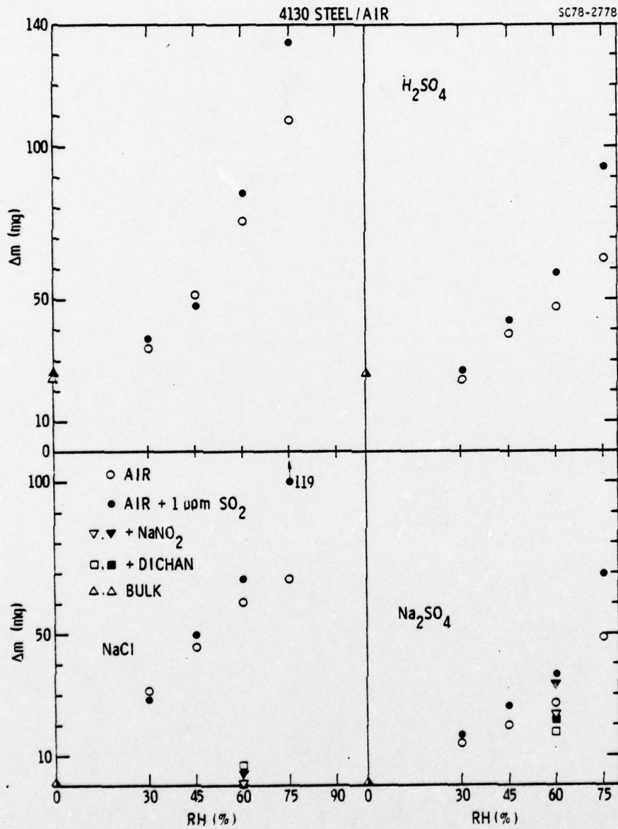
Fig. 20 Weight loss data for 413U steel in bulk and under thin layer electrolytes.
