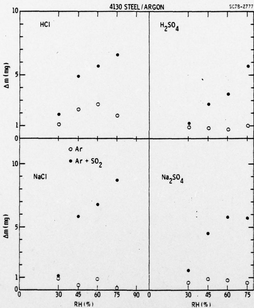
Fig. 20 Weight loss data for 413U steel in bulk and under thin layer electrolytes.
