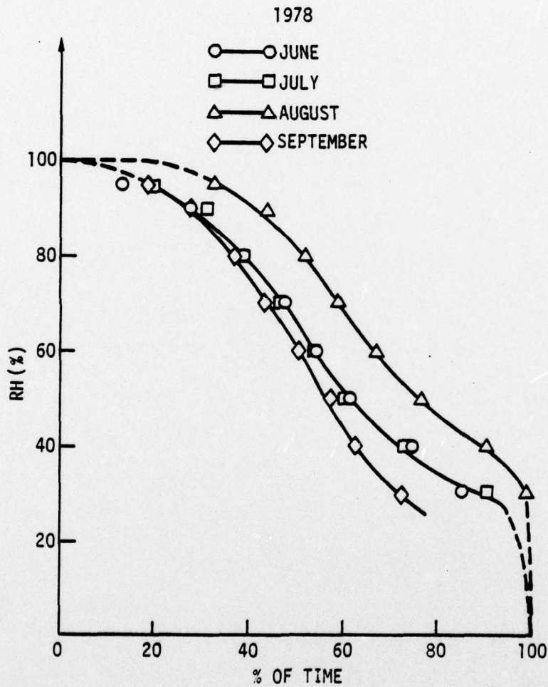
Fig. 43. Distribution of RH as a function of time for June to September 1978.
