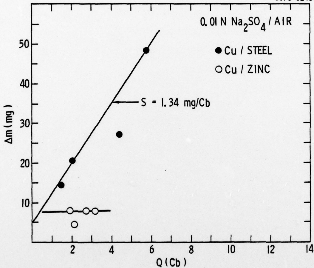
Fig. 34b Correlation between weight loss ( \Delta m ) and electrochemical ( Q ) data for steel and zinc (Fig. 34a) and Cu/steel and Cu/zinc (Fig. 34b) in 0.01N Na 2 SO 4 at different RH-values.
