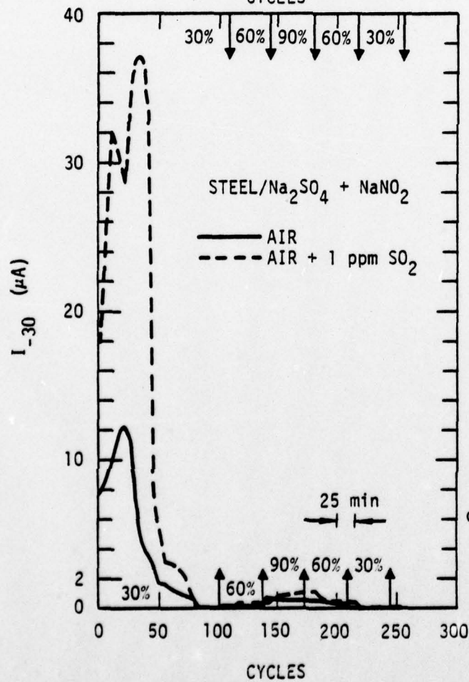
Fig. 19 Current flow for 4130 steel under solutions containing inhibitor exposed to air and air + 1 ppm \text{SO}_2 at varying RH.
