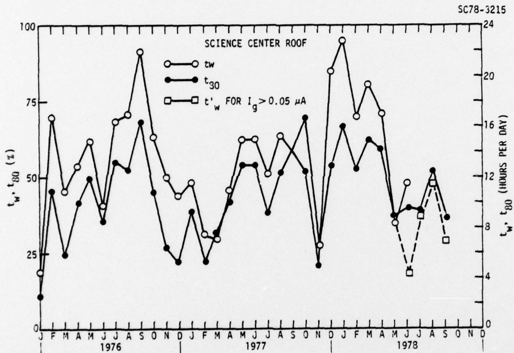
Fig. 40 Monthly averages of the time-of-wetness t_w and the time t_{80} for which RH exceeds 80%, Science Center roof.
