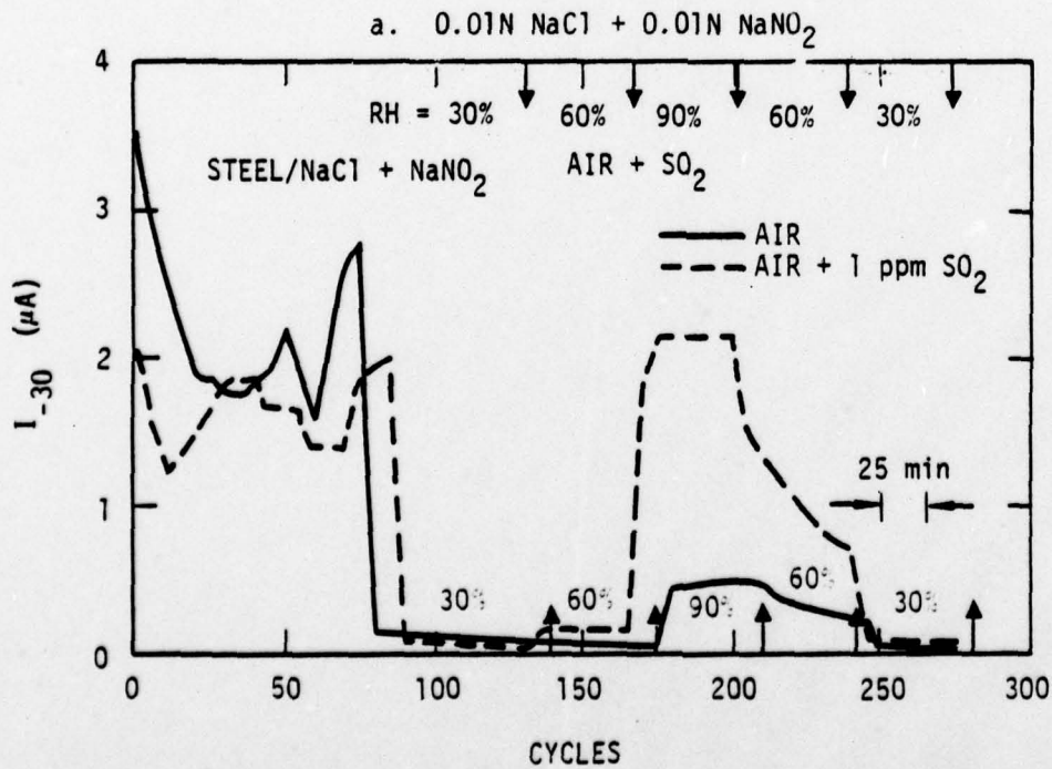
Fig. 19 Current flow for 4130 steel under solutions containing inhibitor exposed to air and air + 1 ppm \text{SO}_2 at varying RH.
