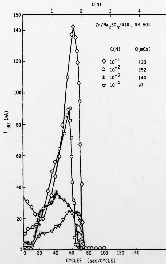
Fig. 30 Current at \Delta E = \pm 30 mV for zinc during drying out as a function of \text{Na}_2\text{SO}_4 concentration. RH = 60%, T = 21 \pm 1^\circ\text{C} .
