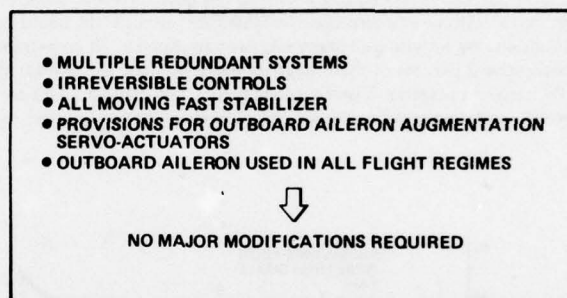
Figure 20. Adaptability of the L-1011 to Accept Active Controls Technology
