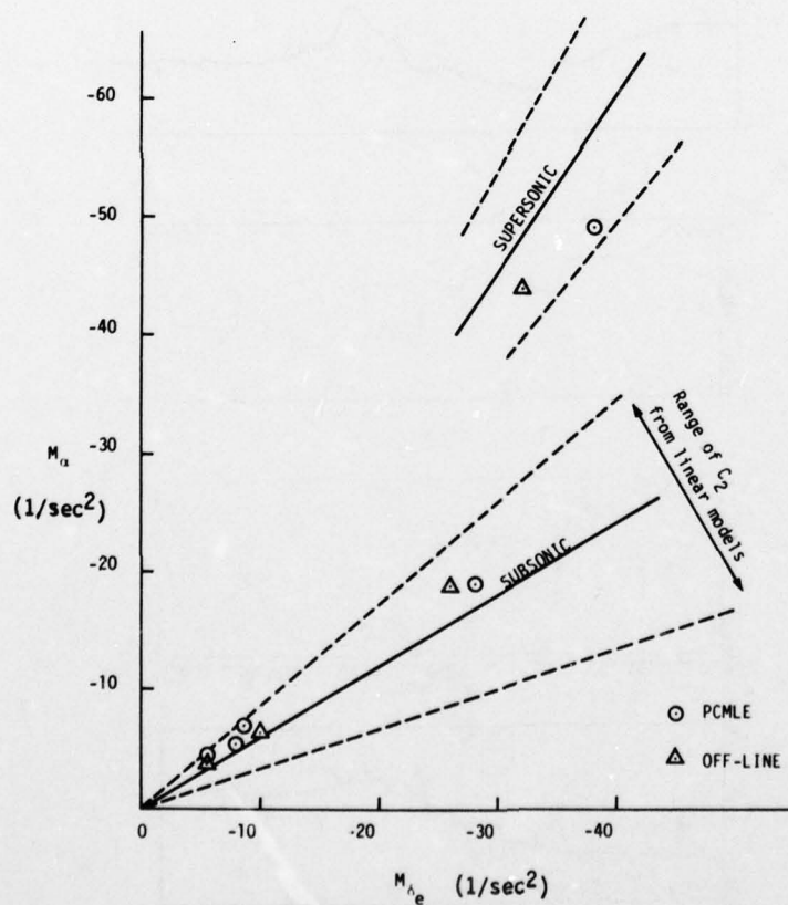
Figure 21. M_\alpha versus M_{\delta e}
