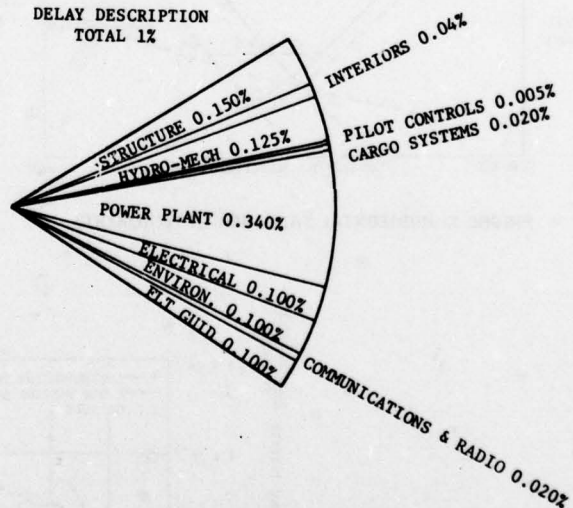
FIGURE 7. DISPATCH RELIABILITY
