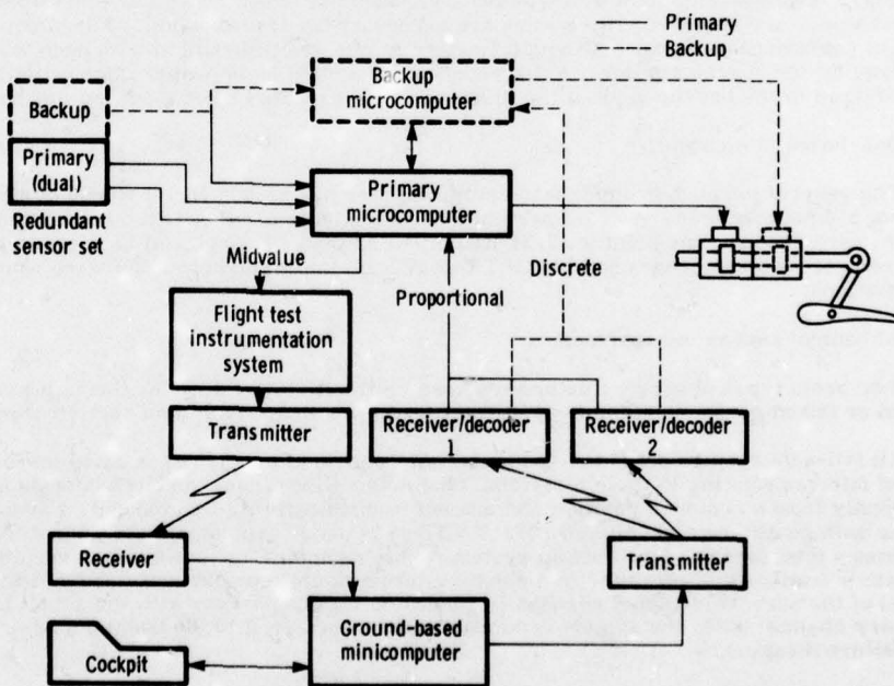
Figure 14. Arrangement of flight control system.
