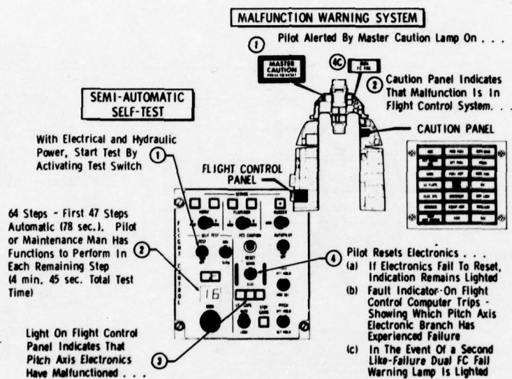
Figure 5 Flight Control Warning and Semi-Automatic, Self-Test System
