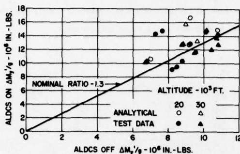
Figure 13 - Maneuver Loads - W.S. 198 Torsion
