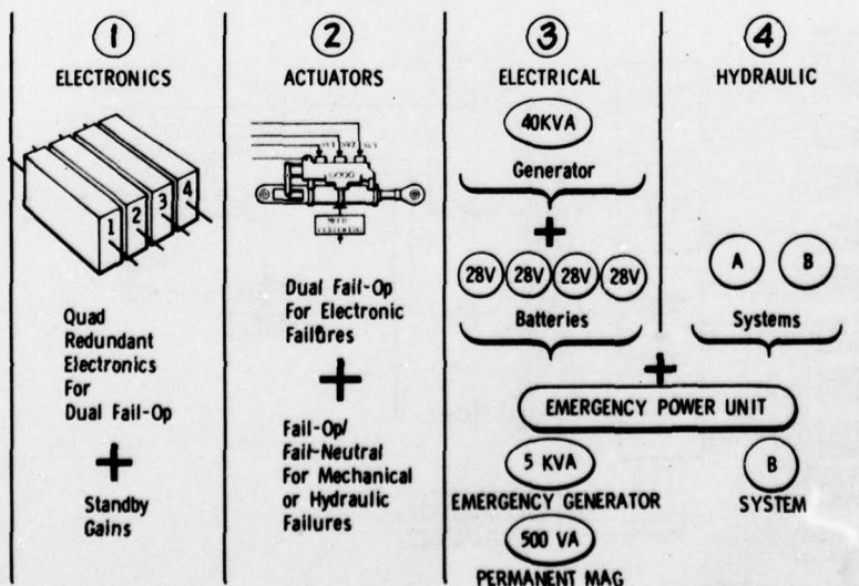
Figure 6 Flight Control System Redundancy Concept
