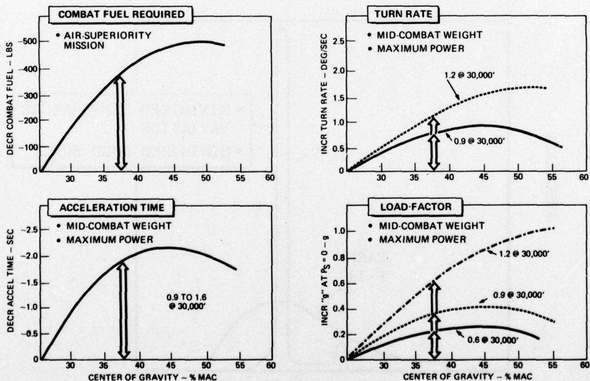
Figure 17 Performance Benefits Derived from Relaxed Static Stability
