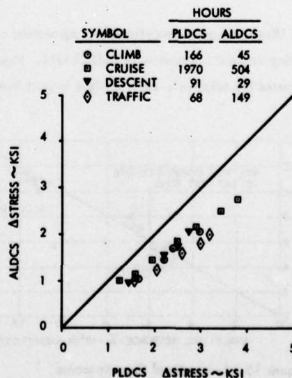
Figure 19 - Maneuver Axial Stress Comparison
