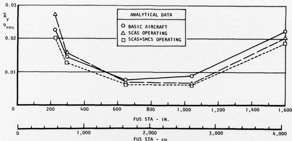
Figure 11. Effect of SMCS on Lateral Load Factor Response Along Fuselage Due to Turbulence, M = 0.85 , h_p = 762 m (2,500 Ft), A_w = 65^\circ , Medium Weight
