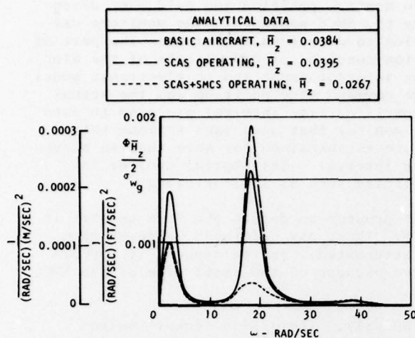
Figure 8. Power Spectral Density Associated With Vertical Crew Sensitivity Index, \bar{H}_z , M = 0.85 , h_p = 762 m (2,500 FT), \Lambda_w = 65^\circ , Medium Weight
