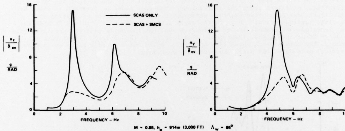
Figure 22. Performance of SMCS With Relocated Forward Sensor Package, FS 516 (203) Flight Test Data
