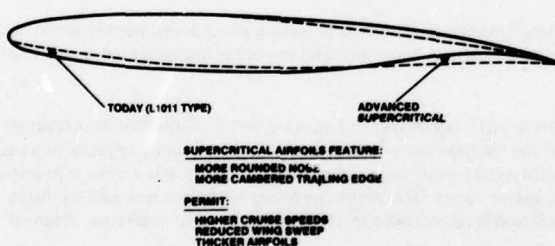
Figure 5. Advanced Airfoils
