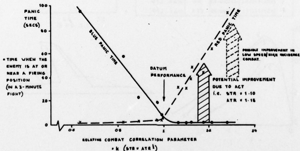
FIG 10 COMBAT CORRELATION FOR STUDY AIRCRAFT (LOW LEVEL ENGAGEMENTS)
