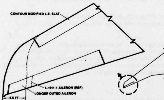
Figure 25. Extended Span Wing
