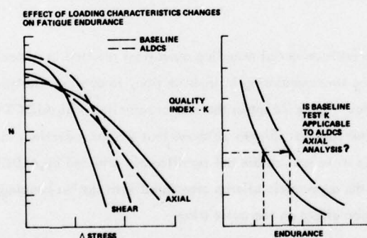
Figure 24 - Analytical/Test Endurance Vs Quality Level
