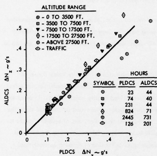
Figure 20 - Gust Load Factor Comparison
