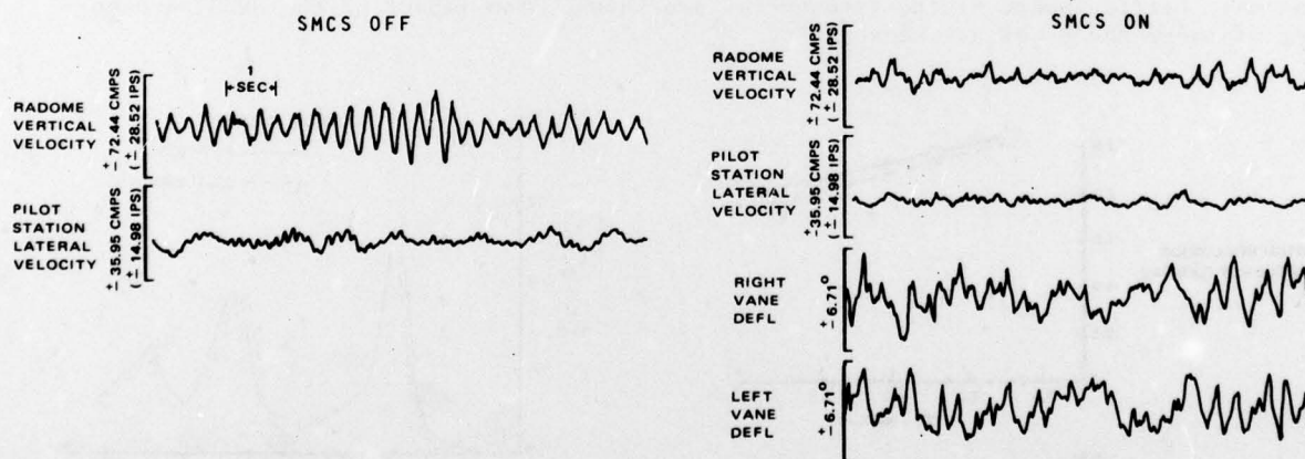
Figure 15. SMCS Performance in Turbulence M = 0.70 , h_{AGL} = 305 m (1,000 Ft). \Lambda_w = 65^\circ
