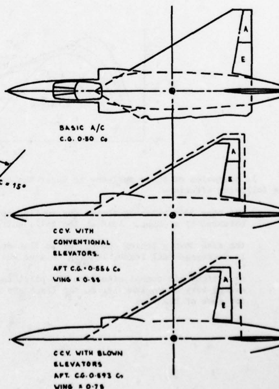
60° DELTA FIG 6 EFFECT OF ARTIFICIAL STABILITY ON WING SIZE
