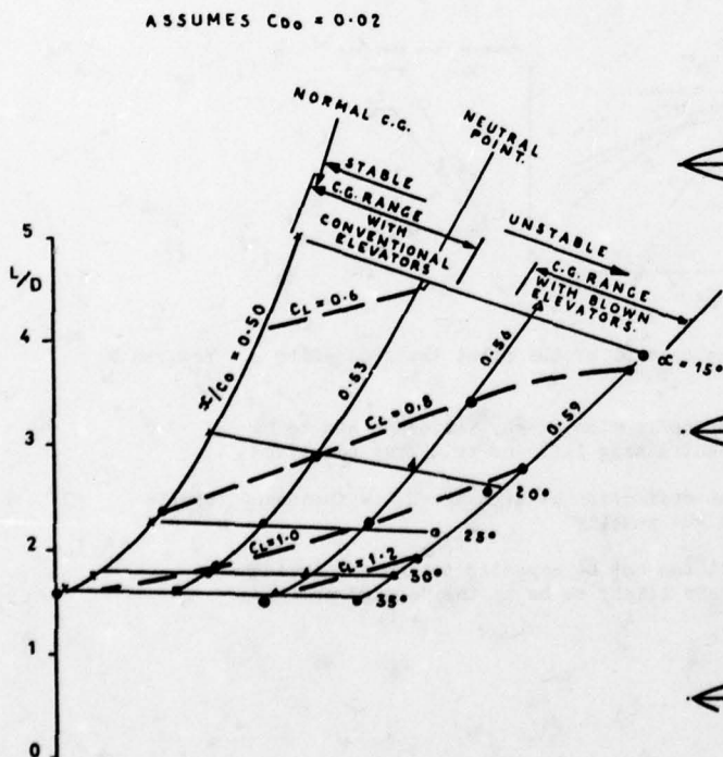
60° DELTA FIG 5 VARIATION OF TRIMMED LIFT/DRAG RATIO WITH C_L ( \alpha ) AND C.G. POSITION [SUBSONIC]
