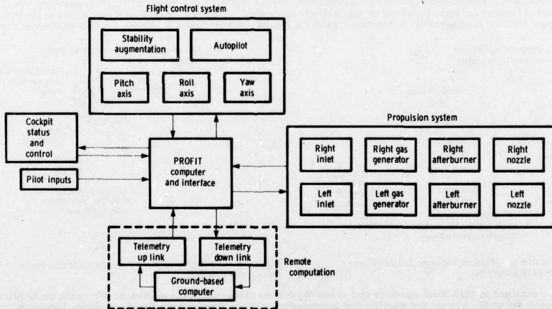
Figure 8. Block diagram of PROFIT system.
