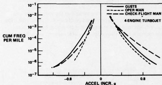
Figure 19. Gust and Maneuver Accelerations for Long-Haul Airplanes
