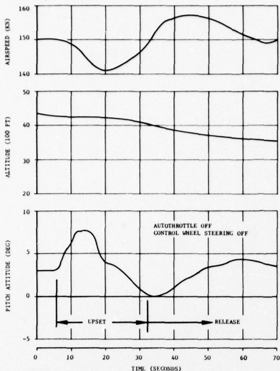
FIGURE 8a. APPROACH LONGITUDINAL STABILITY
