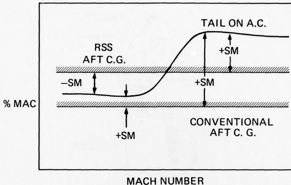
Figure 16 Aerodynamic Center Variation
