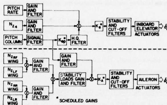
Figure 10 - ALDCS System Block Diagram
