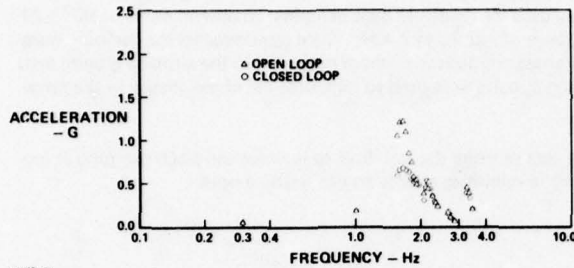
Figure 39. Active Control Effectiveness; Wing-Tip Response
