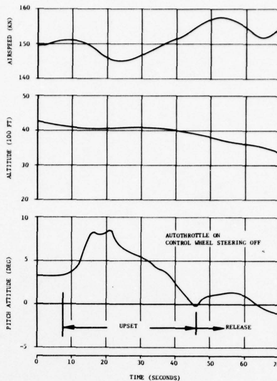
FIGURE 8b. APPROACH LONGITUDINAL STABILITY
