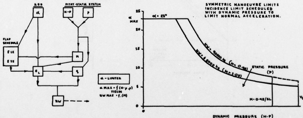
FIG 13 OVERSTRESSING PREVENTION
