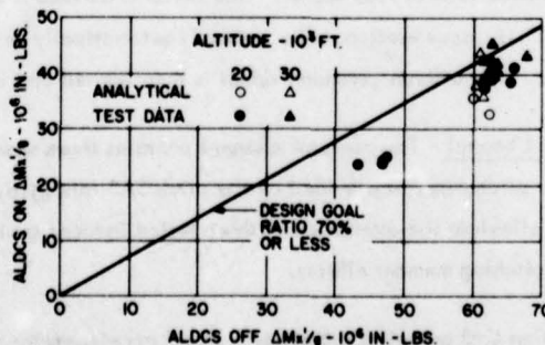
Figure 12 - Maneuver Loads - W.S. 198 Bending
