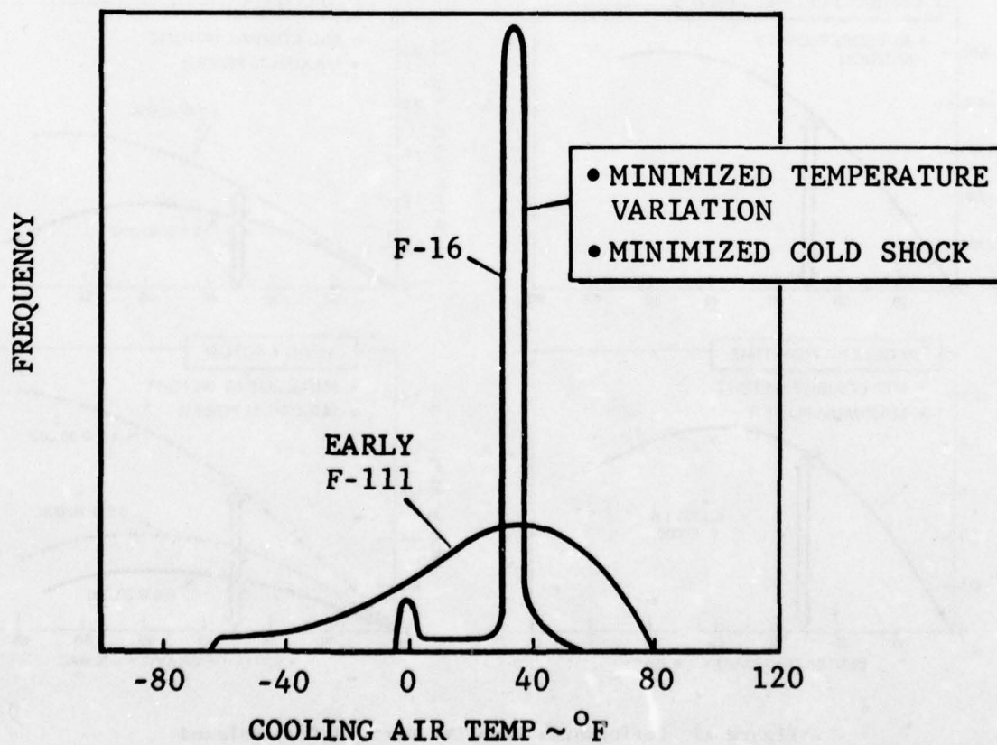
Figure 19 F-16 In-Flight Cooling Air Supply Temperature Characteristics
