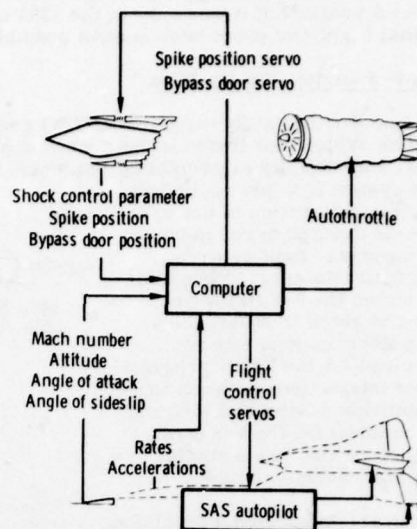
Figure 7. YF-12 cooperative control schematic.
