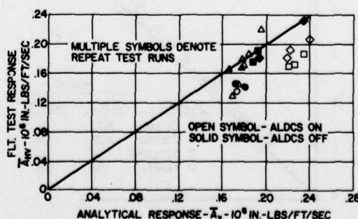
Figure 16 - Normalized Gust Response - W.S. 198 Torsion
