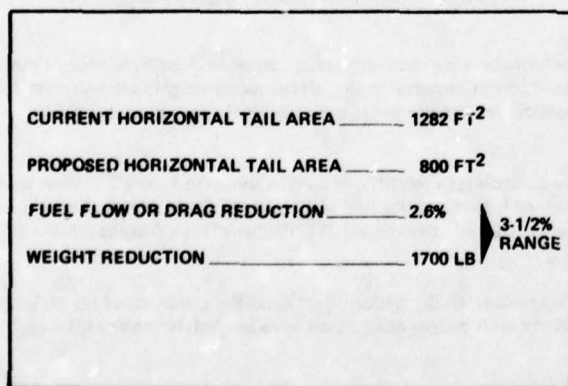
Figure 15. Relaxed Static Stability Impact on Fuel Savings
