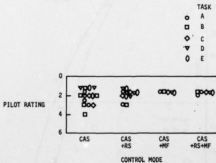
Figure 12. Pilot Ratings of Longitudinal Handling Qualities. Cooper-Harper Scale; Table 5 Defines Tasks; Mach 0.6; 6100 Meters
