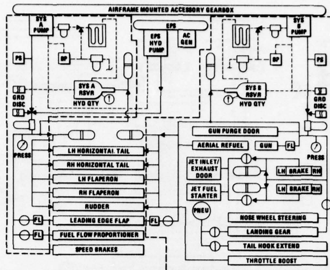
Figure 12 Hydraulic Power Subsystem Block Diagram
