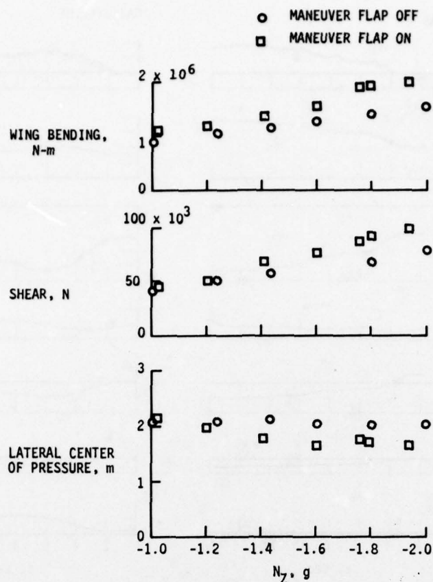
Figure 11. Wing Bending and Shear Load Variation
