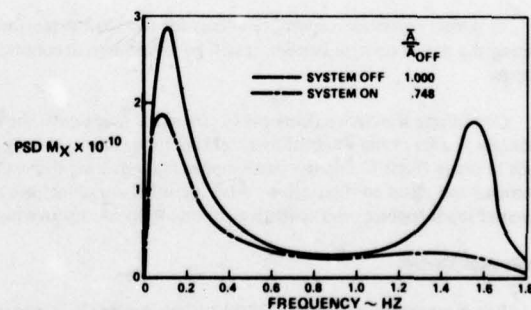
Figure 26. Power Spectral Density of Wing Bending Moment at Gust-Critical Wing Station
