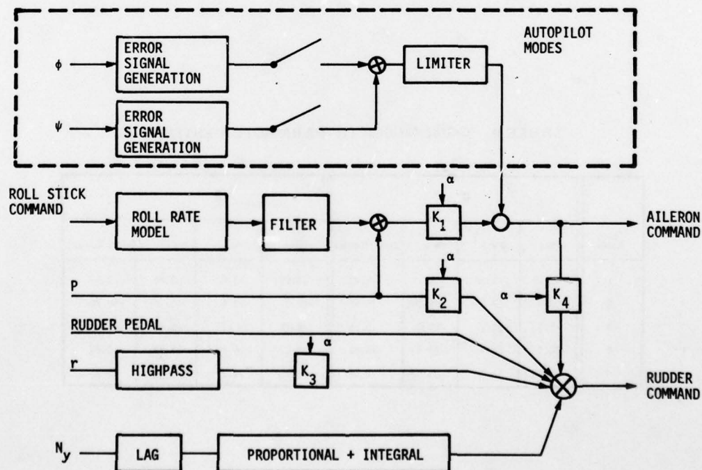
Figure 3. Functional Diagram for F-8 Lateral/Directional SAS
