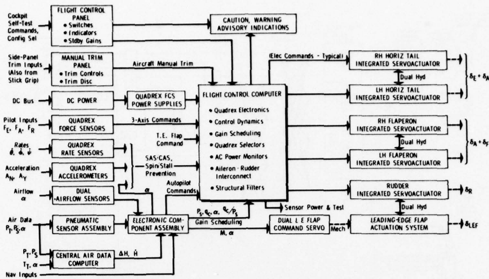
Figure 4 Flight Control System Functional Schematic
