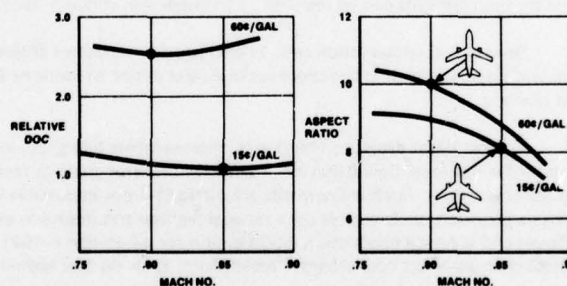
Figure 6. Wing Geometry Trades
