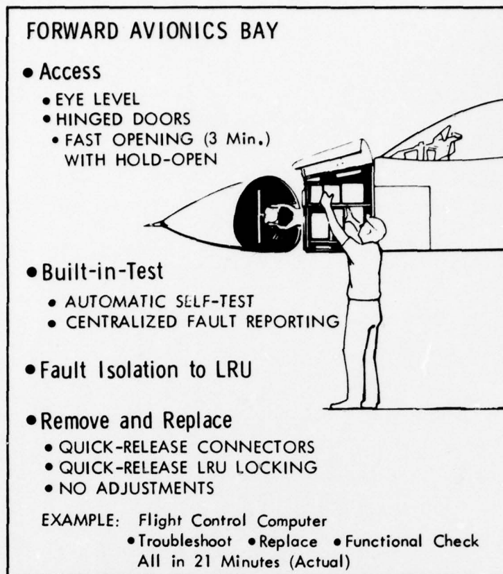
Figure 20 Avionic Equipment Accessibility
