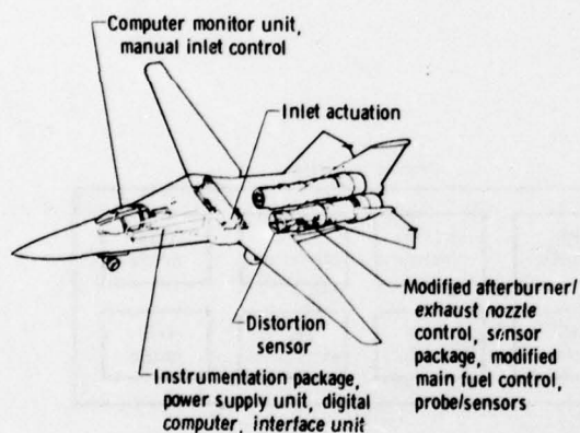
Figure 5. IPCS equipment installed on F-111E airplane.
