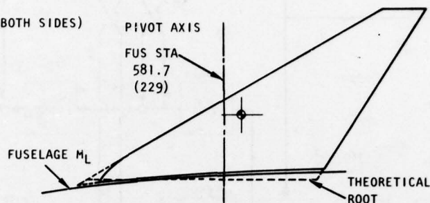
Figure 6. Structural Mode Control Vane Geometric Characteristics
