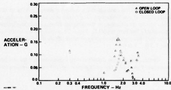
Figure 40. Active Control Effectiveness
