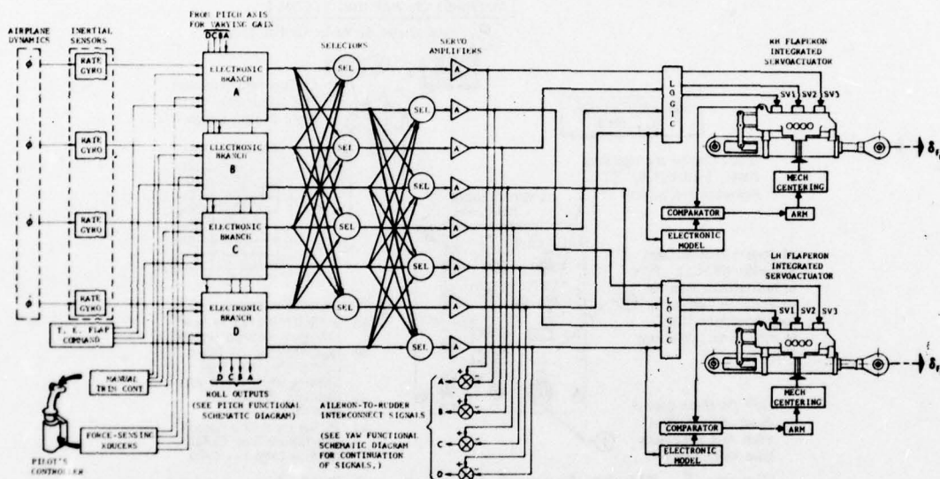
Figure 8 Roll Functional Schematic Diagram
