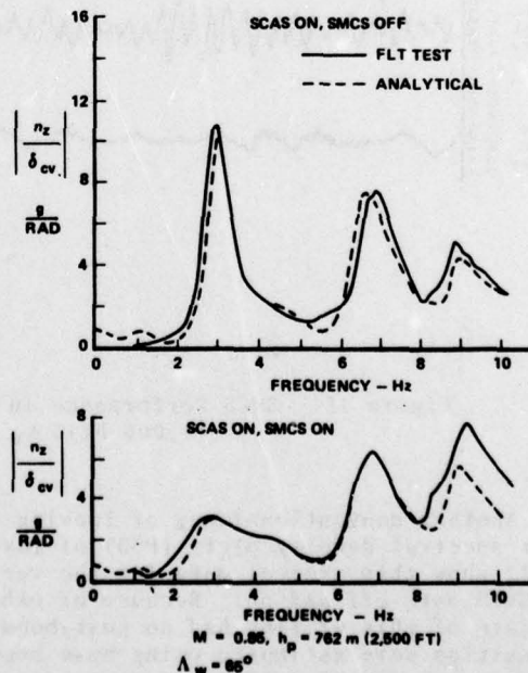
Figure 19. Comparison of Flight Test and Analytical Data, Frequency Response of Vertical Load Factor at FS 582 (229) Due to SMCS Vane Deflection
