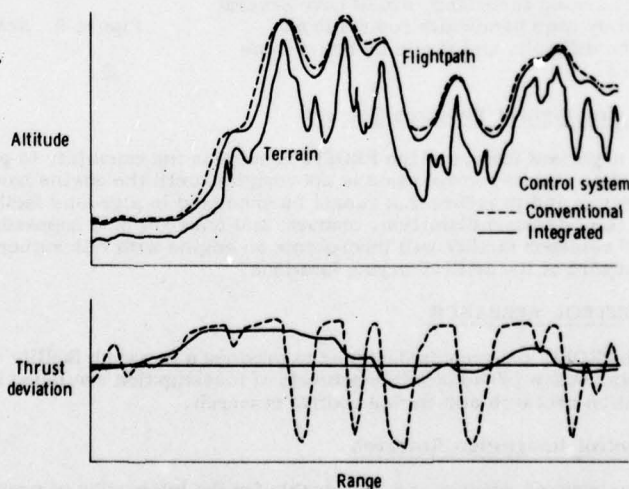
Figure 11. Comparison of altitude and thrust deviations for conventional control and integrated control optimized for terrain following.
