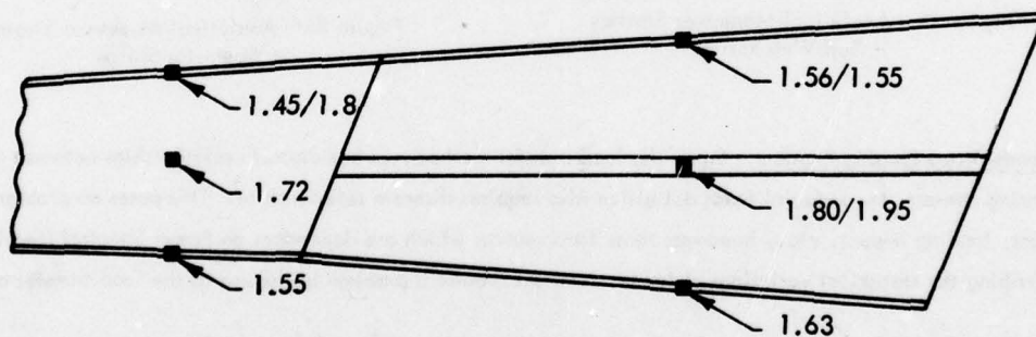
Figure 28 - ALDCS Life Improvement Factors
