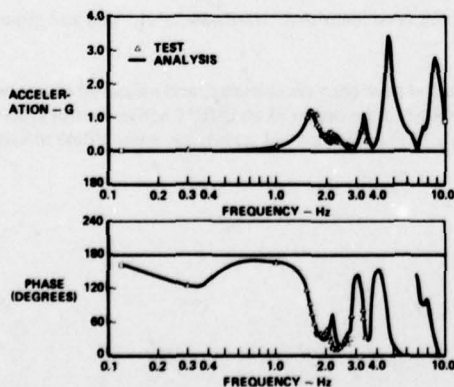
Figure 37. Wing-Tip Response to Aileron Drive, Open Loop
