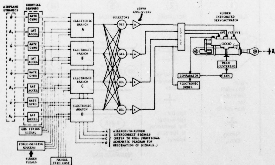
Figure 9 Yaw Functional Schematic Diagram
