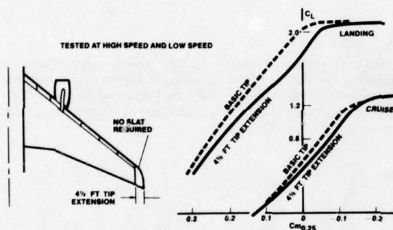
Figure 13. Effects of Tip Extension on L-1011 Pitch Characteristics
