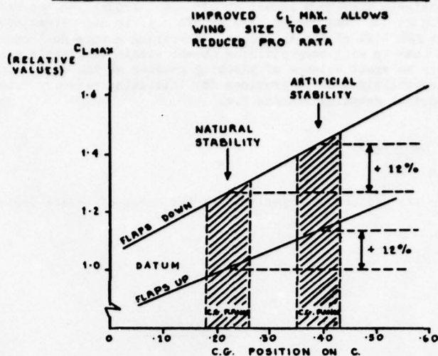
FIG 3 DRAG AND WEIGHT SAVINGS WITH ARTIFICIAL STABILITY
