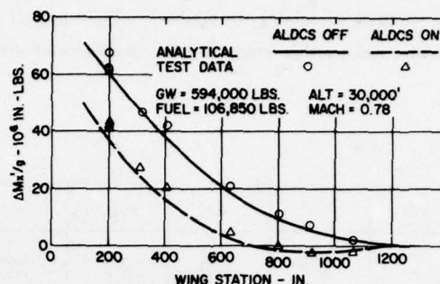
Figure 14 - Maneuver Loads - Spanwise Bending
