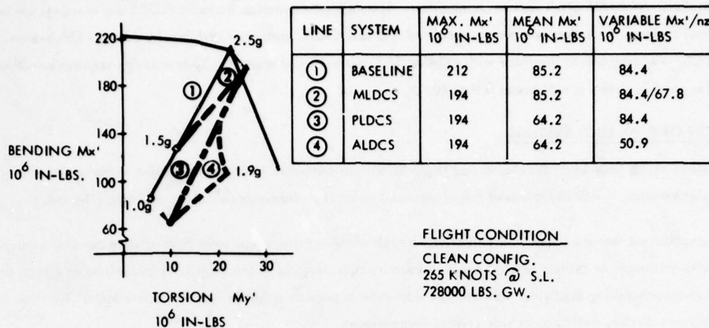
Figure 6 - Comparison of LDCS Loads
