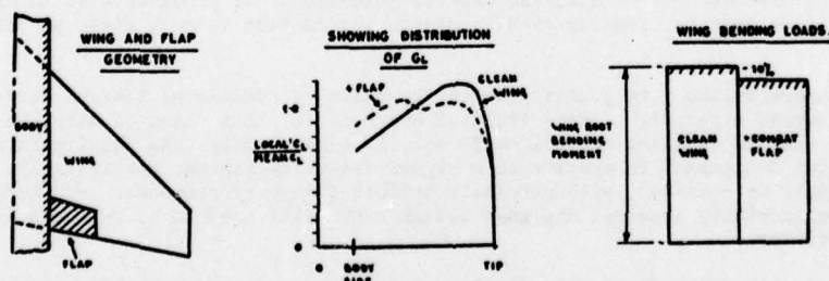
FIG 16 MANOEUVRE LOAD CONTROL
