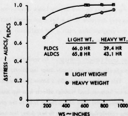
Figure 23 - Aerial Refueling Axial Stress Comparison
