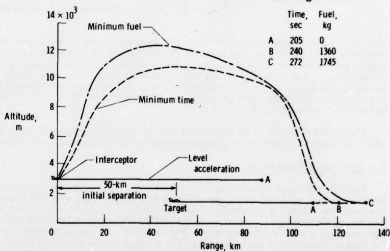
Figure 13. Energy management for intercept mission. Simulation data from Reference 2.
