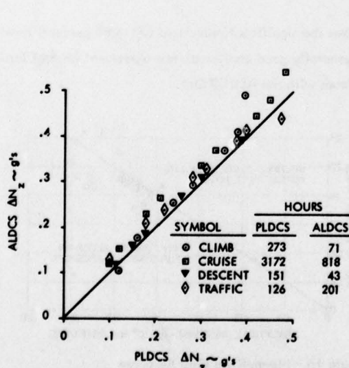
Figure 18 - Maneuver Load Factor Comparison
