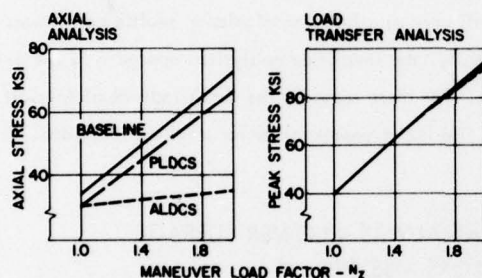
Figure 25 - Analytical Maneuver Stresses - Cap/Web Splice
