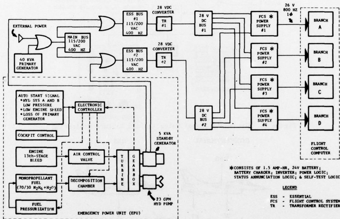
Figure 11 Flight Control System-Electrical Power Schematic Diagram
