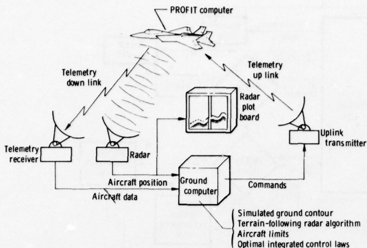
Figure 12. PROFIT concept as applied to optimal terrain-following problem.
