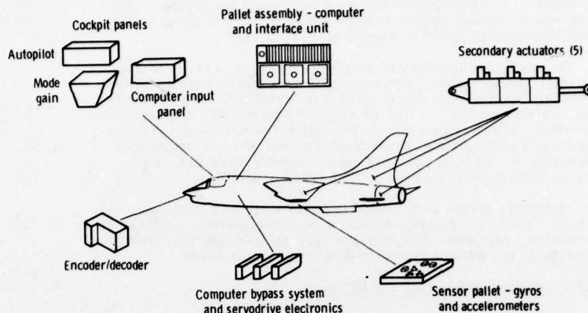
Figure 4. F-8 DFBW hardware elements.
