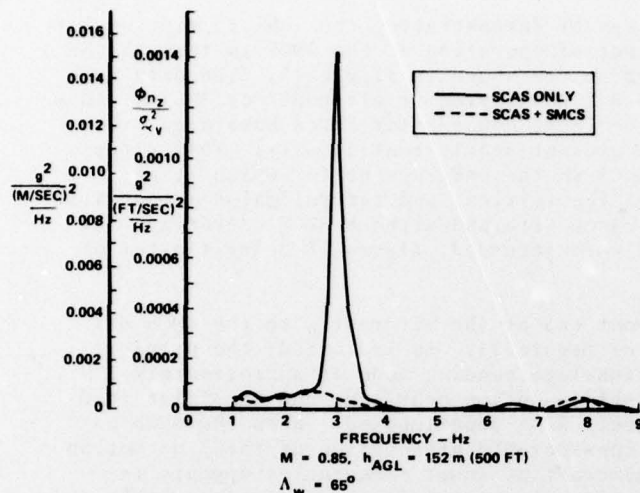
Figure 16. Vertical SMCS Performance in Turbulence as Shown by Power Spectral Density of Vertical Load Factor at Pilot Station
