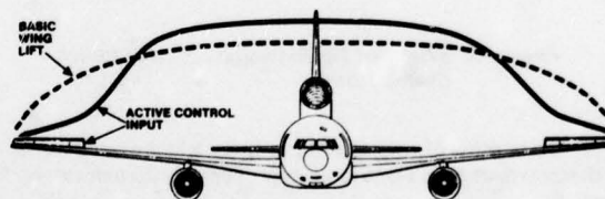
Figure 10. Load Redistribution with Active Controls
