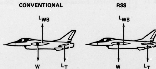
Figure 15 Supersonic Balance Comparison
