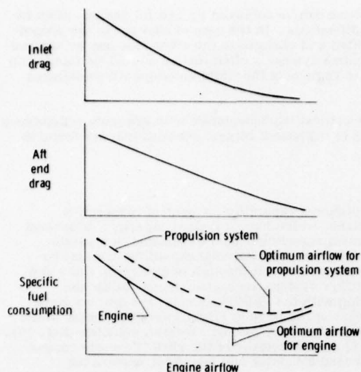
Figure 10. Engine-inlet-nozzle integration at partial power.
