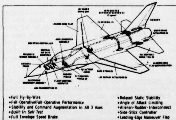
Figure 3 F-16A Flight Control/Stability and Control Features
