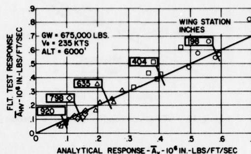
Figure 17 - Normalized Gust Response - Spanwise Bending
