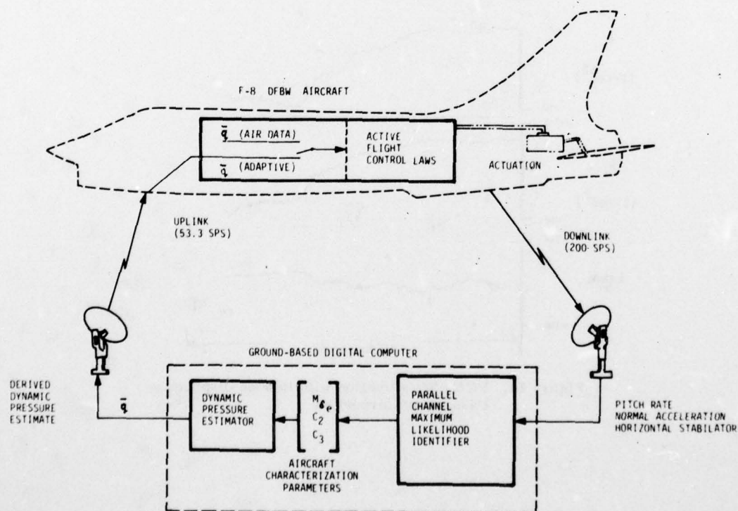
Figure 18. Adaptive Control Flight Test Approach
