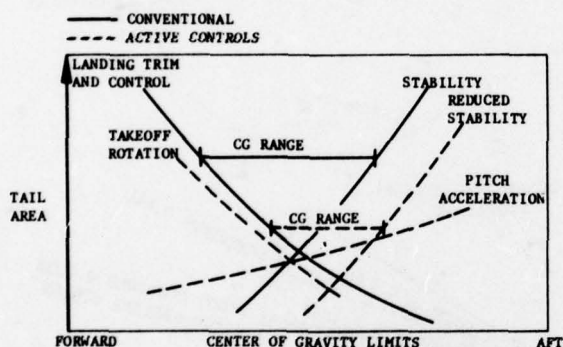
FIGURE 1. HORIZONTAL TAIL AREA REQUIREMENTS
