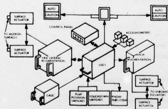
Figure 3 - MLDCS System Components
