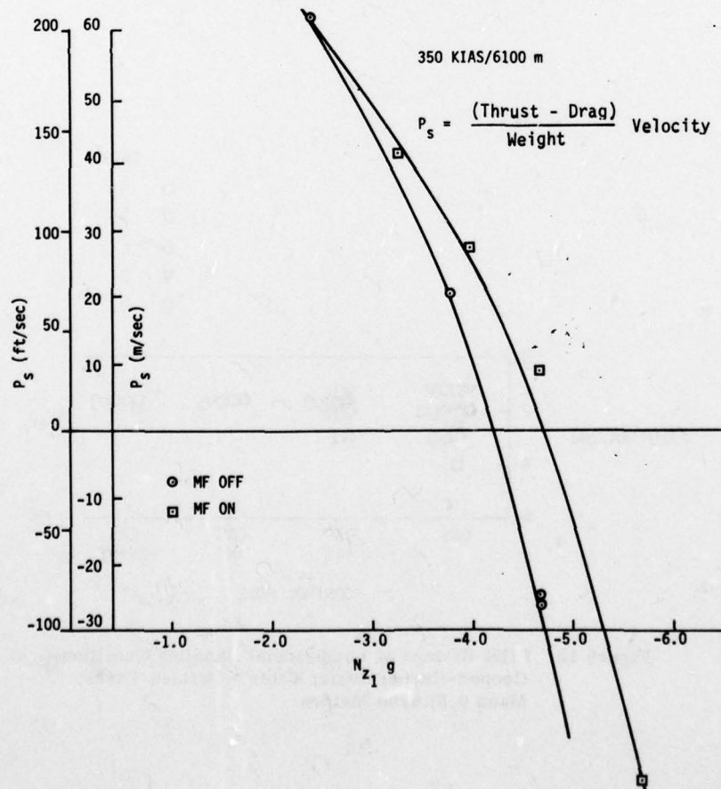
Figure 9. Wind-up Turn 350 KIAS at 6100 Meters
