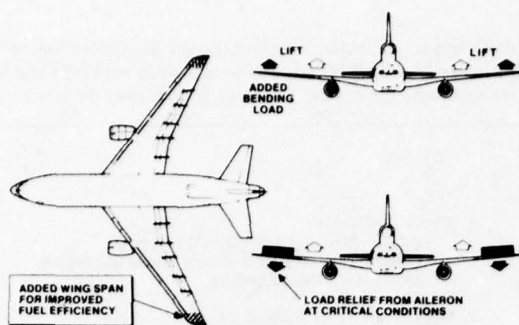
Figure 11. Active Controls for Fuel Conservation
