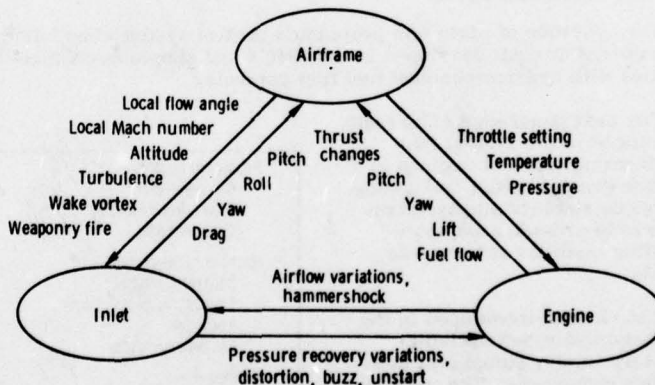
Figure 3. Engine-inlet-airframe interactions.
