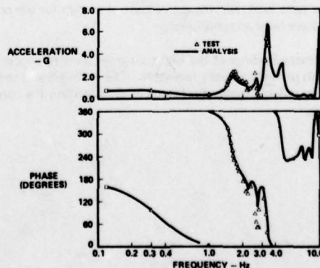
Figure 38. Wing-Tip Response to Stabilizer Drive, Open Loop
