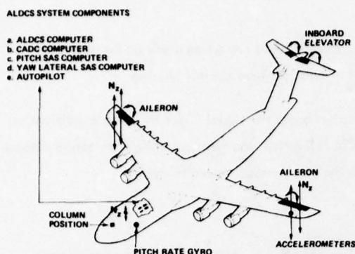
Figure 9 - ALDCS System Components
