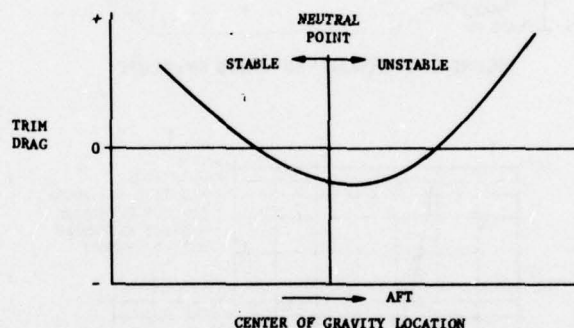
FIGURE 2. TRIM DRAG
