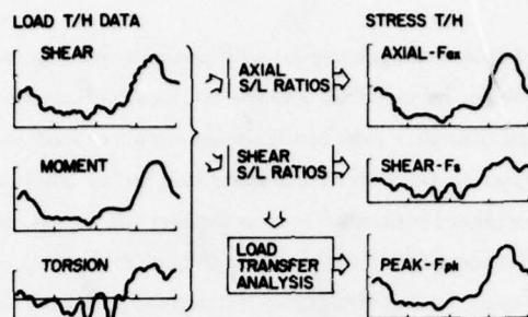
Figure 27 - Stress Time History Generation
