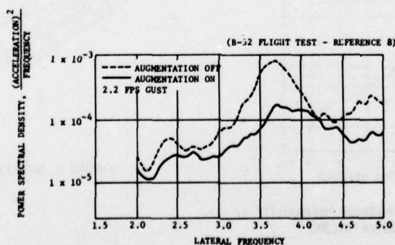
FIGURE 3. RIDE QUALITY IMPROVEMENT
