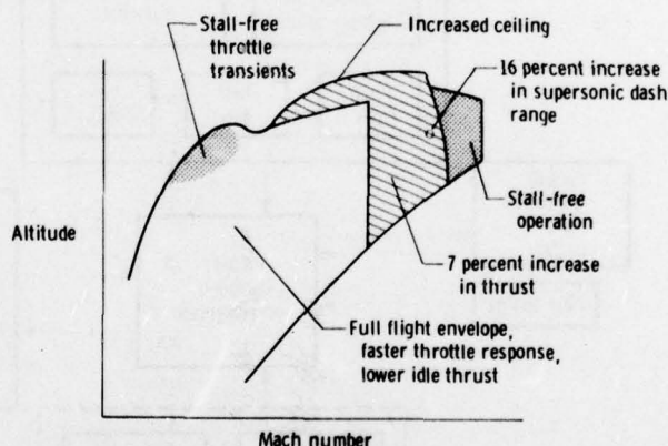
Figure 6. Summary of performance improvements from IPCS program.
