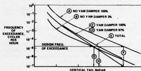
Figure 18. Frequency of Exceedance of Vertical Tail Shear With and Without Yaw Damper
