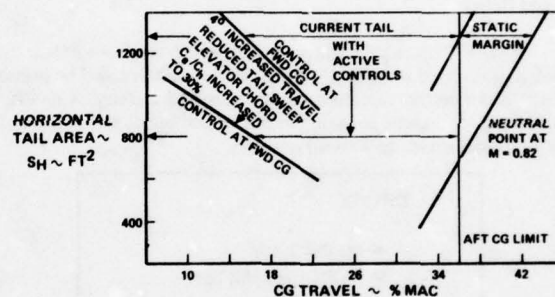
Figure 14. Benefits of Relaxed Static Stability on Tail Size
