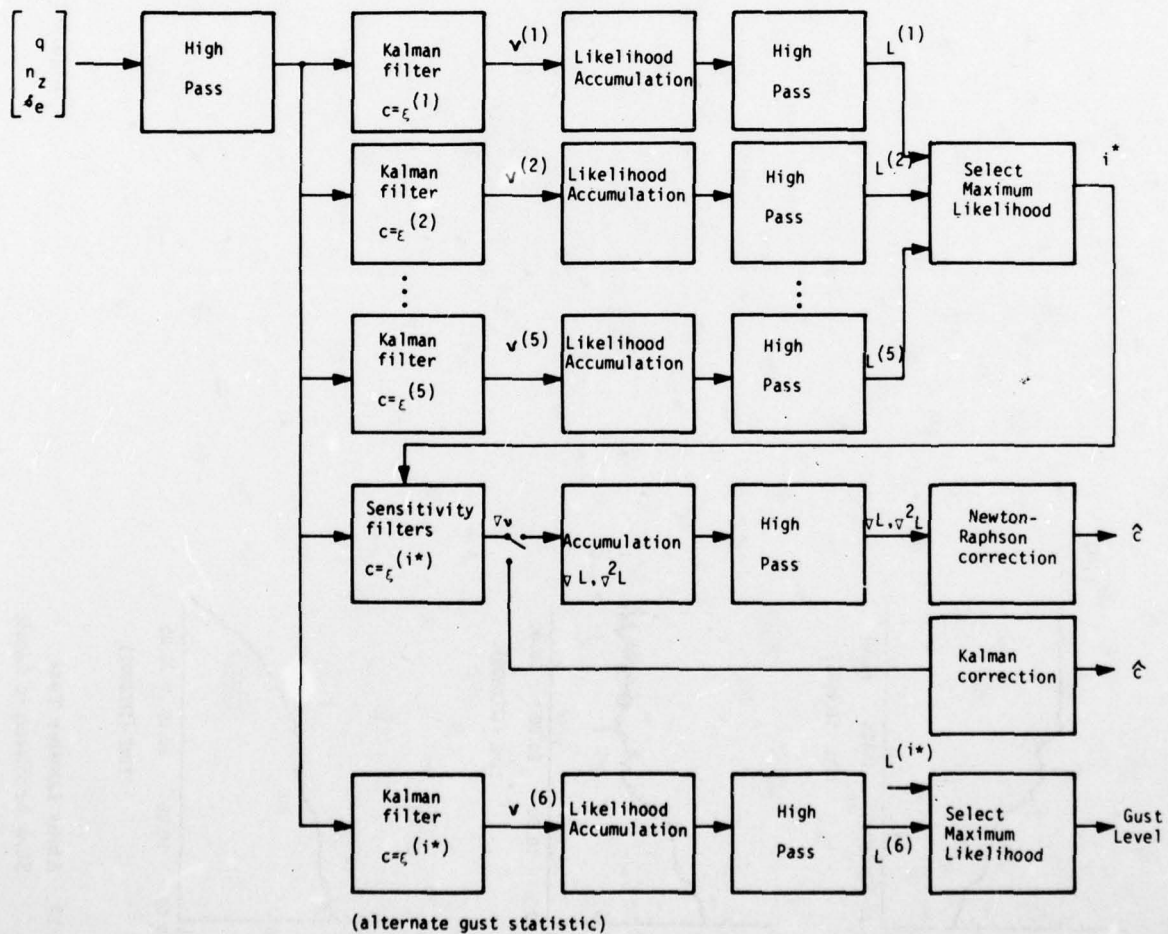
Figure 16. Identifier with Two-Level Gust Estimation and Automatic Gain Adjustment
