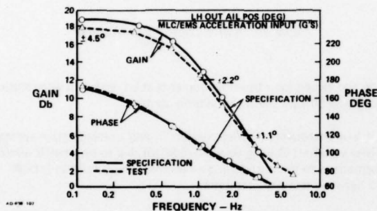
Figure 35. Aileron Control Laws
