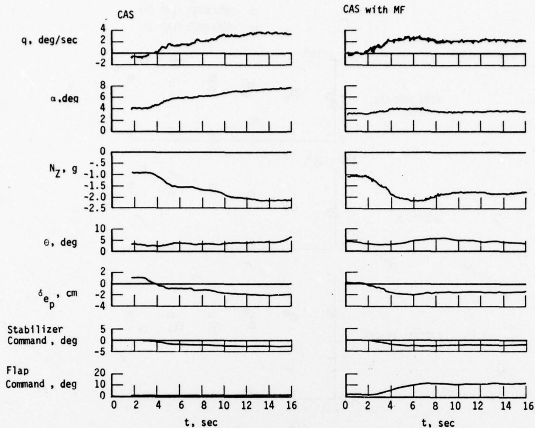
Figure 9. Wind-up Turn 350 KIAS at 6100 Meters
