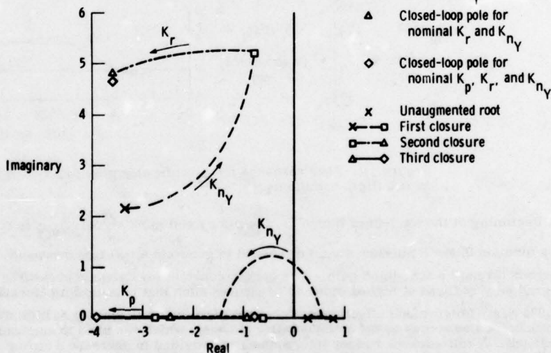
Figure 12. Effects of augmentation loop closures on the lateral-directional roots. Mach 1.0; h = 3050 meters.
