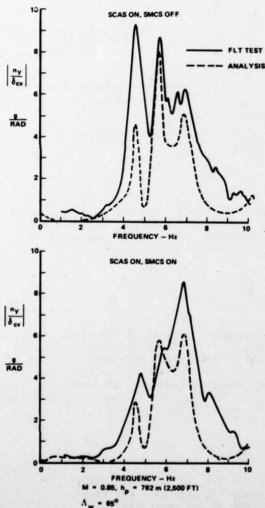
Figure 20. Comparison of Flight Test and Analytical Data, Frequency Response of Lateral Load Factor at FS 582 (229) Due to SMCS Vane Deflection
