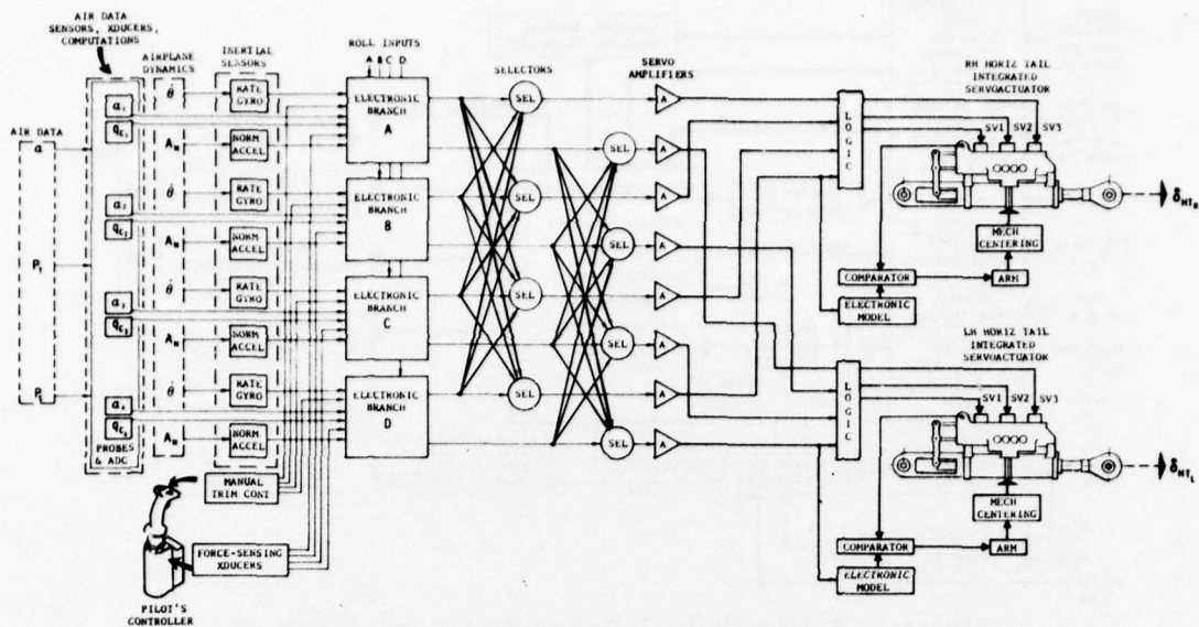
Figure 7 Pitch Functional Schematic Diagram
