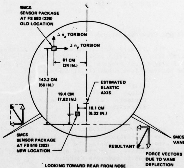
Figure 21. SMCS Sensor Package Locations and Coupling Characteristics
