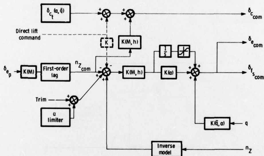
Figure 7. Longitudinal primary control law structure.
