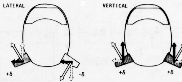
Figure 5. Vane Control Forces
