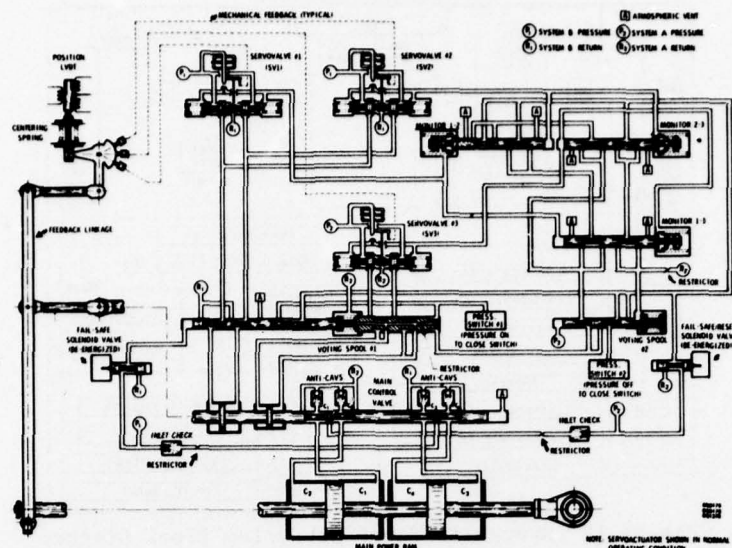
Figure 10 Integrated Servoactuator Schematic
