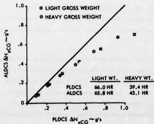
Figure 22 - Aerial Refueling Load Factor Comparison
