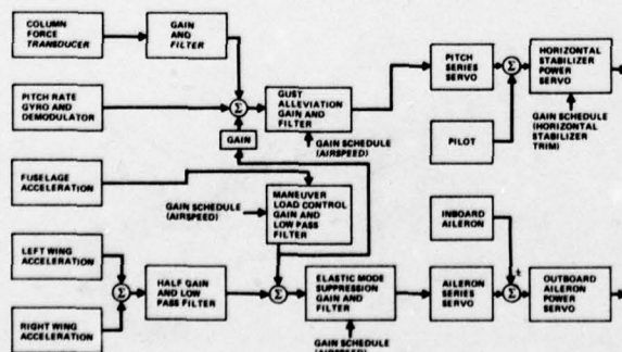
Figure 27. L-1011 MLC/EMS/GA System Block Diagram
