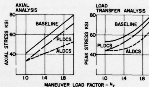
Figure 26 - Analytical Maneuver Stresses - Spanwise Splice
