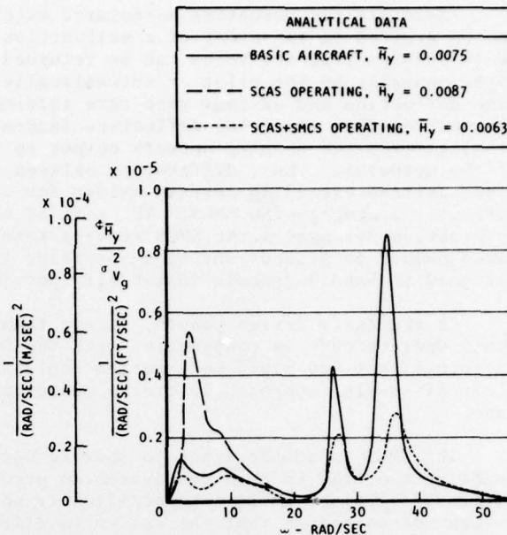
Figure 9. Power Spectral Density Associated With Lateral Crew Sensitivity Index, \bar{H}_y , M = 0.85 , h_p = 762 m (2,500 Ft), \Lambda_w = 65^\circ , Medium Weight
