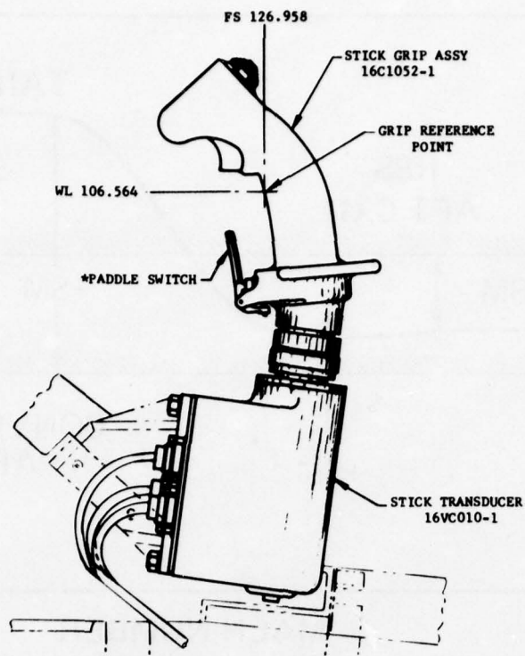
Figure 18 Pilot's Side-Stick Controller
