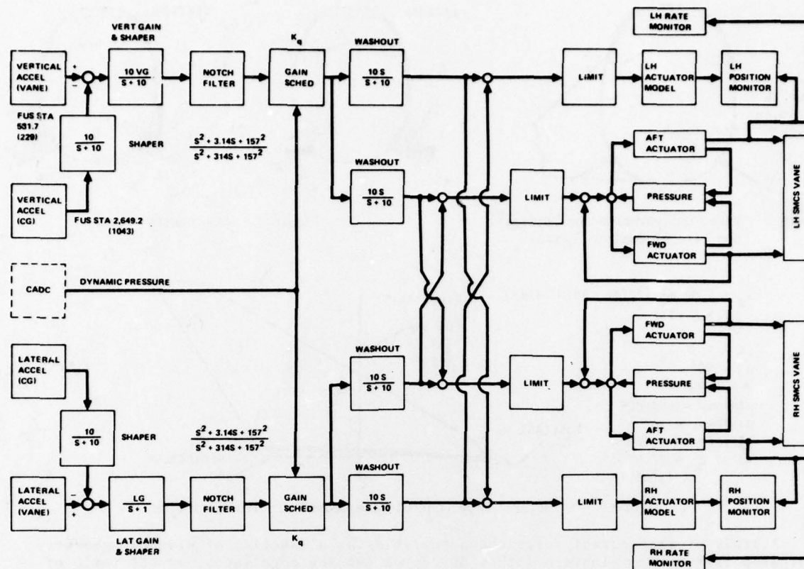
Figure 7. Structural Mode Control System Block Diagram
