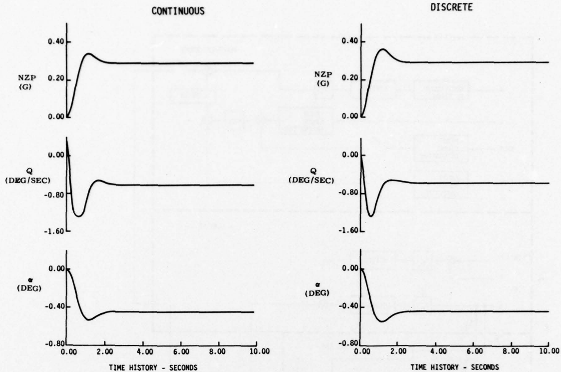
Figure 4. Comparison of Continuous and Discrete ( T=0.03125 ) Command Response
