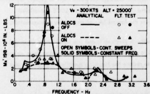
Figure 11 - Wing Root Bending Response
