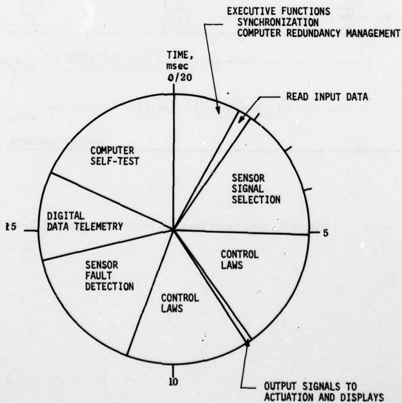
Figure 5. F-8 DFBW Software Timing Chart
