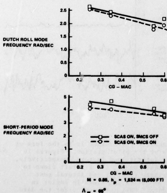
Figure 18. SMCS Impact on Short-Period and Dutch Roll Frequencies
