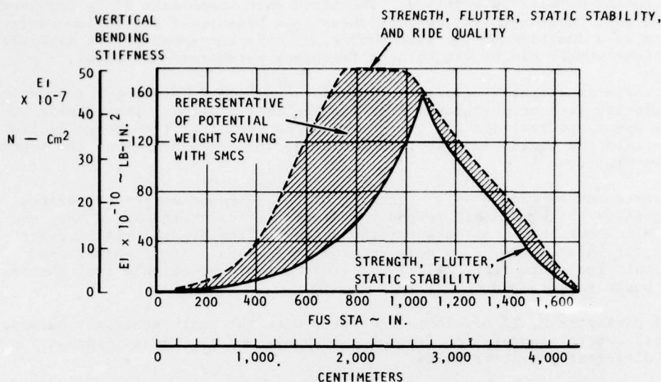
Figure 3. Fuselage Vertical Bending Stiffness Requirements for Vertical Ride Quality
