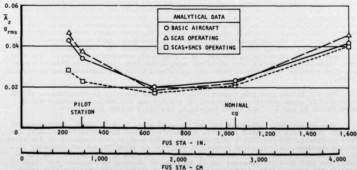
Figure 10. Effect of SMCS on Normal Load Factor Response Along Fuselage Due to Turbulence, M = 0.85 , h_p = 762 (2,500 Ft), \Lambda_w = 65^\circ , Medium Weight
