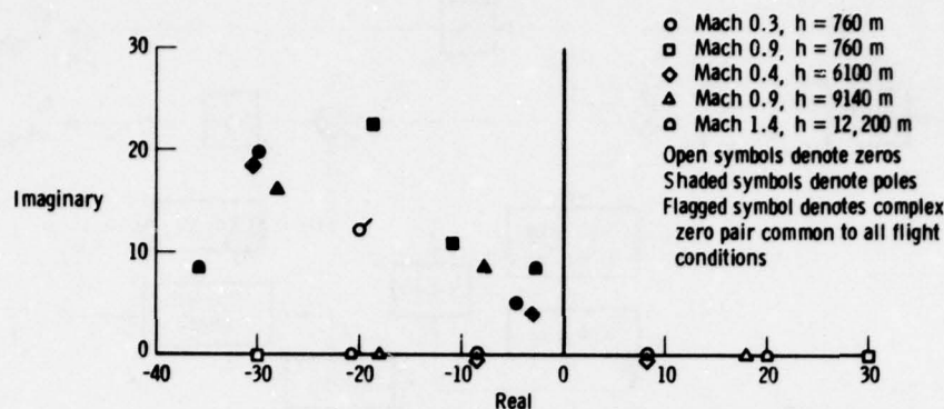
Figure 9. Closed-loop roots in longitudinal axis at selected flight conditions. Closed-loop pole-zero pairs near the origin are similar for all flight conditions.
