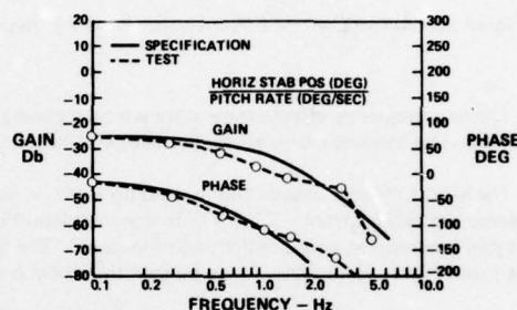
Figure 36. Stabilizer Control Laws
