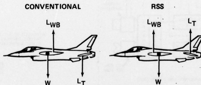
Figure 14 Subsonic Balance Comparison
