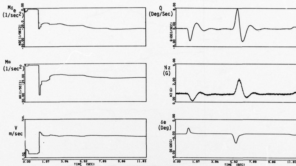
Figure 20. PCMLE Performance at Test Point 4
