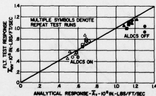
Figure 15 - Normalized Gust Response - W.S. 198 Bending
