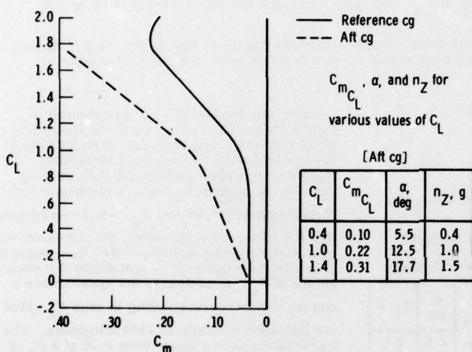
(c) Mach 0.2.
