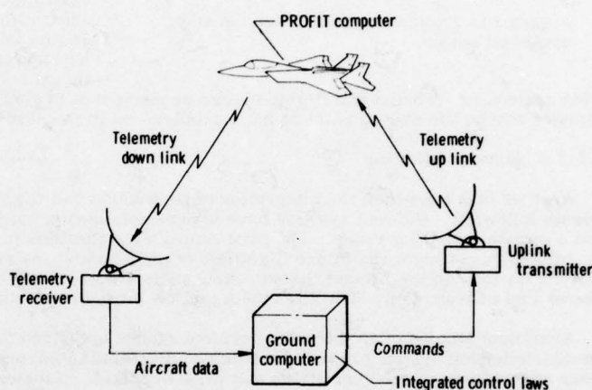
Figure 9. Schematic view of PROFIT remote computation.
