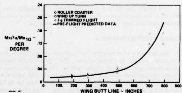
Figure 42. Comparison of Measured to Predicted Relative Wing Bending Moments
