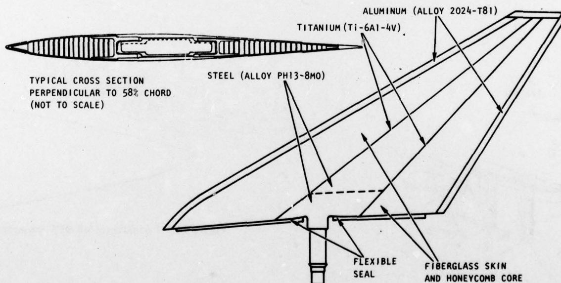
Figure 12. SMCS Vane Construction Details
