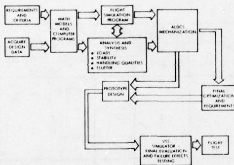
Figure 7 - ALDCS Development Tasks
