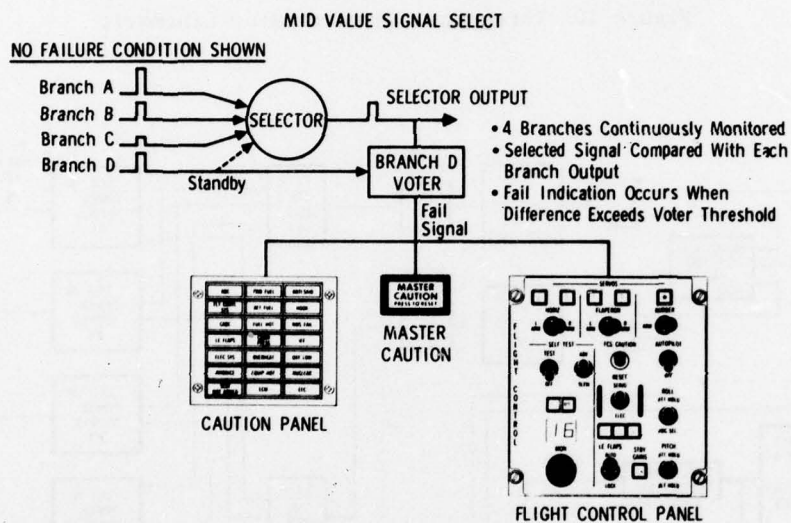
Figure 13 Electronic Signal Selection and Failure Monitoring
