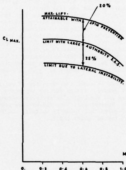
FIG 12 MANOEUVRE LIMITS EFFECT OF "FLY-BY-WIRE"
