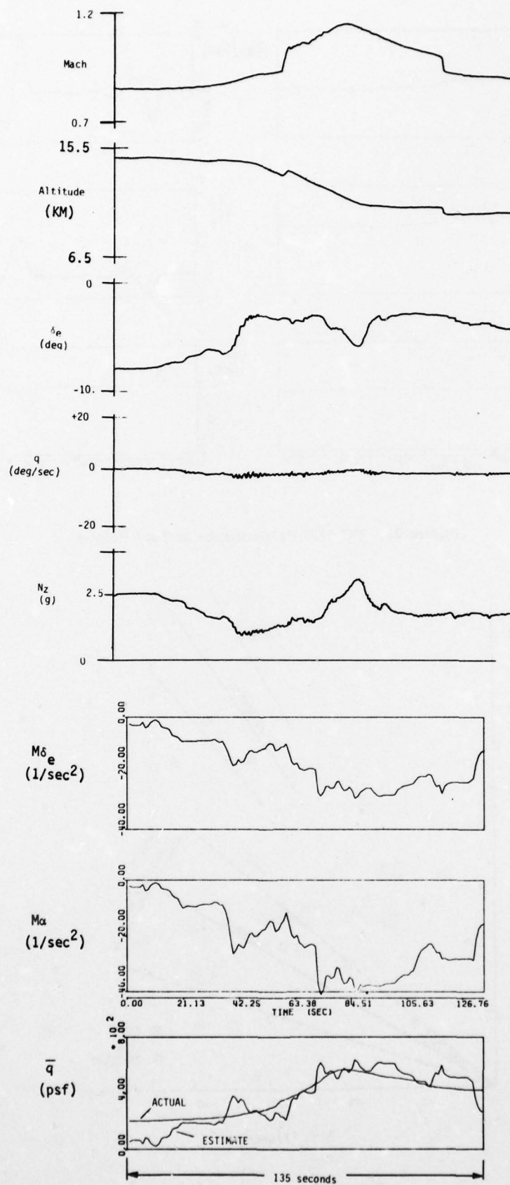
Figure 22. PCMLE Performance in Maneuvering Flight
