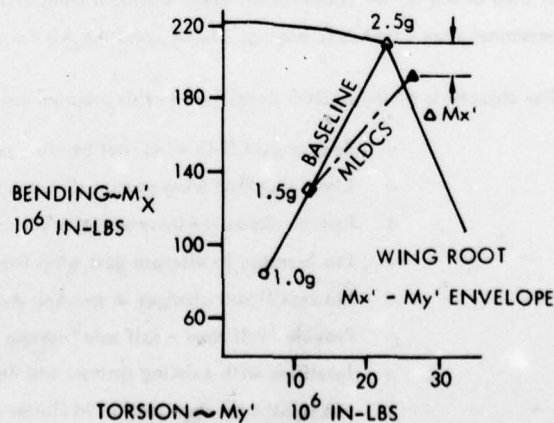
Figure 4 - MLDCS Loads Improvement
