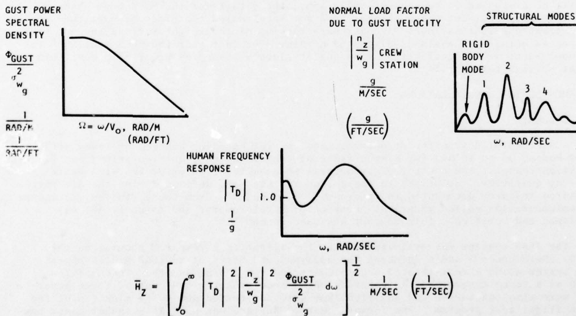
Figure 2. Crew Sensitivity Index for Ride Quality
