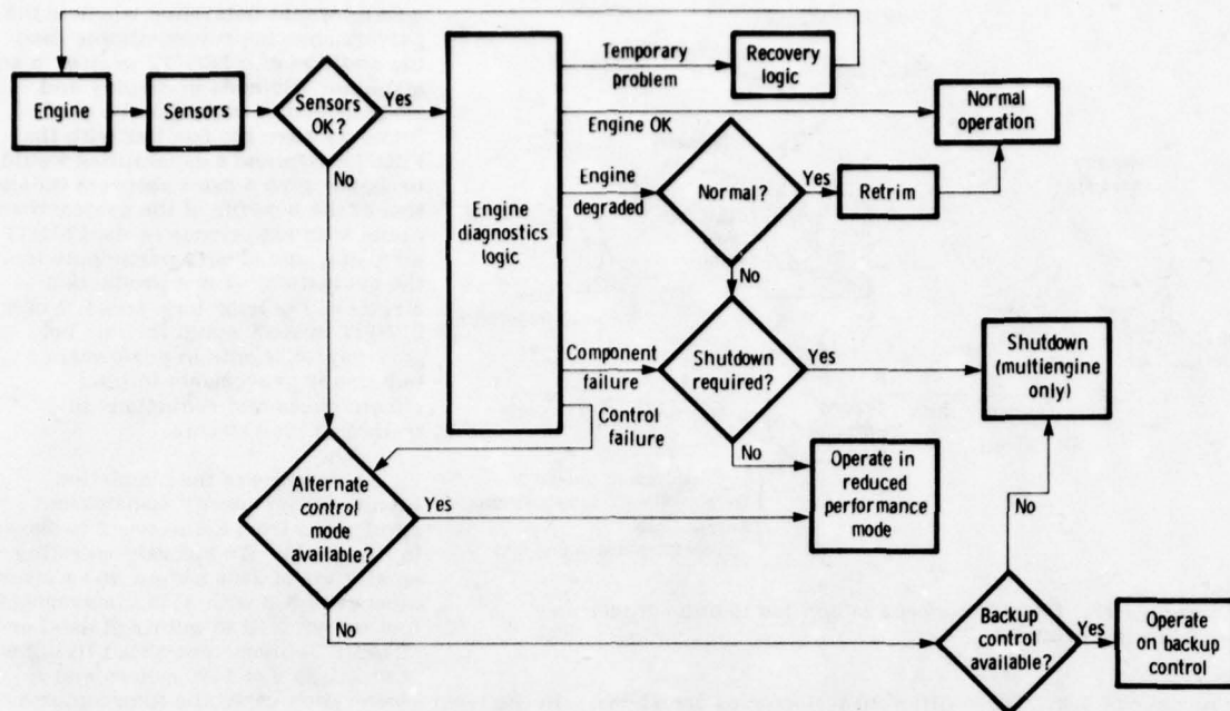
Figure 14. Engine diagnostic and action flow chart.
