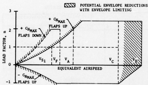
FIGURE 5. DESIGN MANEUVERING ENVELOPE
