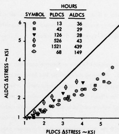
Figure 21 - Gust Axial Stress Comparison
