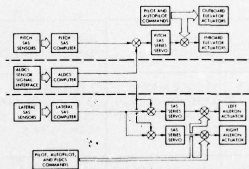
Figure 8 - ALDCS Systems Interfaces
