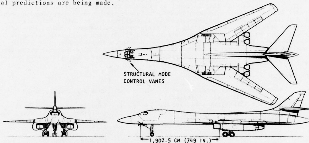
Figure 1. B-1 Aircraft with Wings Swept Aft
