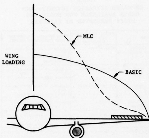
4a. UNLOADING OUTER WING
