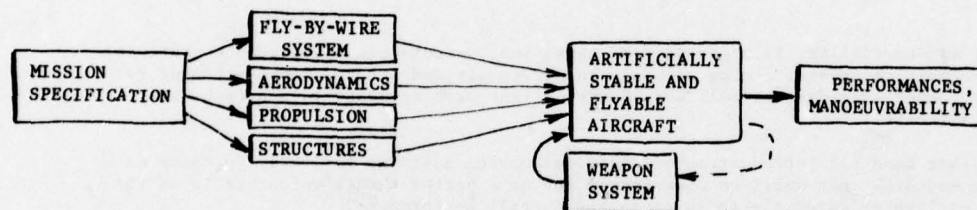
CCV Aircraft
