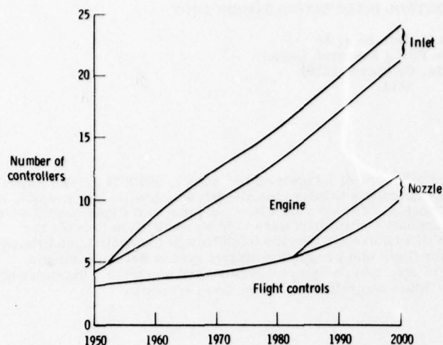
Figure 2. Number of controllers for propulsion and flight control systems of high performance aircraft.
