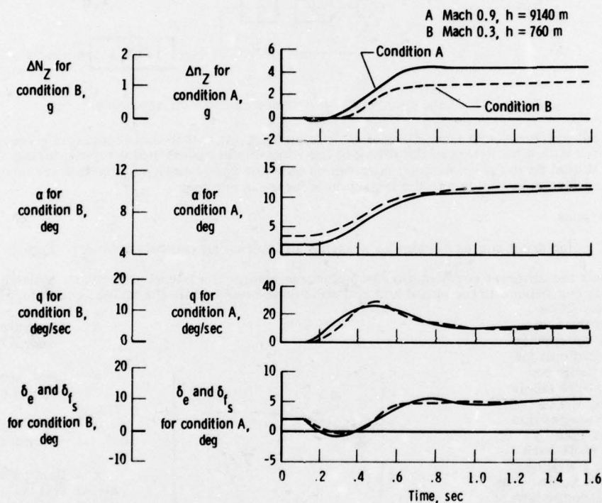
Figure 10. Time response for 3-centimeter pilot pitch stick step command at two flight conditions.
