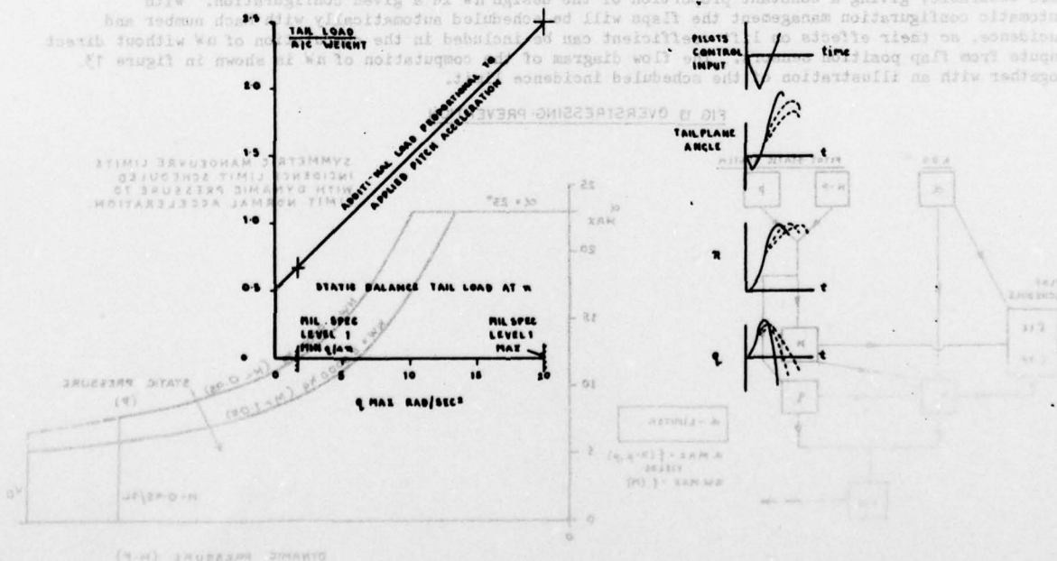
FIG.14 EFFECT OF ANGULAR ACCELERATION IN PITCH APPLIED AT PEAK NORMAL ACCELERATION ON DESIGN POSITIVE TAIL LOAD.
