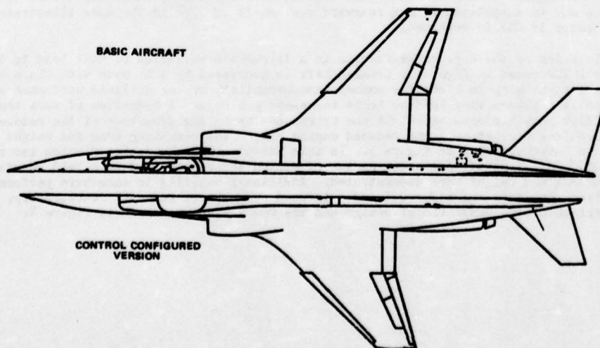
FIG 4 EFFECT OF ARTIFICIAL STABILITY ON AIRCRAFT SIZE
