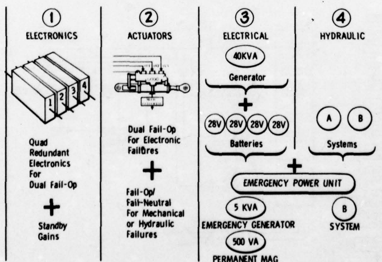
Figure 6 Flight Control System Redundancy Concept
