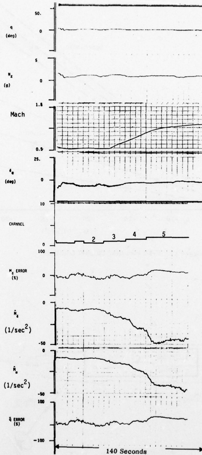
Figure 19. PCMLE Estimation with Newton-Raphson Parameter Correction
