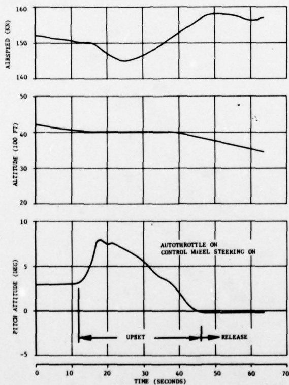
FIGURE 8c. APPROACH LONGITUDINAL STABILITY
