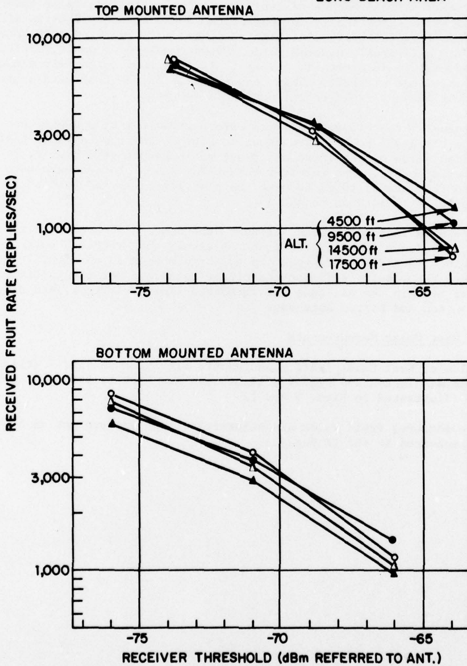
Fig. 6 Effects of altitude on fruit receptions.
