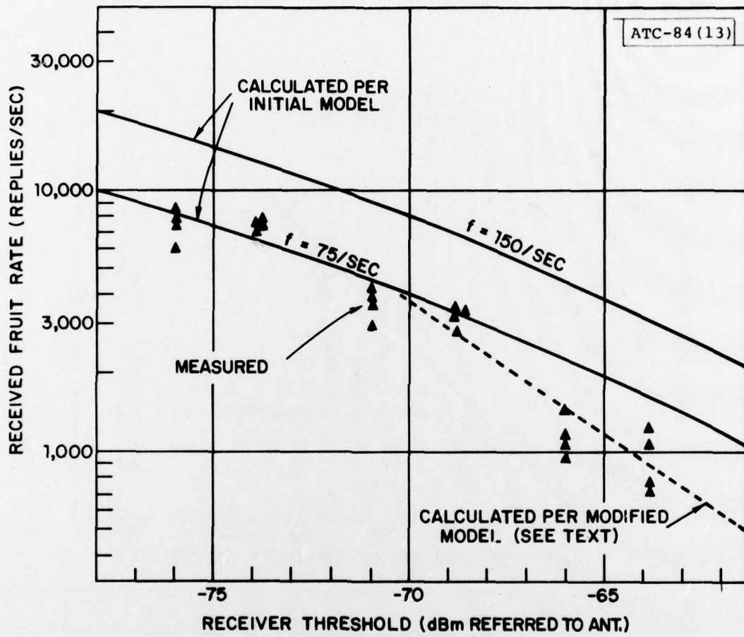
Fig. 13 Comparison between model and measurements.
