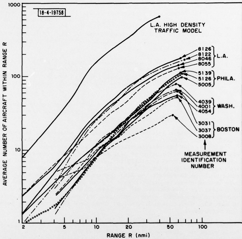
Fig.12. ATCRBS traffic distributions in range.
