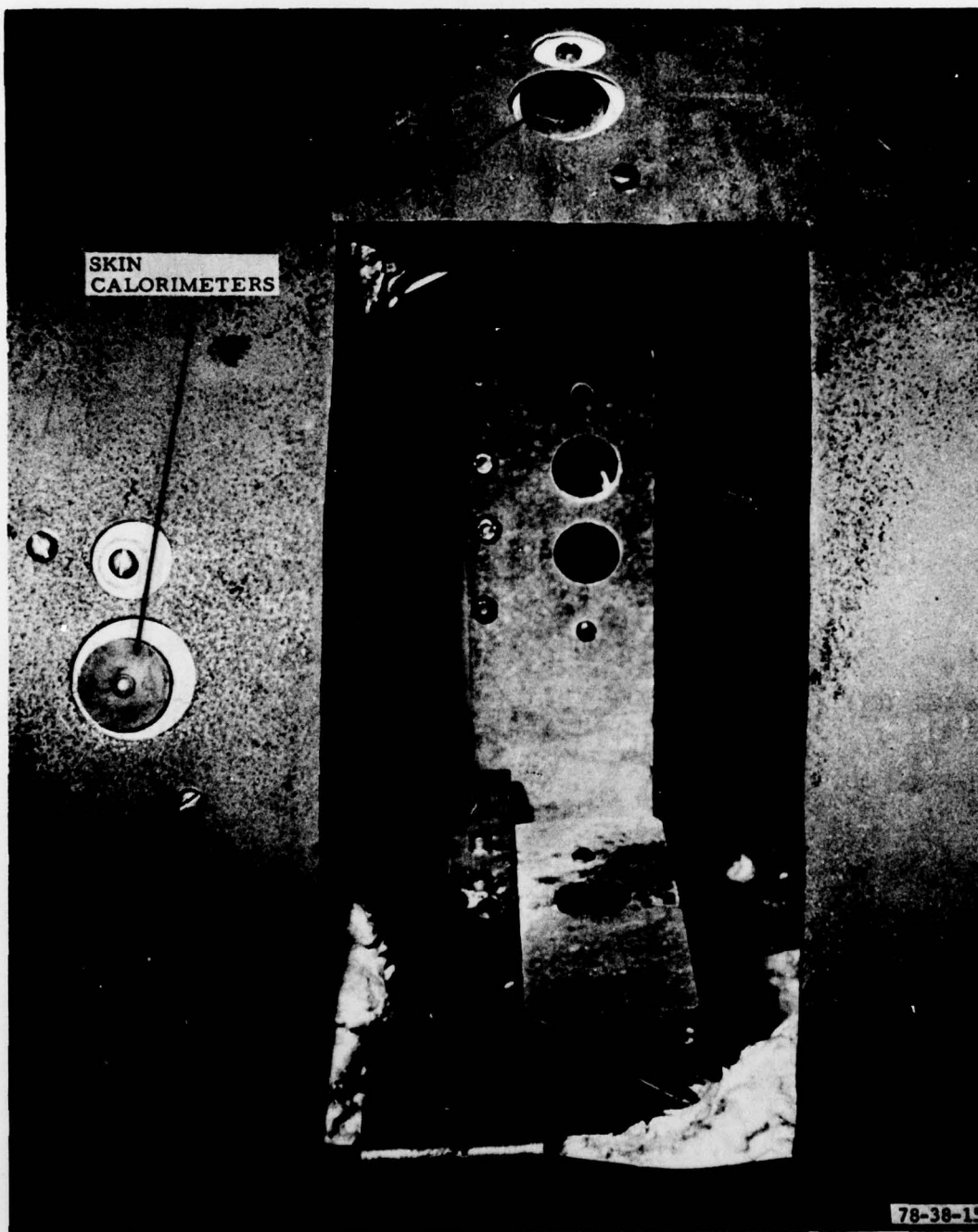
FIGURE 16. CALORIMETERS IMBEDDED IN SKIN OF 2-FOOT DUCT
