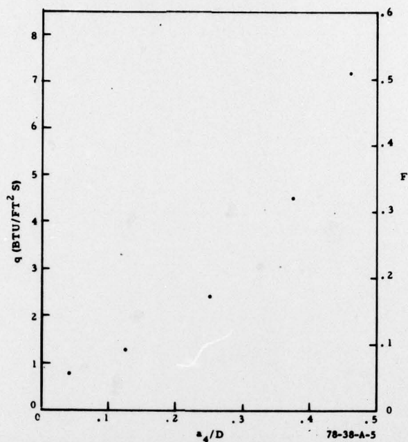
FIGURE A-5. VARIATION OF FLOOR HEAT FLUX BETWEEN DOOR EDGE AND DUCT MIDPLANE (D IS FUSELAGE DIAMETER)
