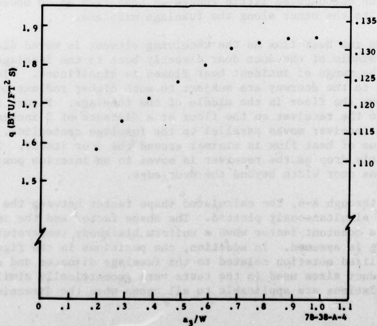
FIGURE A-4. VARIATION OF MIDPLANE RADIATION WITH HEIGHT
