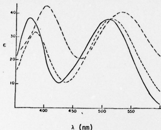
Figure 5. Absorption spectra for \text{Cr}(\text{NH}_3)_5\text{Cl}_2^+ and photolysis products. —, \text{Cr}(\text{NH}_3)_5\text{Cl}_2^+ ; ----, \text{cis-Cr}(\text{NH}_3)_4(\text{H}_2\text{O})\text{Cl}_2^+ ; - · - ·, (\text{H}_2\text{O})\text{Cl}_2^+ ; · · · ·, \text{cis-Cr}(\text{NH}_3)_4(\text{OH})\text{Cl}^+ .
