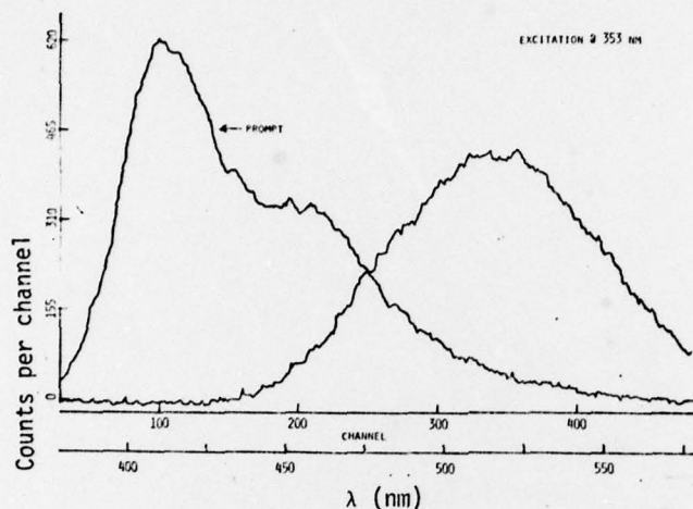
Figure 14. Time resolved emission spectra for 0.4 M aqueous K_2Pt(CN)_4 . The prompt spectrum (left) follows the 20 nsec exciting pulse; the right hand spectrum shows a 500 nsec decay (and is oxygen quenched).
