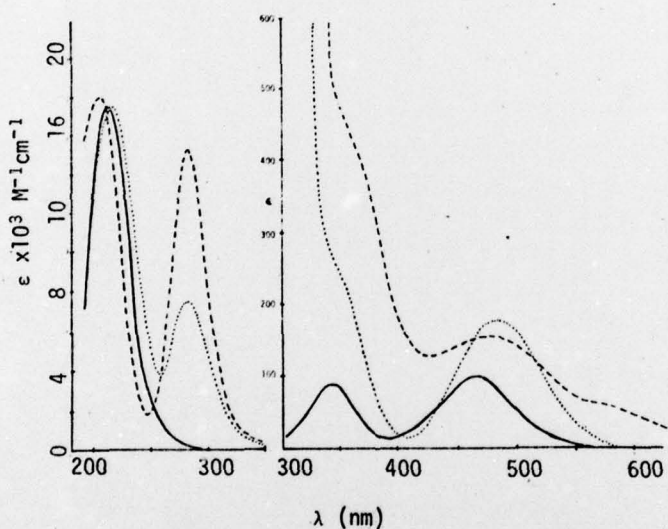
Figure 8. Adsorption spectra for \text{Co(en)}_2\text{L}^{n+} complexes. —, \text{Co(en)}_3^{3+} . ---, \text{Co(en)}_2(\text{SN})^{2+} . ····, \text{Co(en)}_2(\text{MeSN})^{3+} .
