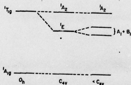
Figure 10. Splitting of the {}^1T_{1g} state in d^6 by reduction of symmetry.
