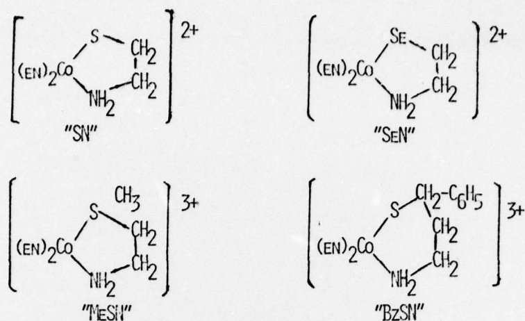
Figure 7. Structure and designations of ligands L in \text{Co(en)}_2\text{L}^{n+} .
