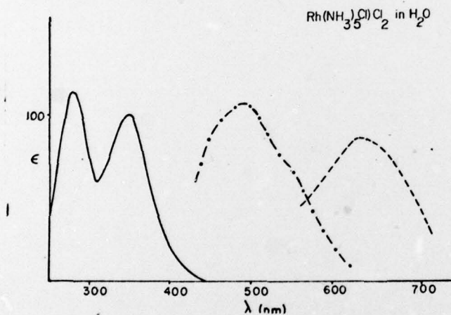
Figure 6. Aqueous \text{Rh}(\text{NH}_3)_5\text{Cl}_2^+ . — absorption spectrum. - · - · excited state absorption (minimum \epsilon_{\text{max}} , ca. 100 \text{ M}^{-1}\text{cm}^{-1} ). ---- emission spectrum (uncorrected for variation in vidicon sensitivity with wave length; correction will shift the maximum somewhat to longer wavelengths).
