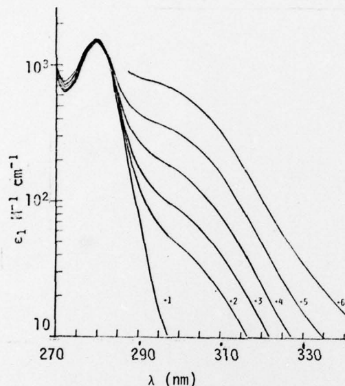
Figure 12. Apparent molar extinction coefficients for various concentrations of aqueous \text{K}_2\text{Pt}(\text{CN})_4 . Concentrations: 1, 8.96 \times 10^{-3} M; 2, 0.52 M; 3, 0.218 M; 4, 0.311 M; 5, 0.445 M; 6, 0.635 M.
