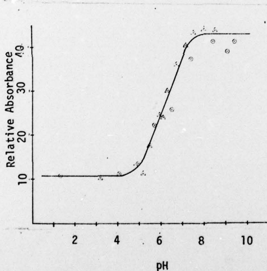
Figure 4. Absorbance increase (prompt plus delayed) on 530 nm pulse laser photolysis of aqueous \text{Cr}(\text{NH}_3)_5\text{Cl}^{2+} as monitored at 580 nm. Solid line shows the transition from \text{Cr}(\text{NH}_3)_4(\text{H}_2\text{O})\text{Cl}^{2+} to \text{Cr}(\text{NH}_3)_4(\text{OH})\text{Cl}^+ .
