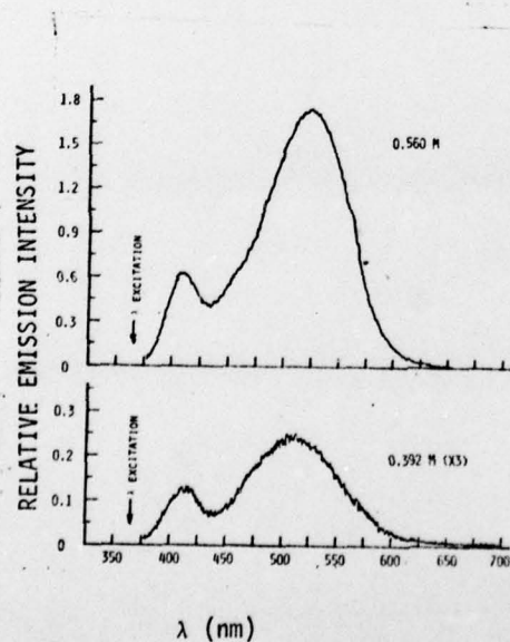
Figure 13. Spectrofluorimetric emission spectra for two concentrations of aqueous \text{K}_2\text{Pt}(\text{CN})_4 . Excitation at 366 nm.
