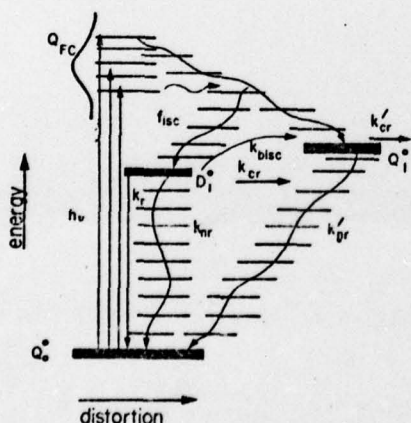
Figure 1. Excited state scheme for a d^3 system.
