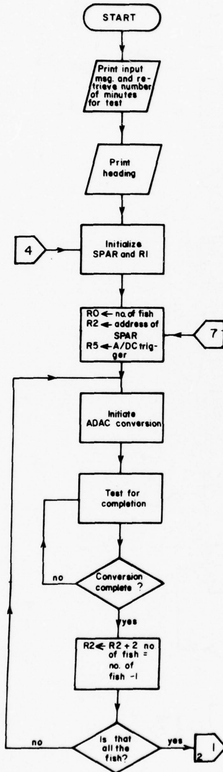
Figure 10. Flow Chart Depicting the Computer Program.
