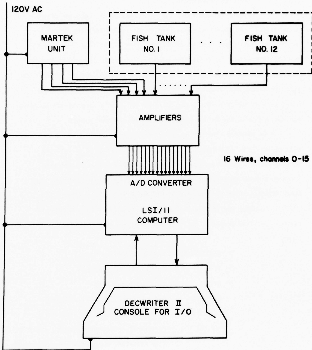
Figure 9. System Layout.
