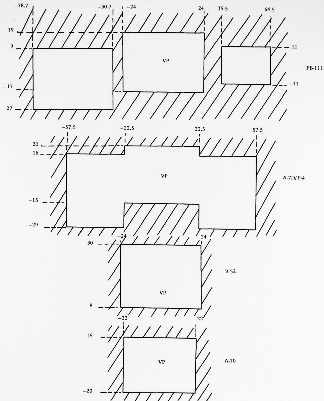
Figure 4. Aerial refueling FOVs.
