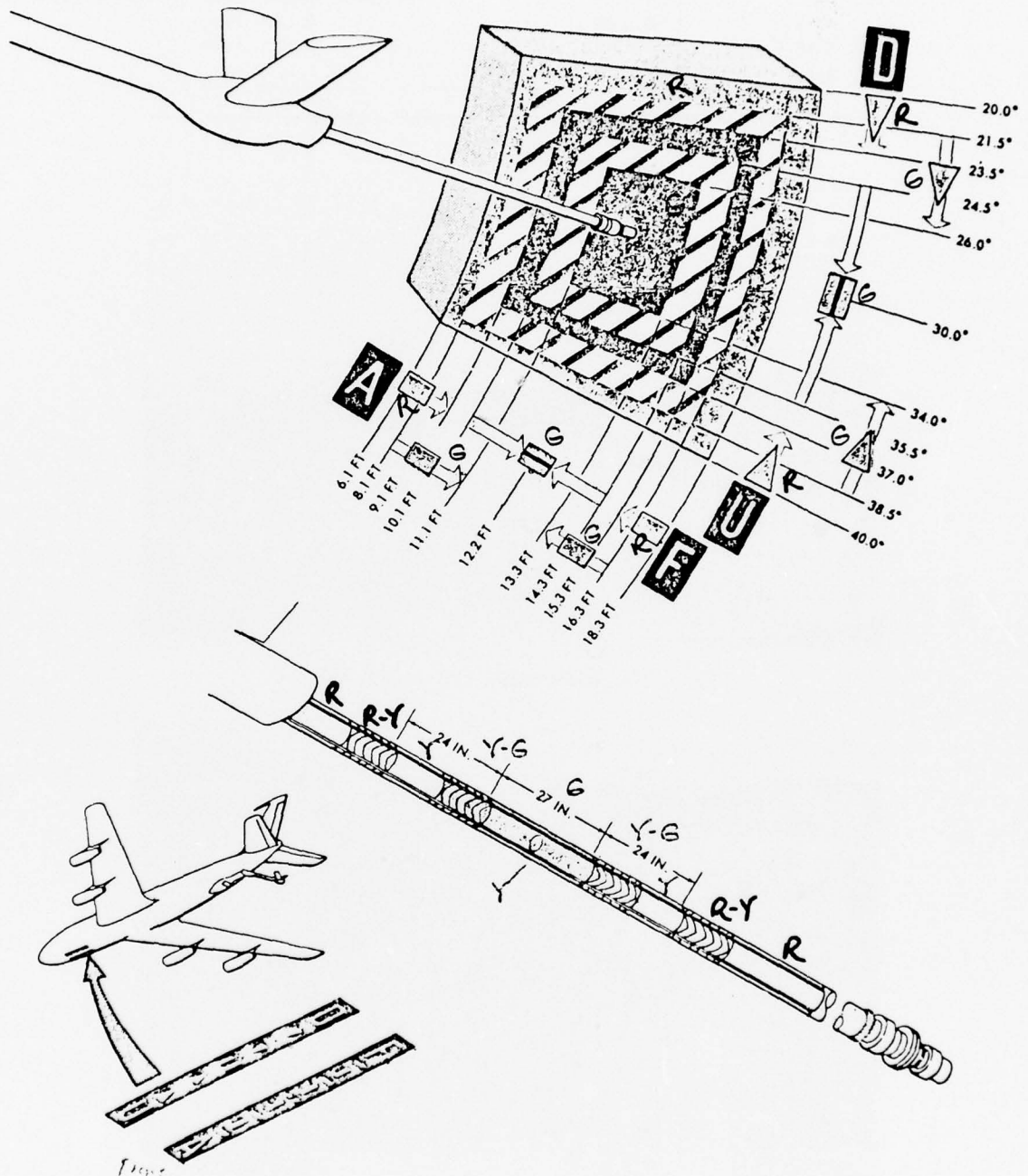
Figure 26. Receiver director lights illumination profile.
