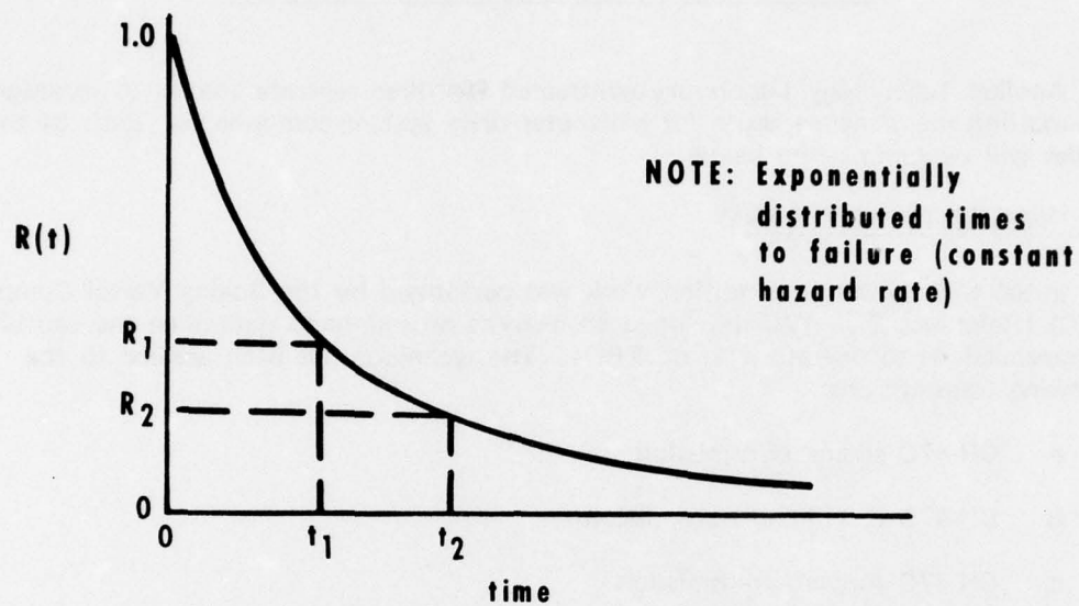
Figure 5. Reliability function for a constant hazard rate.
