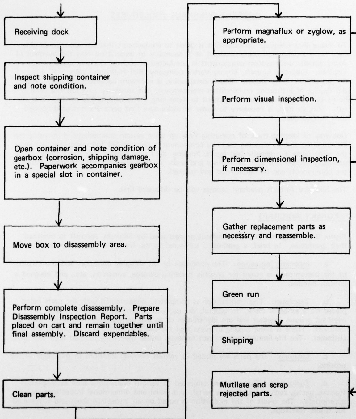
Figure 9. Sikorsky Aircraft transmission overhaul process.
