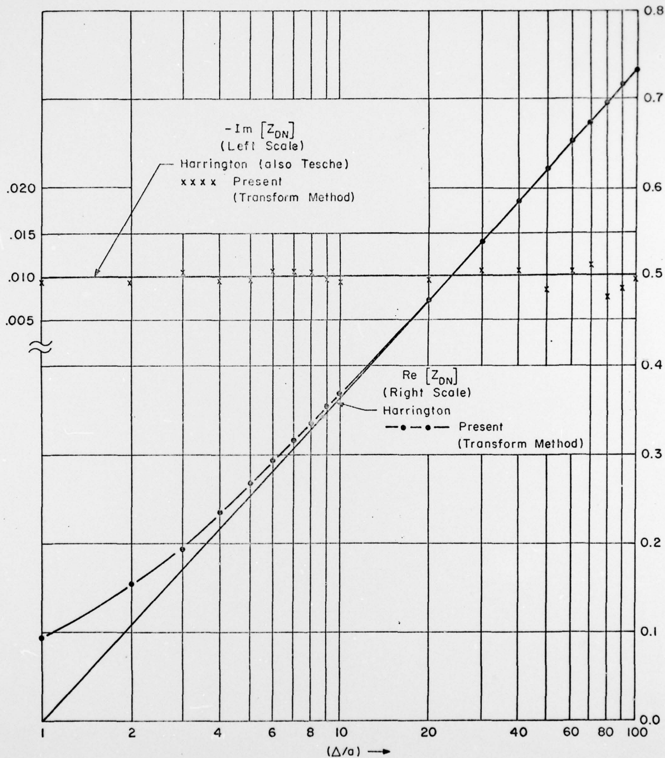
Figure 2. Plot of the Diagonal Term of the Normalized Hallén-System Matrix as a Function of Normalized Cell Width (\Delta/a) , K\Delta = 0.125664 (or 50 Cells Per Wavelength)
