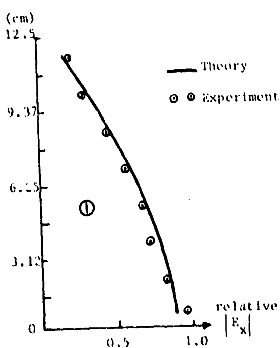
Fig. 3 Theoretical and experimental results on the x-components of the induced electrical fields in a conducting body of 12.5 \times 6.25 \times 3.12 cm placed at a distance of 4.5 cm from a \lambda_0/4 monopole.
