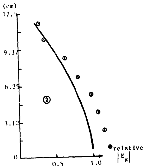
Fig. 3 Theoretical and experimental results on the x-components of the induced electrical fields in a conducting body of 12.5 \times 6.25 \times 3.12 cm placed at a distance of 4.5 cm from a \lambda_0/4 monopole.
