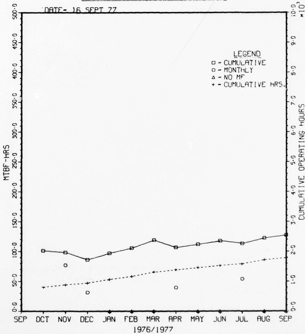
Figure 21 UHF ARC-171
