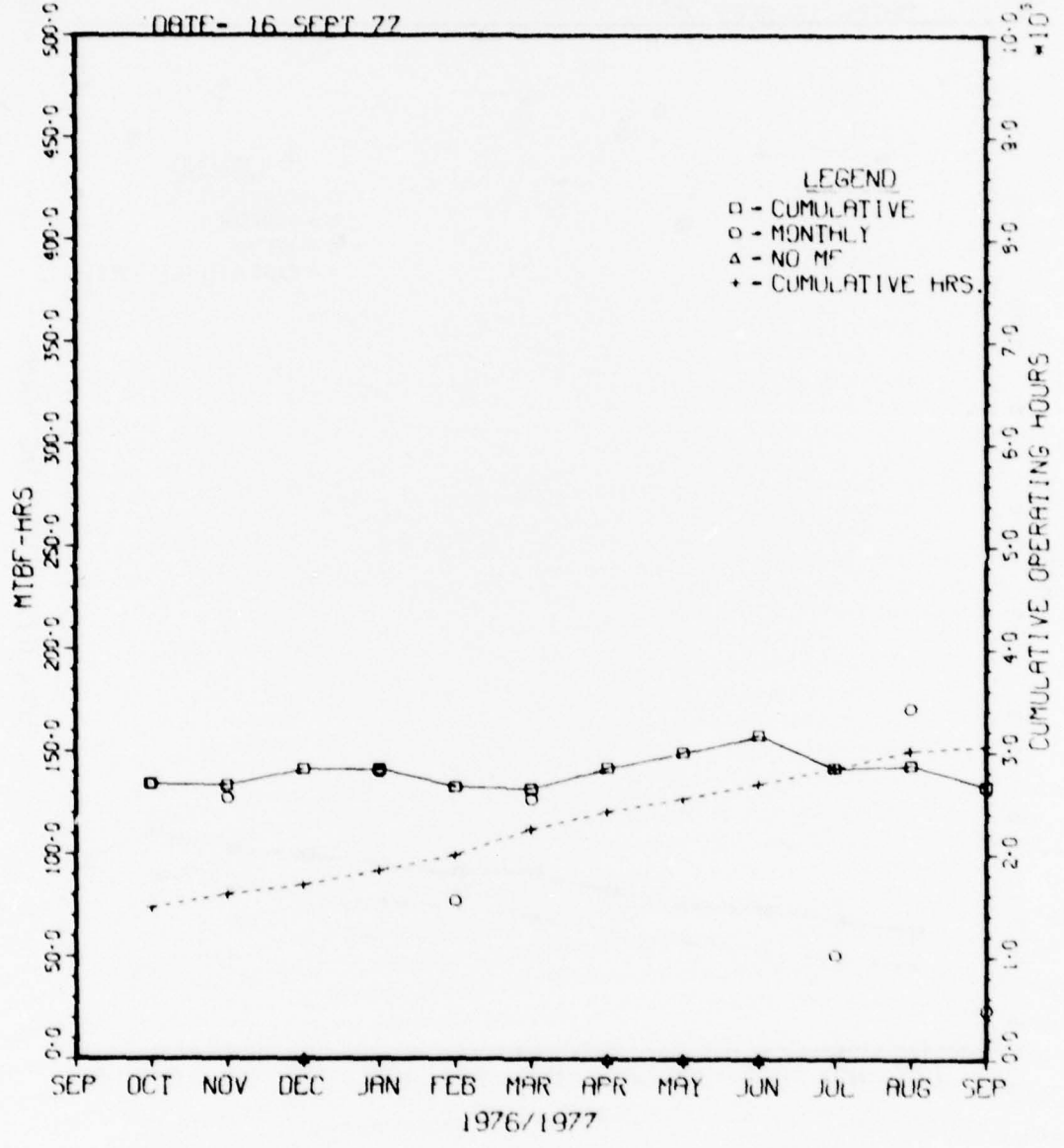
Figure 23 MODEM/Processor Group
