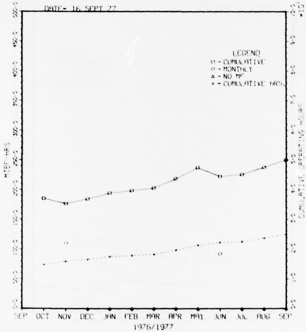
Figure 26 UHF ARC-151
