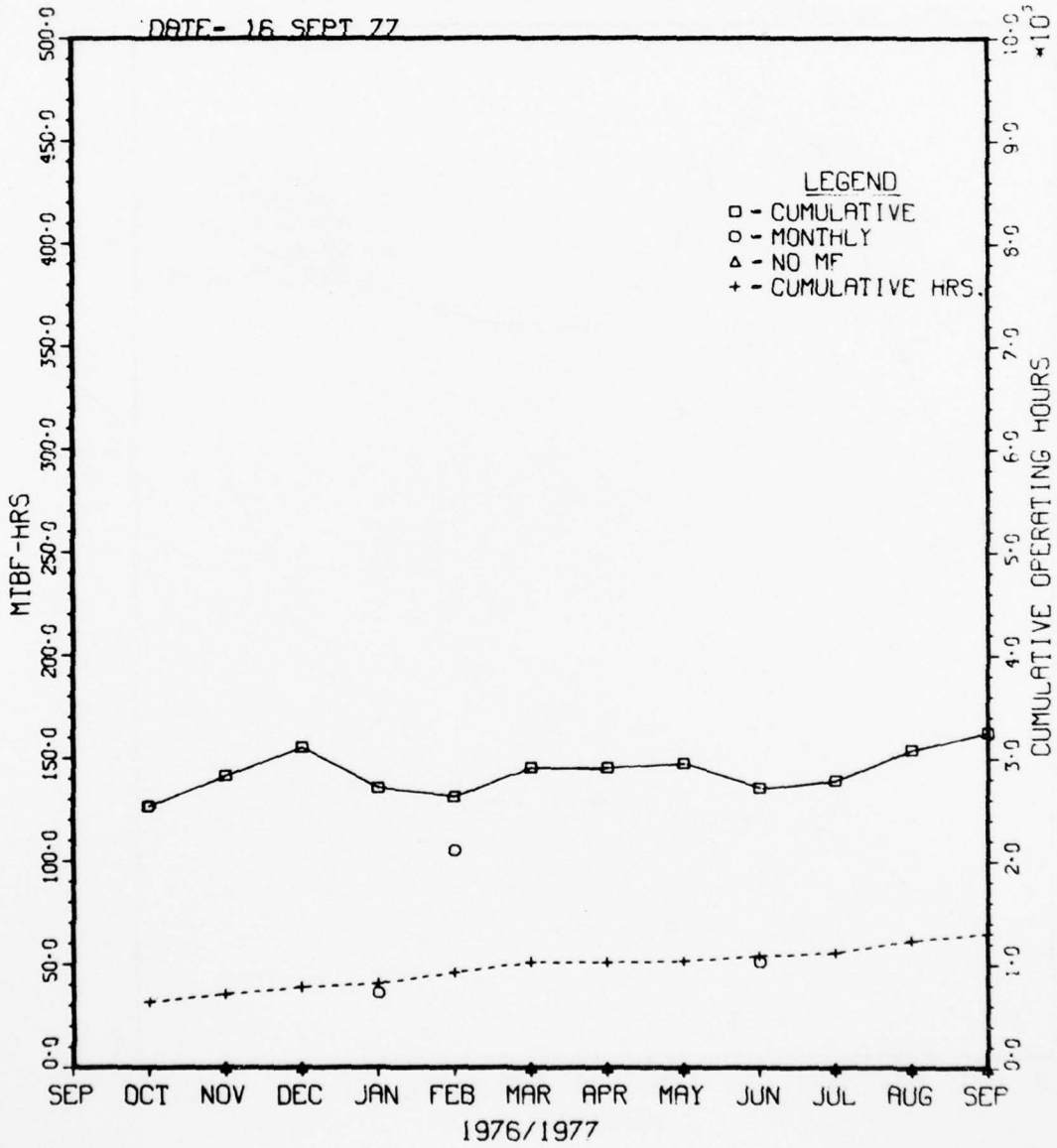
Figure 19 UHF ARC-151
