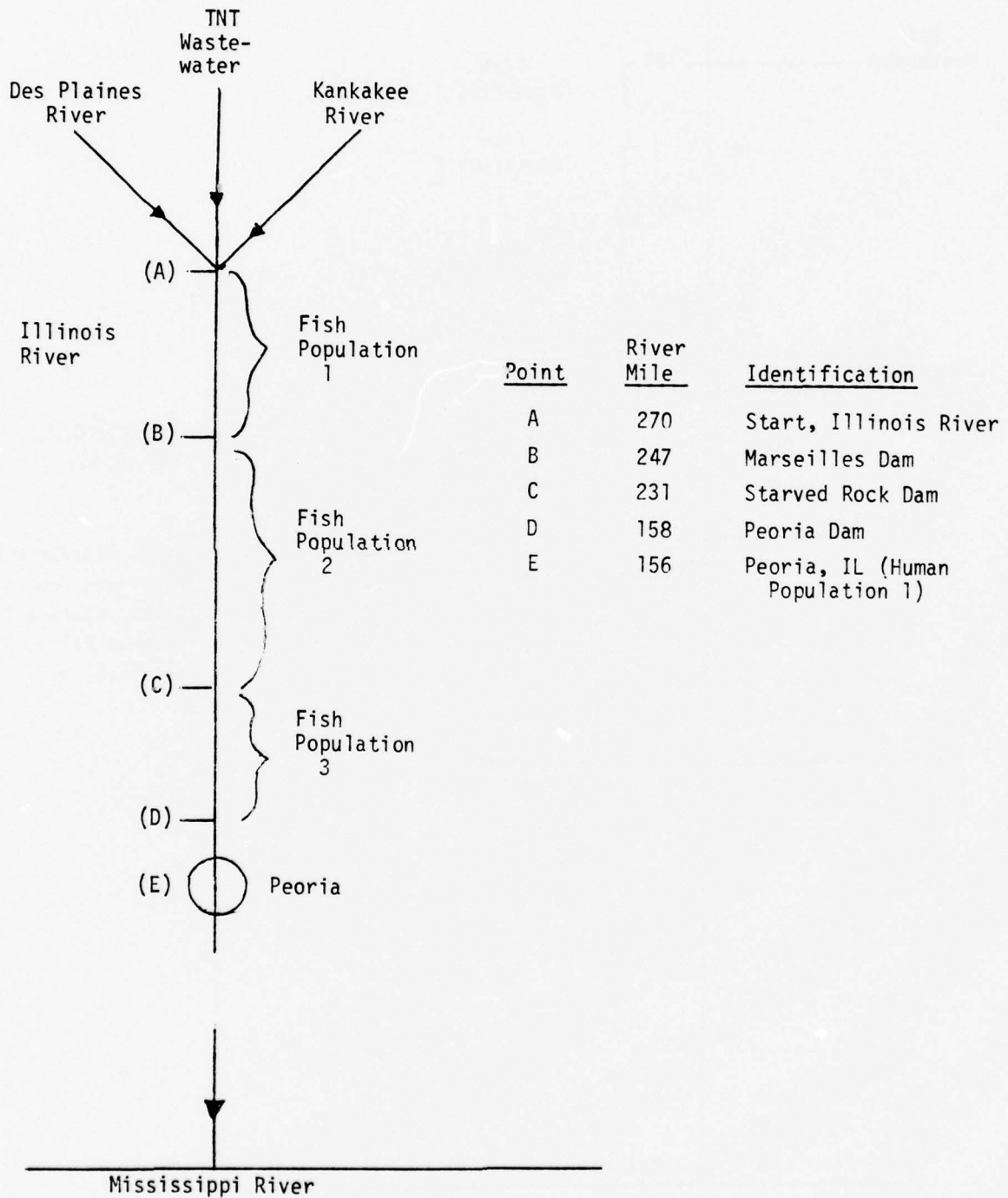
Figure 2. HRAM Representation of Populations at Risk from TNT Wastewaters of Joliet Army Ammunition Plant.
