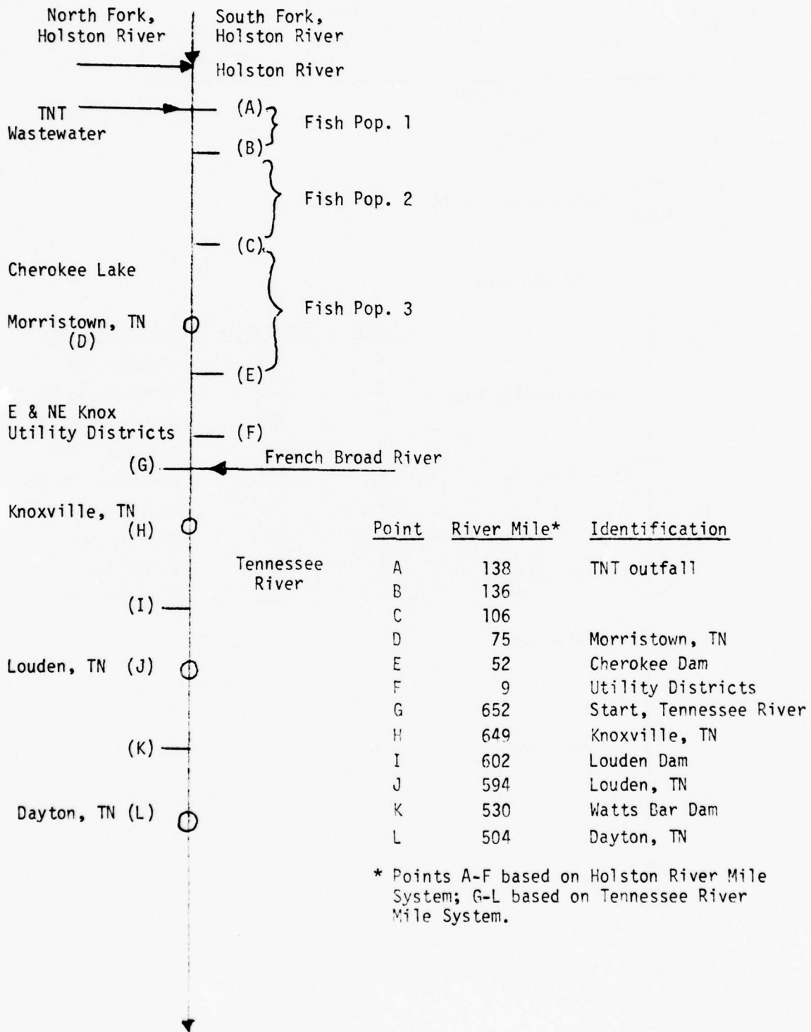
Figure 5. HRAM Representation of Populations at Risk from TNT Wastewaters of Holston Army Ammunition Plant.
