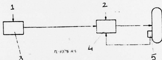
Fig. 5. Diagram of the antiskid system with a measurement of wheel angular deceleration 8 .
