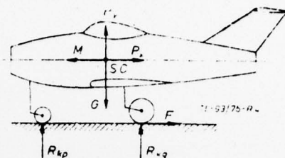
Fig. 4. Forces acting on an aircraft during braking at landing: ( P_y - aerodynamic force, P_x - aerodynamic drag, M - inertia, G - weight, F - adhesion force between tire and a surface, R_{kp} , R_{kg} - ground reactions, S.C. - center of gravity)
