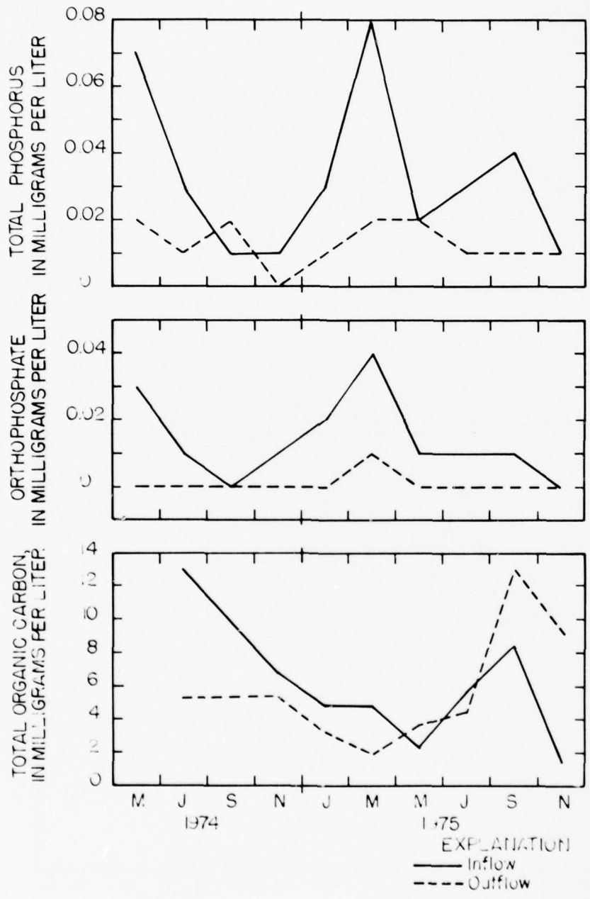
Figure 8.--Physical, chemical, and bacteriological data for the inflow and outflow--Continued
