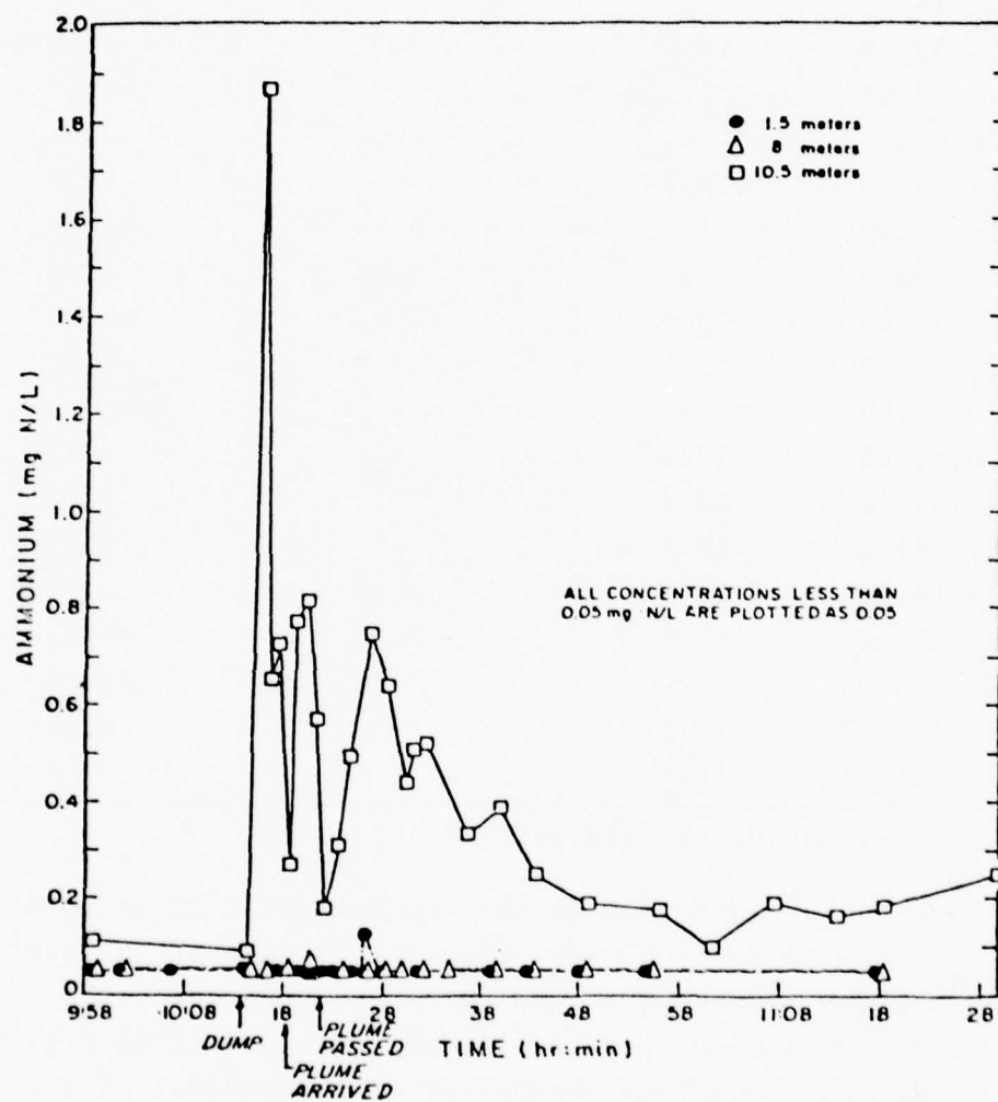
Figure 108 Ammonium Concentrations: Texas City Dump No. 2 near Buoy B 1 (October 10, 1975)
