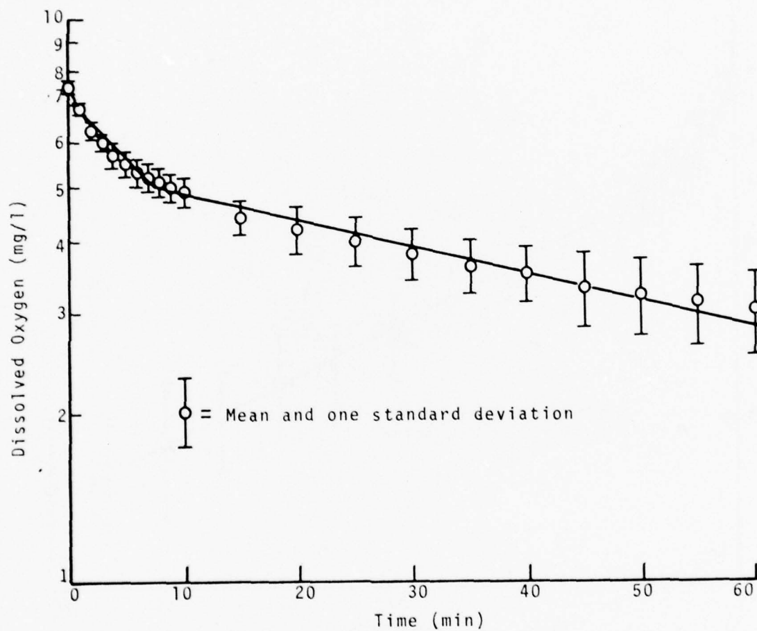
Figure 100 Oxygen Demand Test: Texas City Channel Site 5 Sediment (Sample size - 3 cc)
