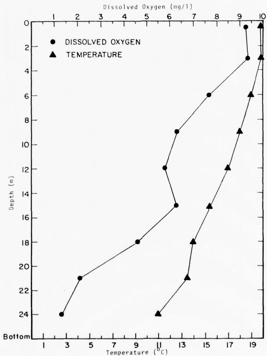
Figure 164 Post-Disposal Temperature and Dissolved Oxygen Water Column Profiles: New York Bight Dump No. 2 - Hatton
