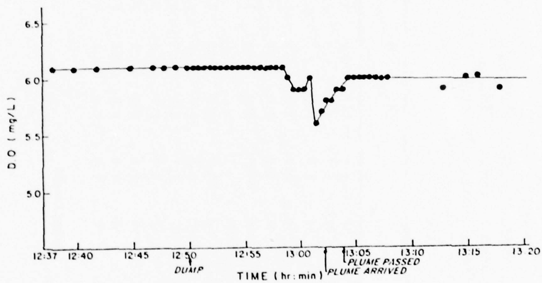
Figure 95 Dissolved Oxygen Concentrations: Galveston Dump No. 6 near Buoy D, Depth 15 m, Dredged Material from Galveston Bay Entrance Channel Buoys 3-7A, September 9, 1975
