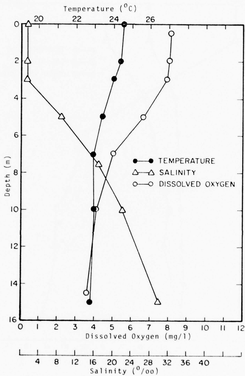
Figure 185 Temperature, Salinity, Dissolved Oxygen Profiles: Mobile Bay, Alabama near Buoys 21-22 June 3, 1976
