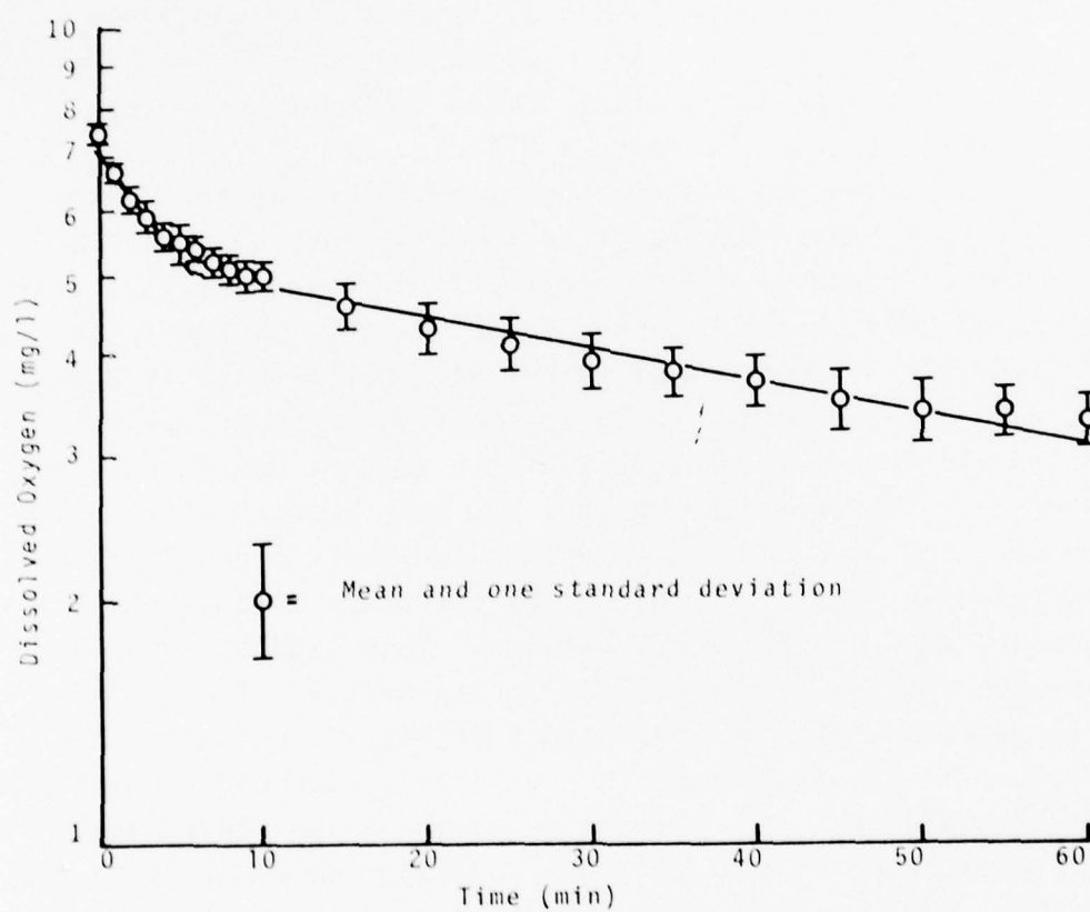
Figure 115 Oxygen Demand Test: Port Lavaca Sediment
