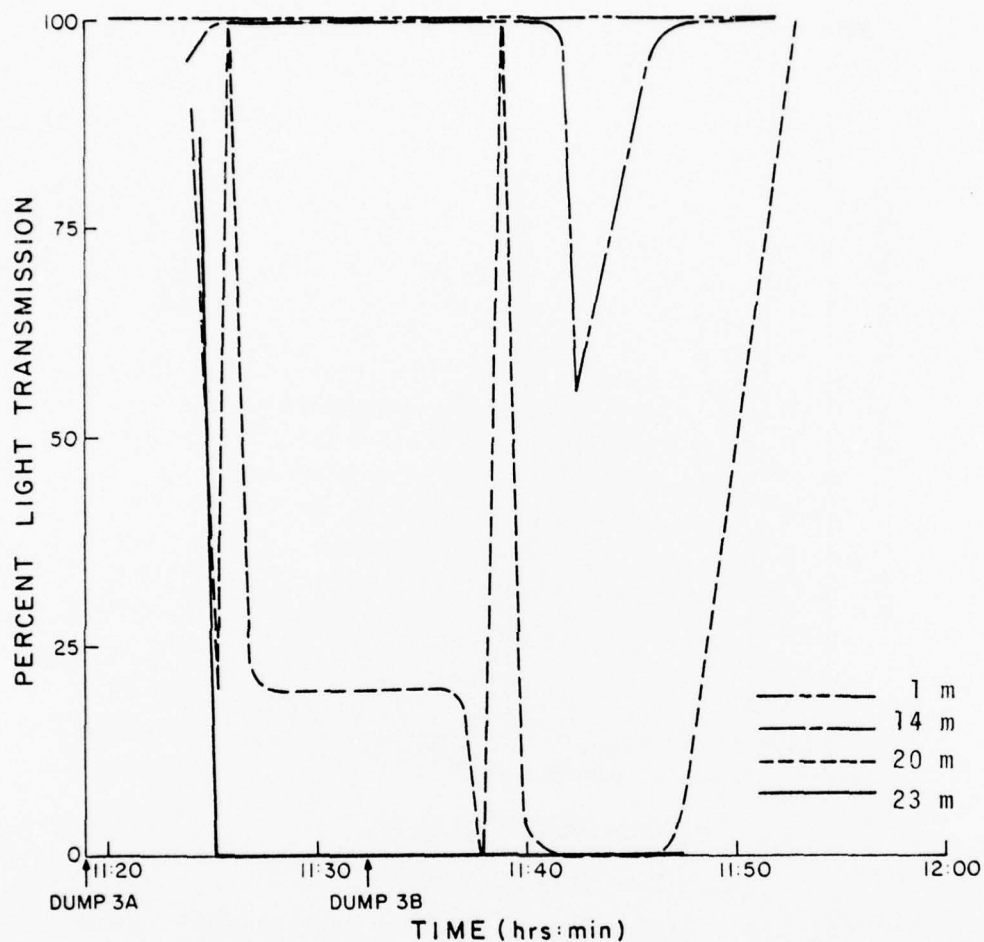
Figure 171 Percent Light Transmission as a Function of Depth and Time during New York Bight Dump No. 3 - Hatton (12 cm path length)
