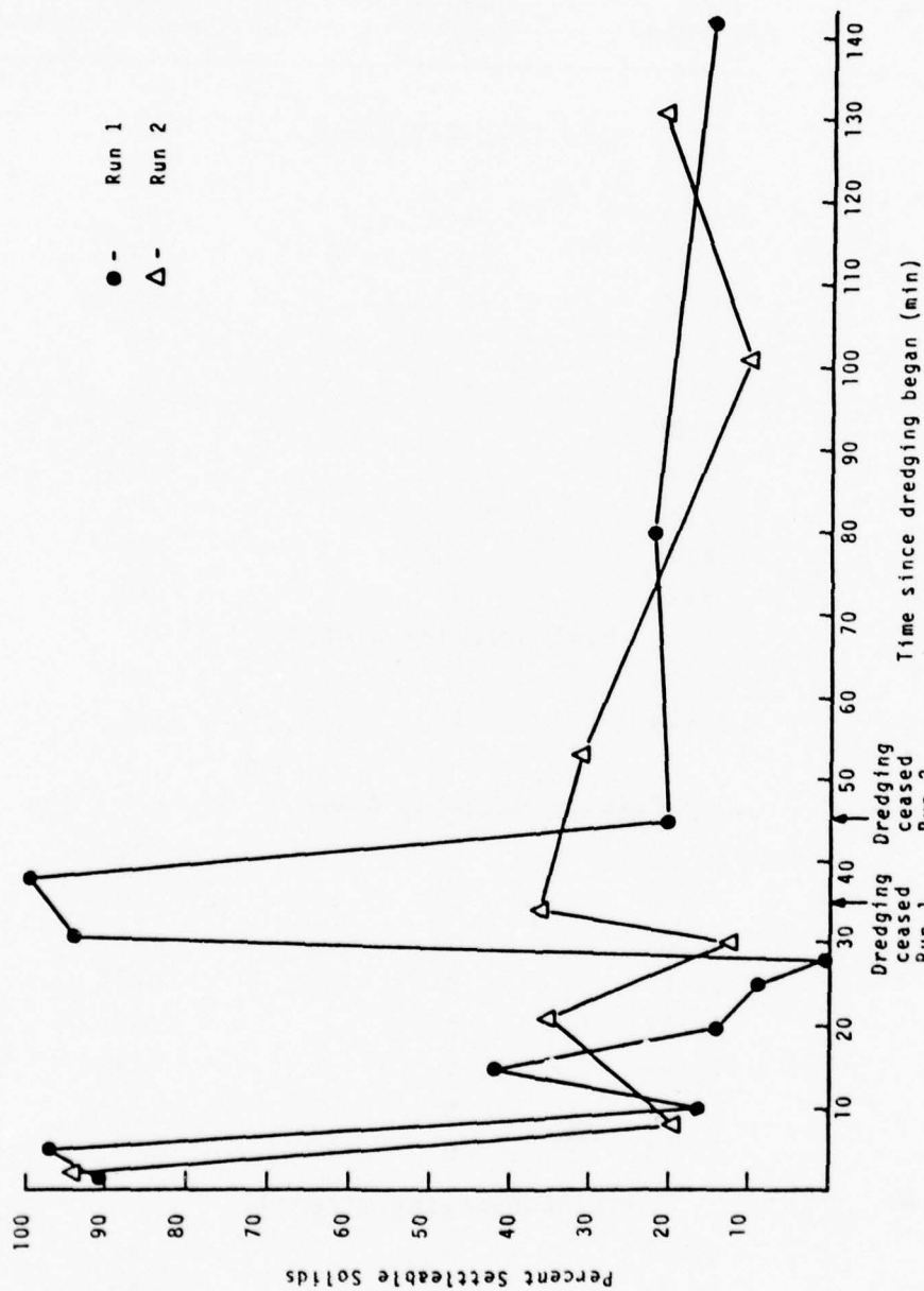
Figure 103 Changes in Percent Settleable Solids: Hopper Dredge Samples Dredged from Texas City Channel and Turning Basin (October 9, 1975)
