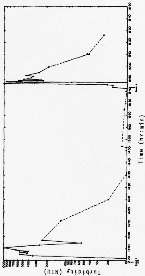
Figure 145 Turbidity in Near Bottom (24 m) Water during New York Dump Nos. 1 and 2 - Hutton
