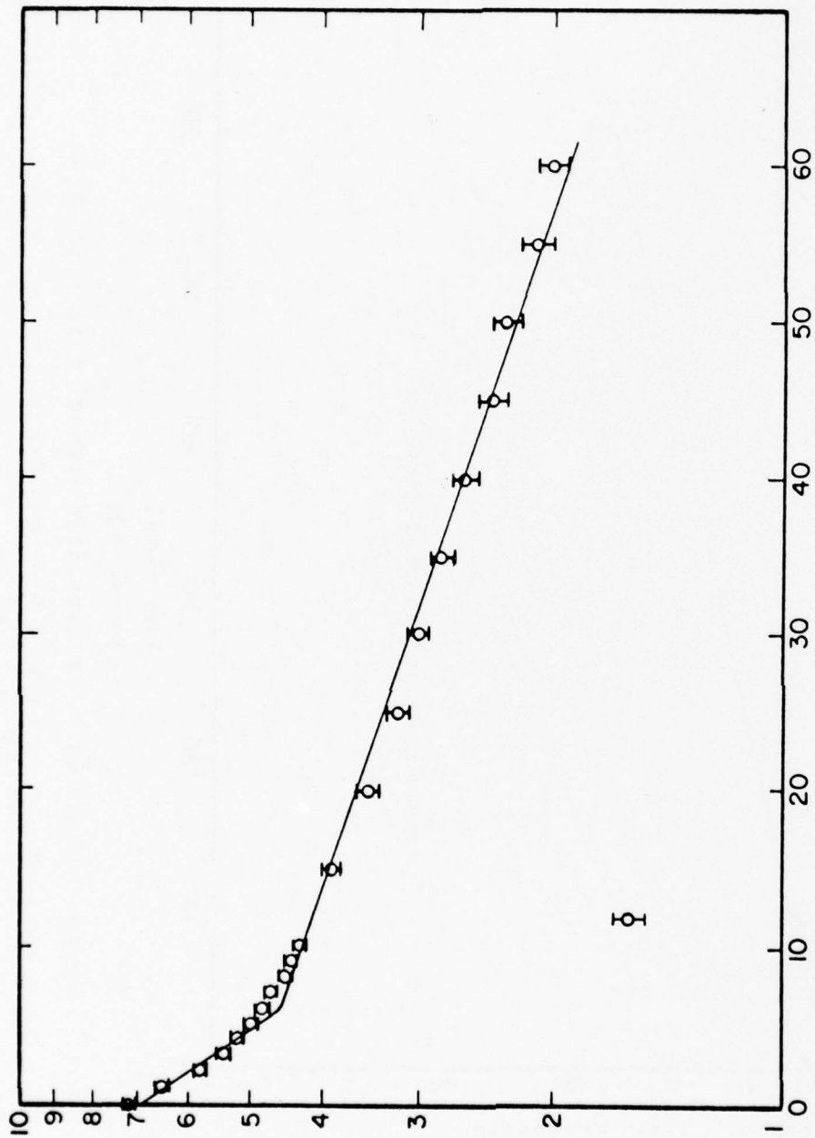
Oxygen Demand Test: Houston Ship Channel Site 3 Sediment Figure 113 (Sample size-3cc)
