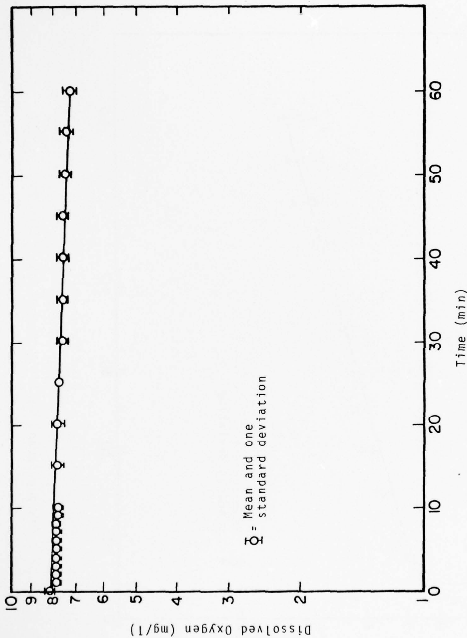
Figure 117 Oxygen Demand Test: Duwamish River Site 1 (Sample Size - 3 cc)
