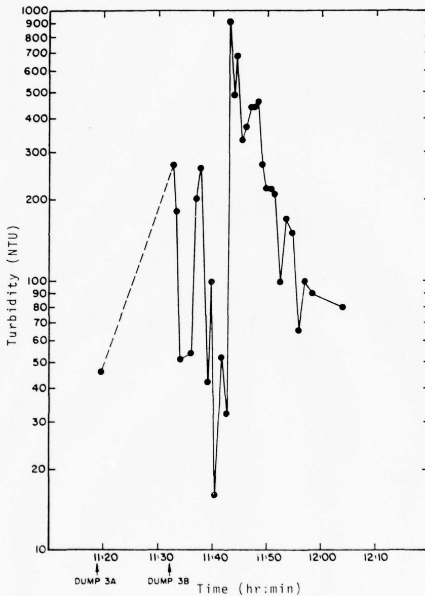
Figure 169 Turbidity in Near Bottom (23 m) Water during New York Bight Dump No.3 - Hudson
