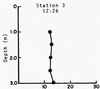
Figure 192 Water Column Profiles Transmissometer Data: Mobile Bay, Alabama - June 3, 1976
