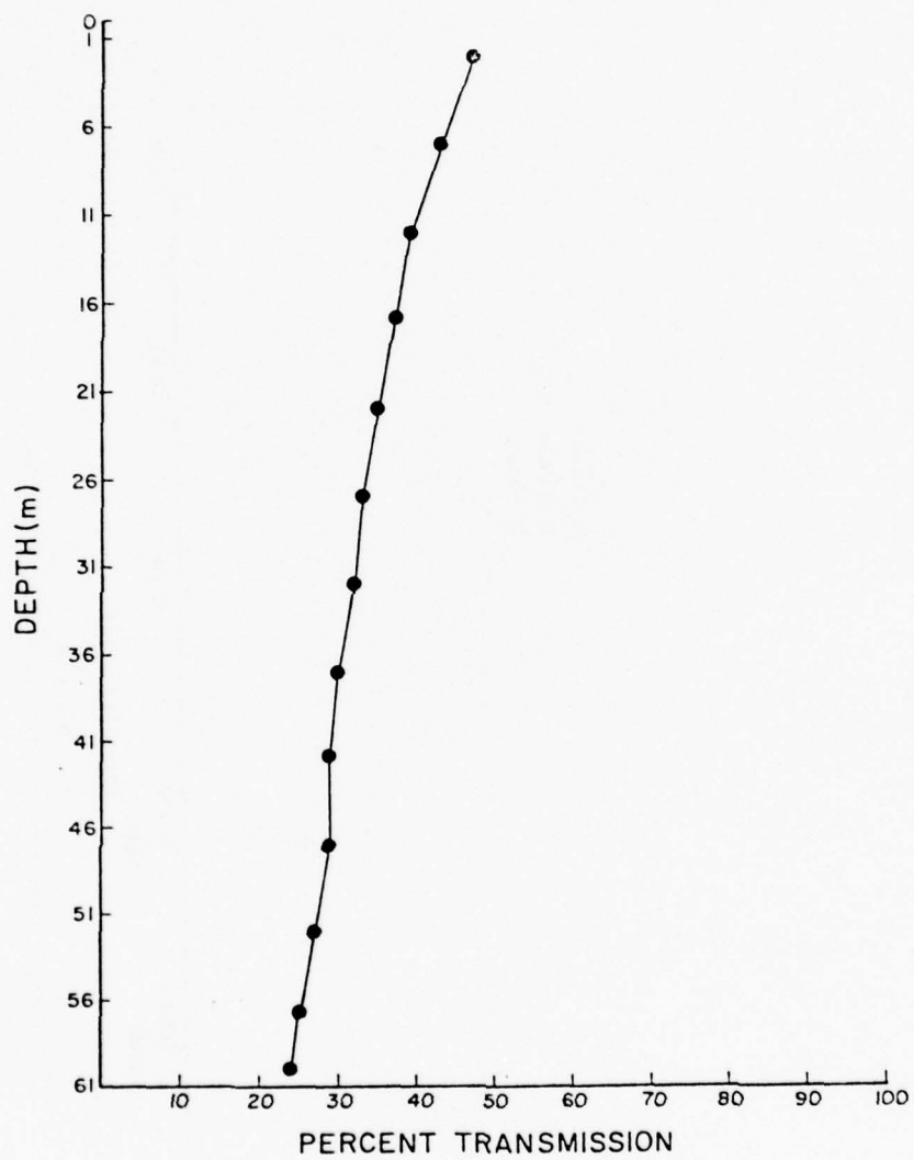
Figure 121 Percent Transmission Profile: Pre-Disposal Elliott Bay - 9:30
