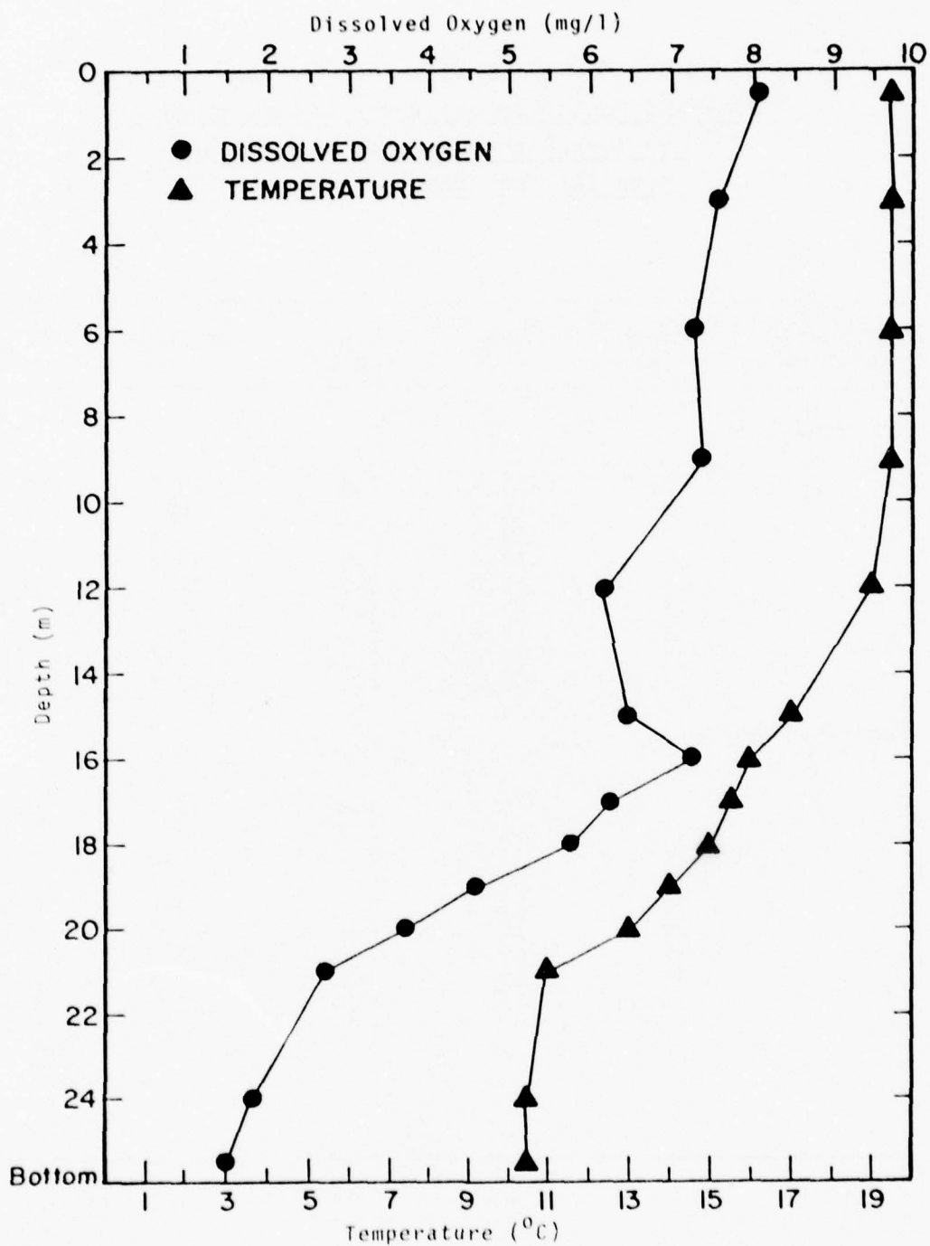
Figure 151 Pre-Disposal Temperature and Dissolved Oxygen Profiles: New York Bight Mud Dump Site Hatton
