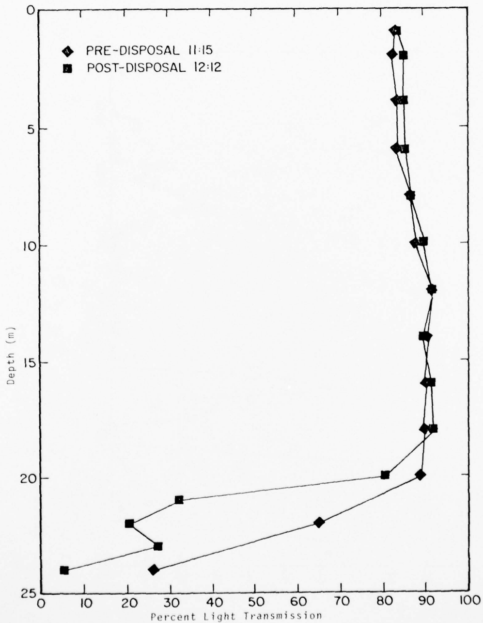
Figure 172 Water Column Profiles: Percent Light Transmission during New York Bight Dump No. 3 - Hudson
