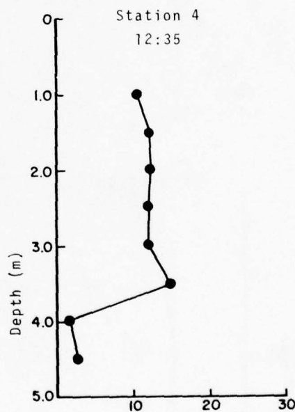
Figure 192 Water Column Profiles Transmissometer Data: Mobile Bay, Alabama - June 3, 1976
