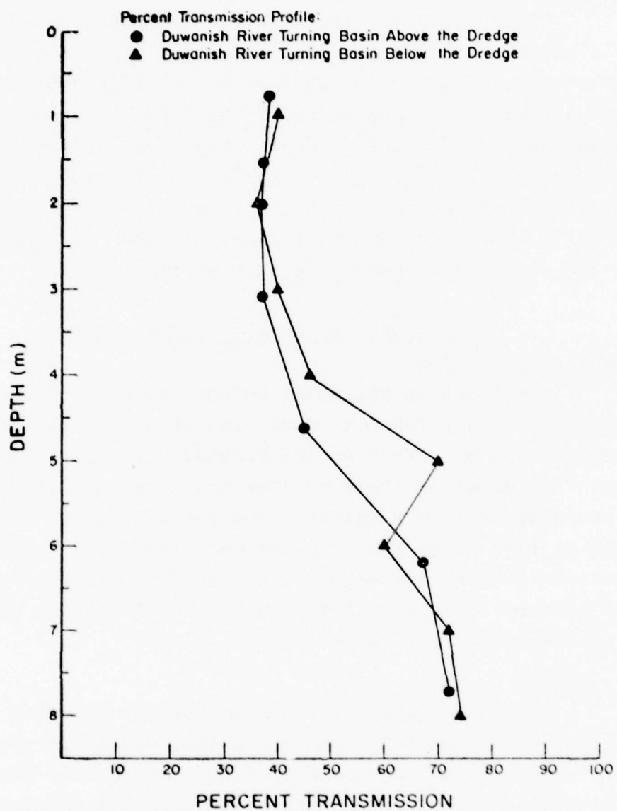
Figure 137 Percent Transmission Profile: Duwanish River Above and Below Dredge
