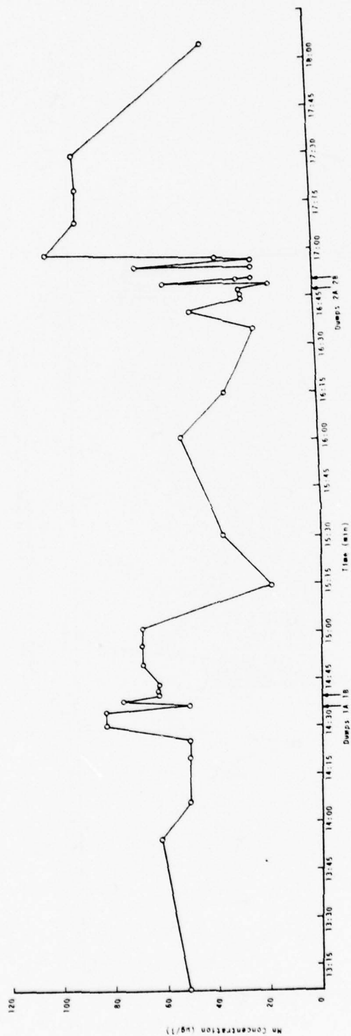
Figure 137 Soluble Manganese Concentrations at 1 Meter Depth, Elliott Bay Disposal Operations: Sediment from Hueshish River
