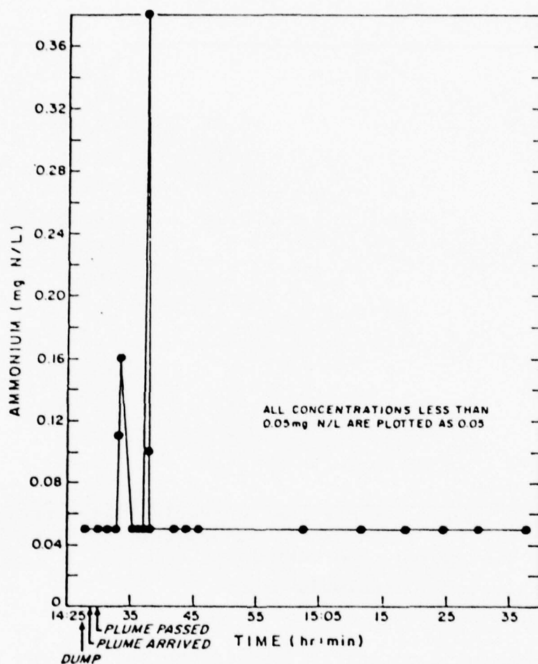
Figure 92 Ammonium Concentrations in Bottom Waters, Galveston Dump No. 5 near Buoy D, August 29, 1975
