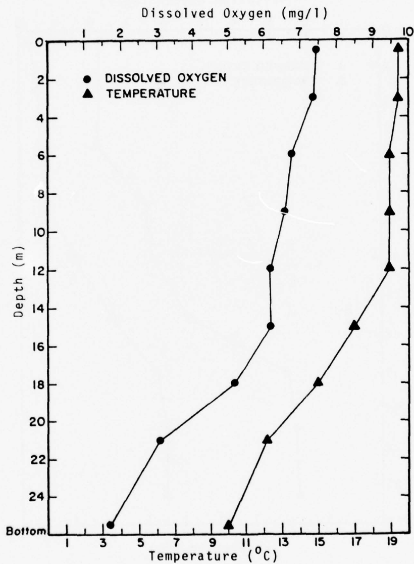
Figure 152 Pre-Disposal Water Column Temperature and Dissolved Oxygen Profile: New York Bight Dump No. 1 Hatton
