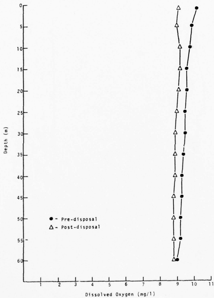
Figure 130 Pre- and Post-Disposal Dissolved Oxygen: Elliott Bay Dump No. 2 (February 17, 1976)
