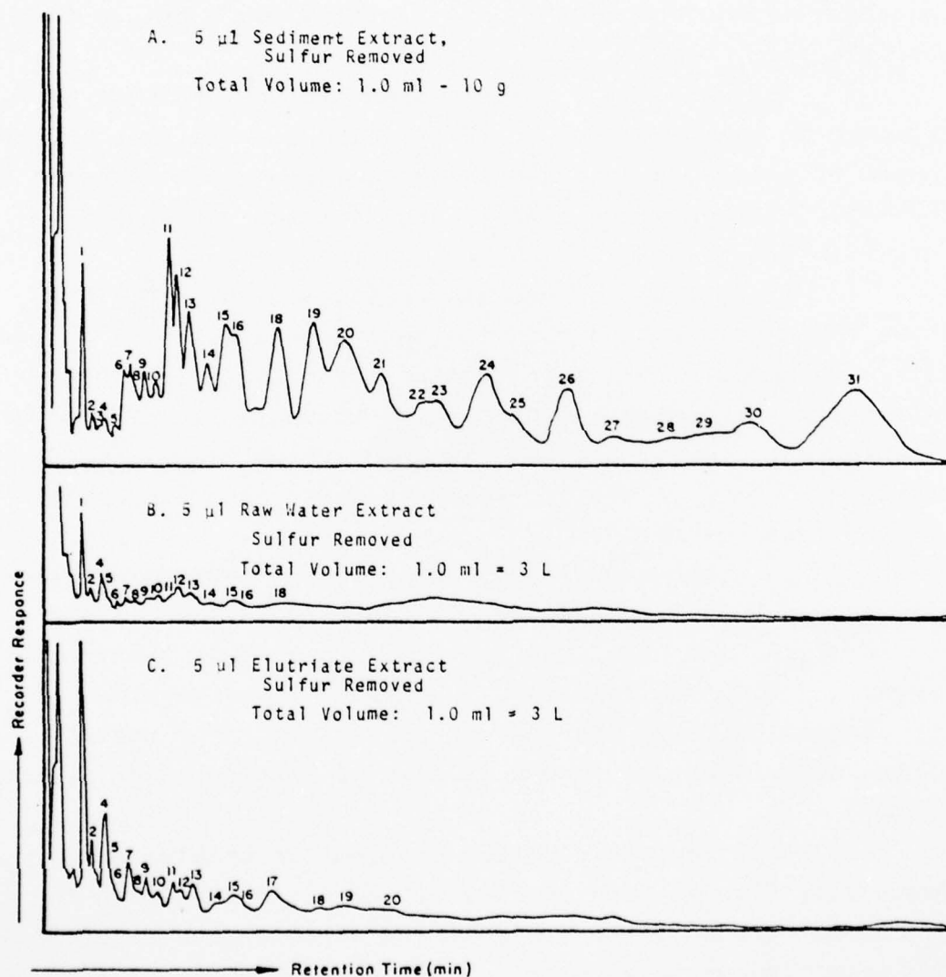
Figure 102 Profile of Organic Residues on GC Chromatograms: Texas City Channel Site 1 Sediment, Water and Elutriate
