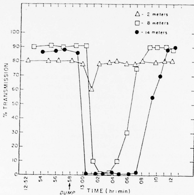
Figure 88 Percent Transmission: Galveston Dump No. 4 Dredged Material from Galveston Bay Entrance Channel, Buoys 1-3, August 29, 1975
