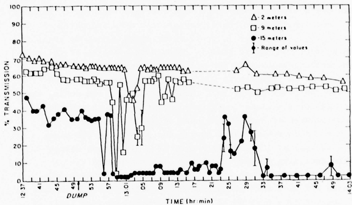
Figure 94 Percent Transmission: Galveston Dump No. 6 near Buoy D, Dredged Material from Galveston Bay Entrance Channel Buoys 3-7A, September 9, 1975
