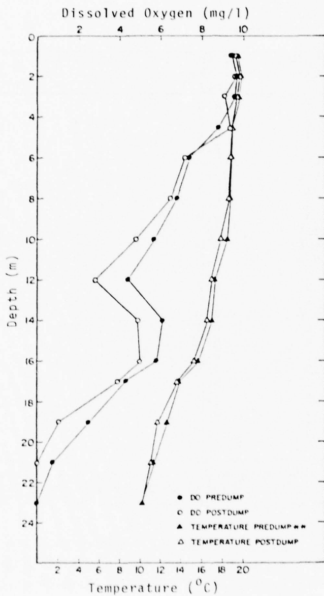
Figure 166 Pre- and Post-Dump Water Column D.O. and Temperature Profiles* New York Bight Dump No. 2 - Hudson
