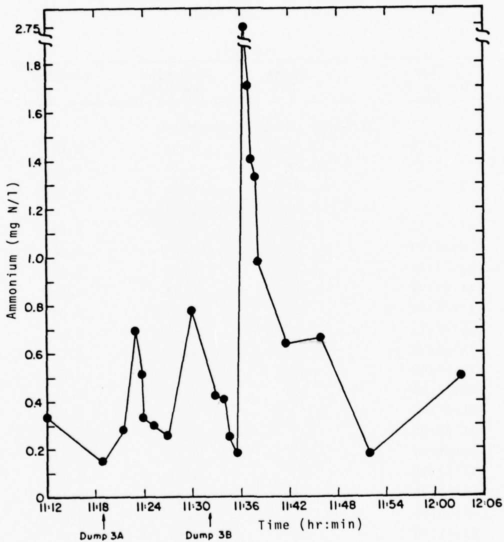
Figure 176 Ammonium Concentrations in Near Bottom Water as a Function of Time: New York Bight Dump Nos. 3A and 3B Hatton
