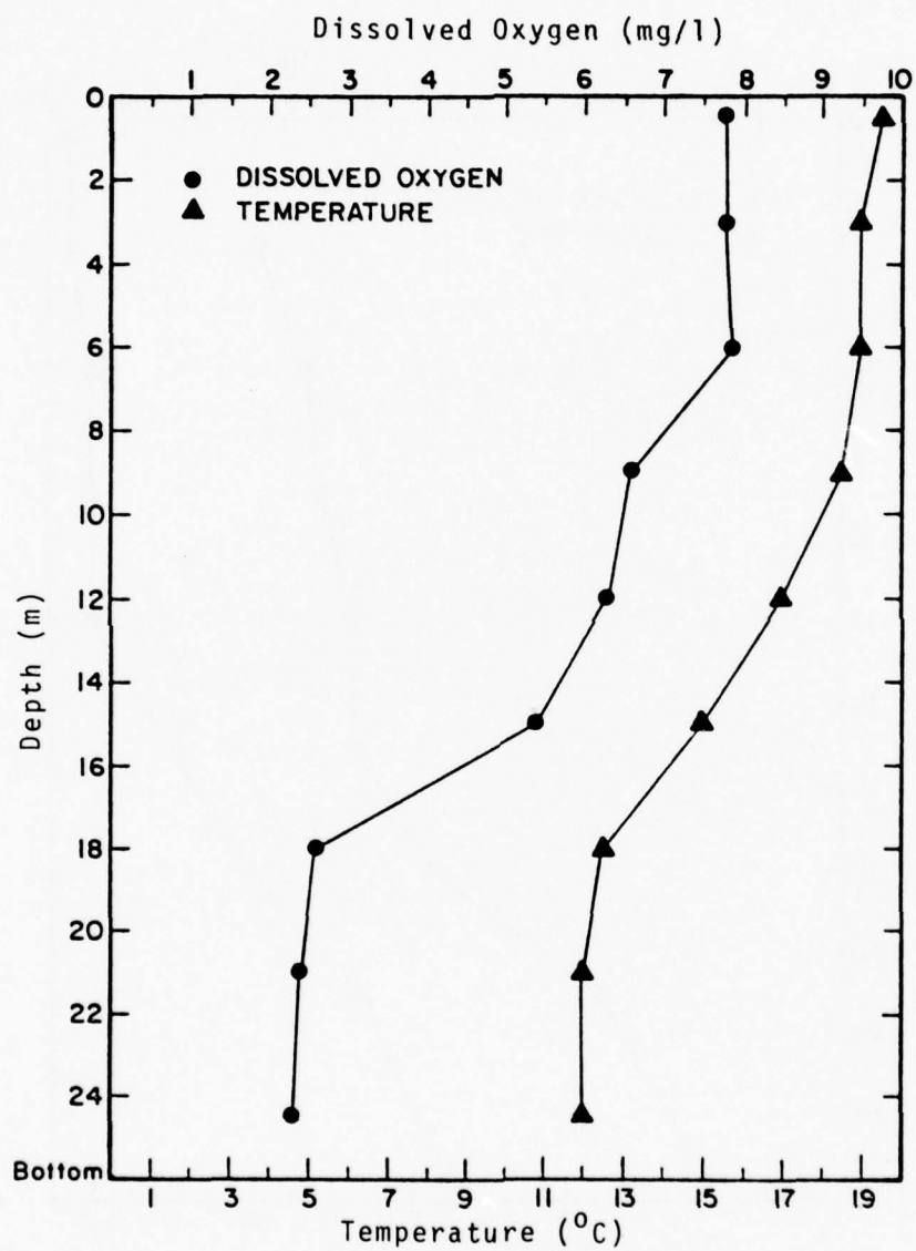
Figure 153 Post-Disposal Water Column Temperature and Dissolved Oxygen Profile: New York Bight Dump No. 1: Hatton
