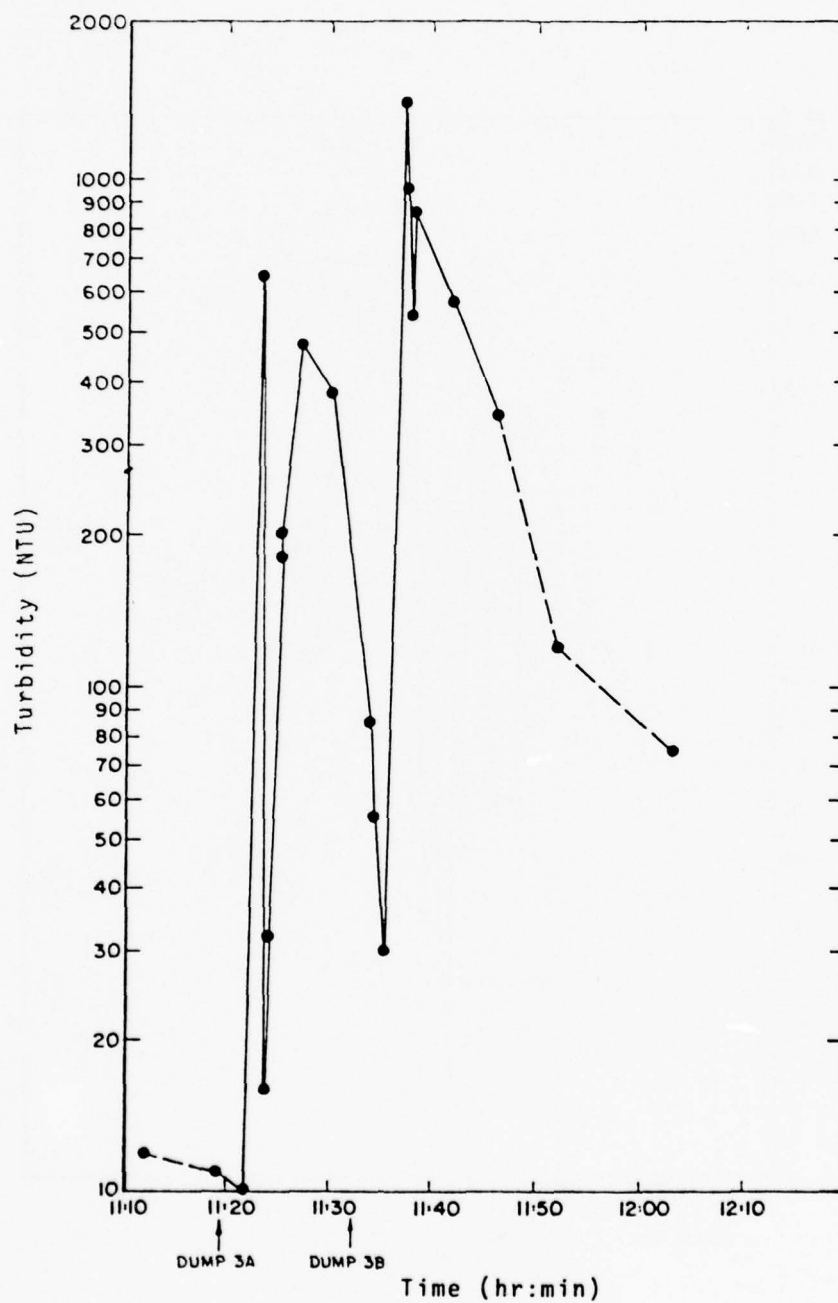
Figure 168 Turbidity in Near Bottom (24 m) Water During New York Bight Dump No.3 - Hatton
