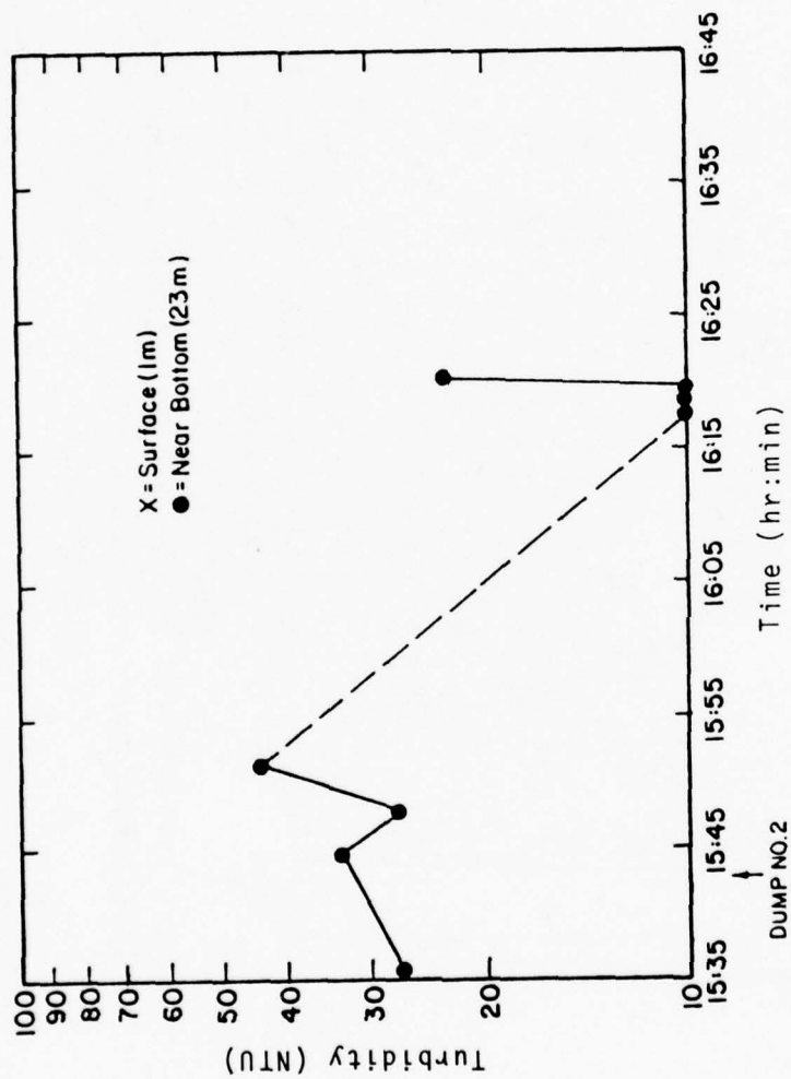
Figure 159 Turbidity in Surface and Near Bottom Water during New York Bight Dump No. 2 - Hudson
