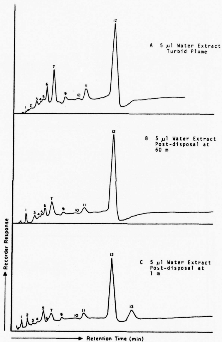
Figure 136 Profile of Organic Residues on GC Chromatograms Elliott Bay Dump No. 2
