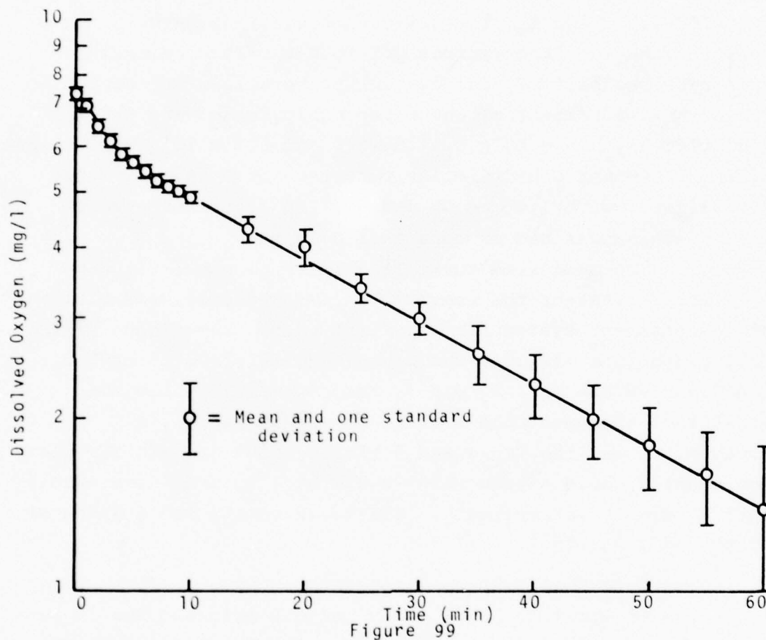
Figure 99 Oxygen Demand Test: Texas City Channel Site 4 Sediment (Sample size - 3 cc)
