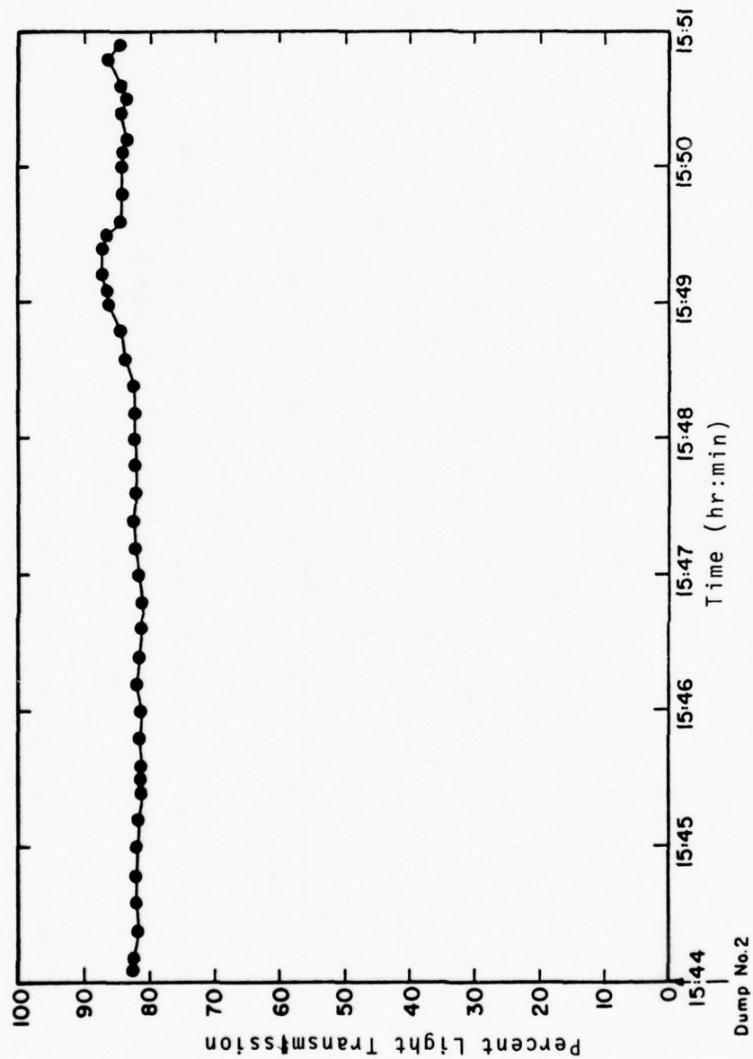
Figure 162 Percent Light Transmission during New York Bight Dump No. 2 Depth - 3 meters - Hudson
