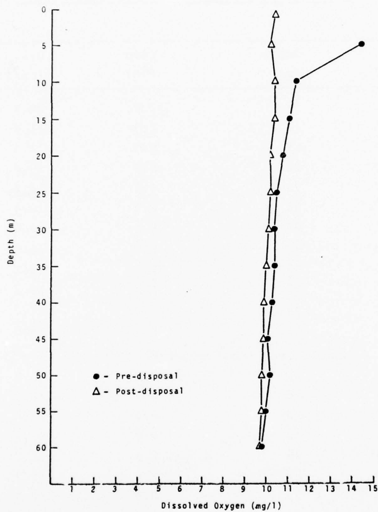
Figure 127 Changes in Dissolved Oxygen: Elliott Bay Unmonitored Disposal Operation (February 17, 1976)
