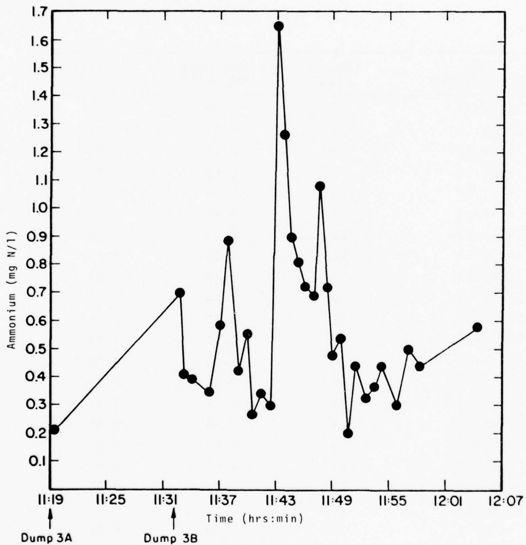
Figure 177 Ammonium Concentrations in Near Bottom Water as a Function of Time: New York Bight Dump Nos. 1, 3A & 3B-Hudson
