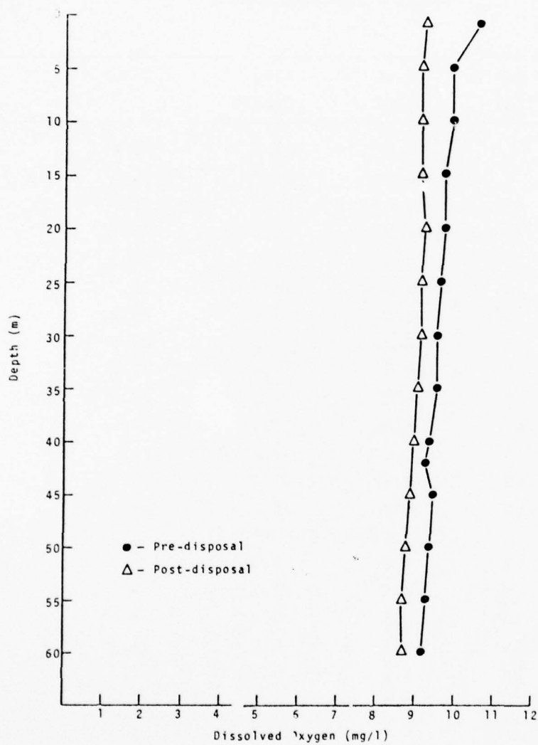
Figure 128 Pre- and Post-Disposal Dissolved Oxygen: Elliott Bay Dump No. 1 (February 17, 1976)
