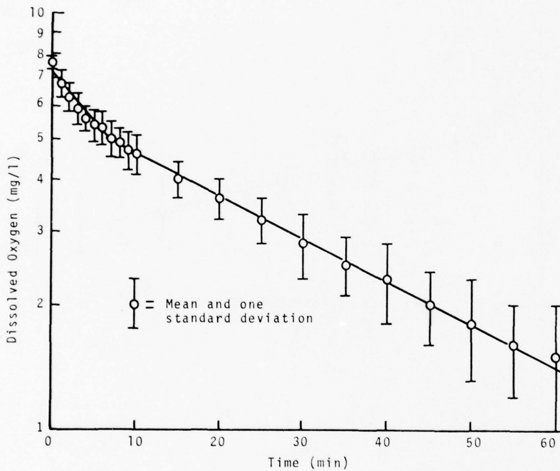
Figure 101 Oxygen Demand Test: Texas City Channel Site 6 Sediment (Sample size - 3 cc)
