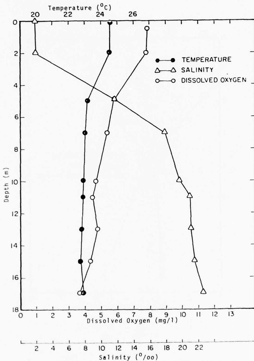
Figure 184 Temperature, Dissolved Oxygen, Salinity Profiles: Mobile Bay, Alabama 15 m in front of dredge June 2, 1976
