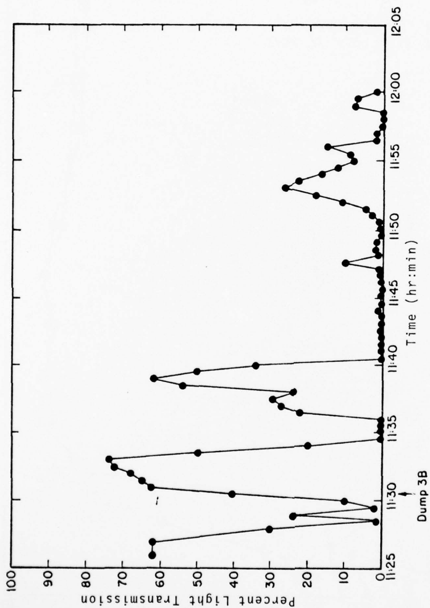
Figure 173 Percent Light Transmission: New York Bight Dump No.3 Depth 23 m - Hudson
