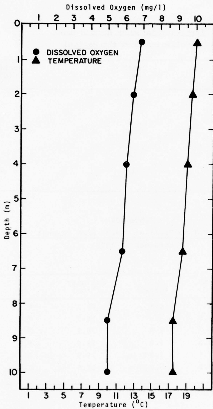
Figure 178 Water Column Temperature and Dissolved Oxygen Profile: Sandy Hook Channel - September 1, 1976
