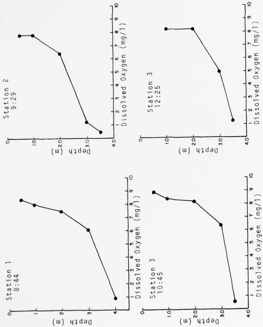
Figure 189 Dissolved Oxygen Profiles: Mobile Bay, Alabama June 3, 1976
