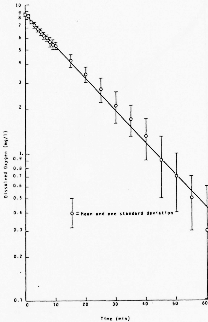
Figure 97 Oxygen Demand Test: Texas City Site 1 Sediment (Sample Size - 5 cc)
