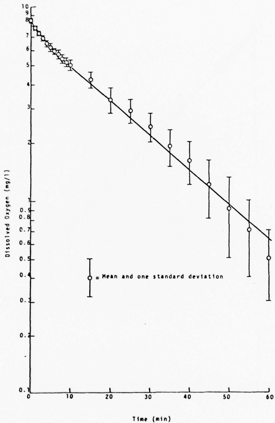
Figure 98 Oxygen Demand Test: Texas City Site 2 Sediment (Sample size - 5 cc)
