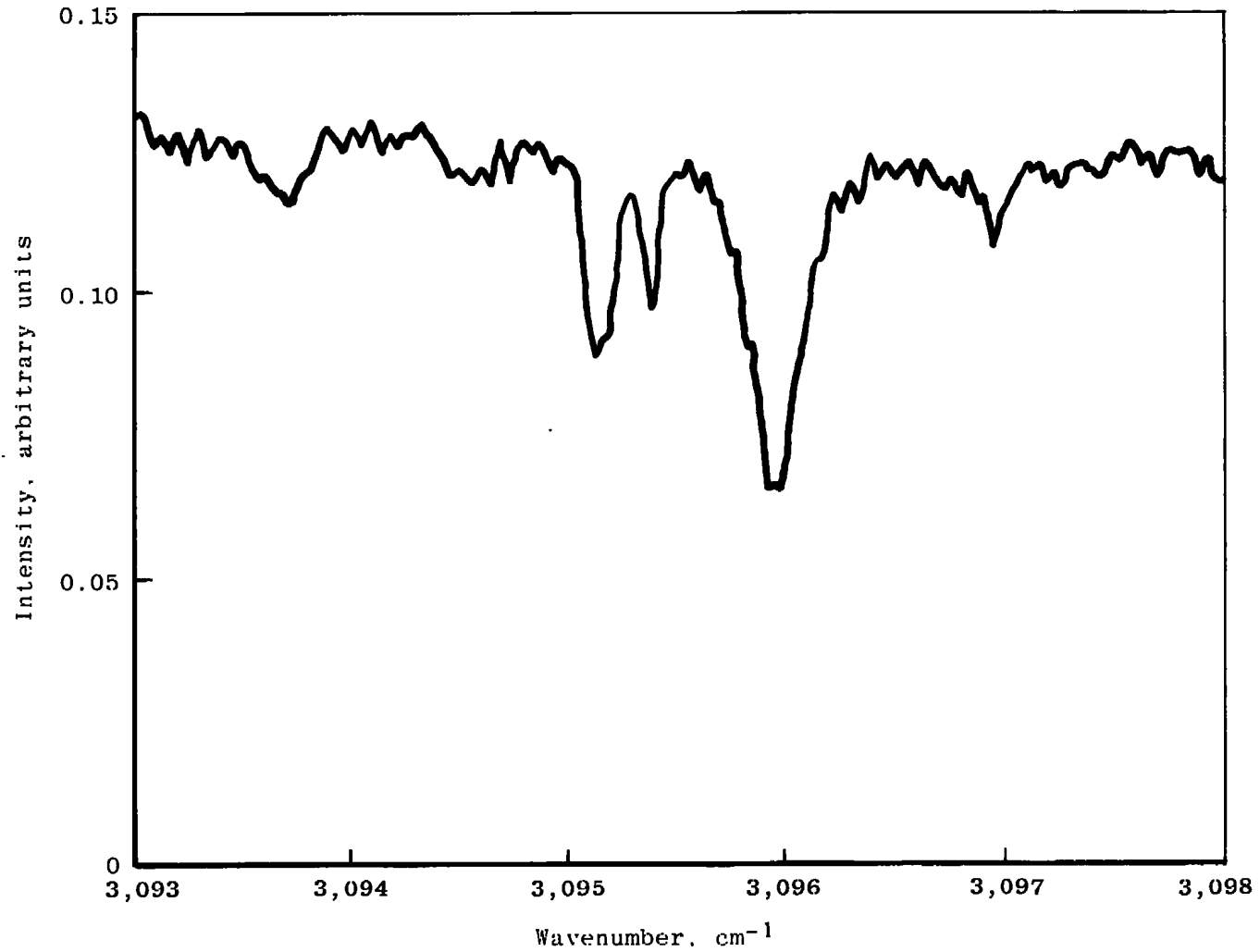
Figure 10. Absorption spectrum of methane in nitrogen at 773°K, R 7 line, methane concentration 996 ppm, pressure 97.9 kPa, pathlength 50.7 cm.
