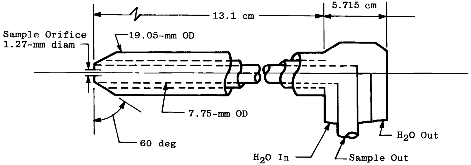
Figure 26. Diagram of emissions probe.
