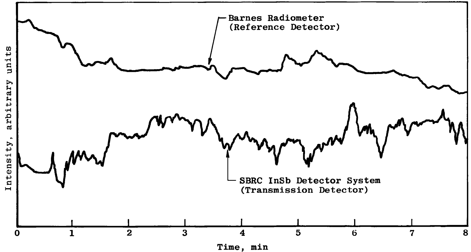
Figure 21. Simultaneous recordings of He-Ne IR laser power monitors; upper trace, filter radiometer; lower trace, InSb detector system, chart speed 2.54 \text{ cm}\cdot\text{min}^{-1} .
