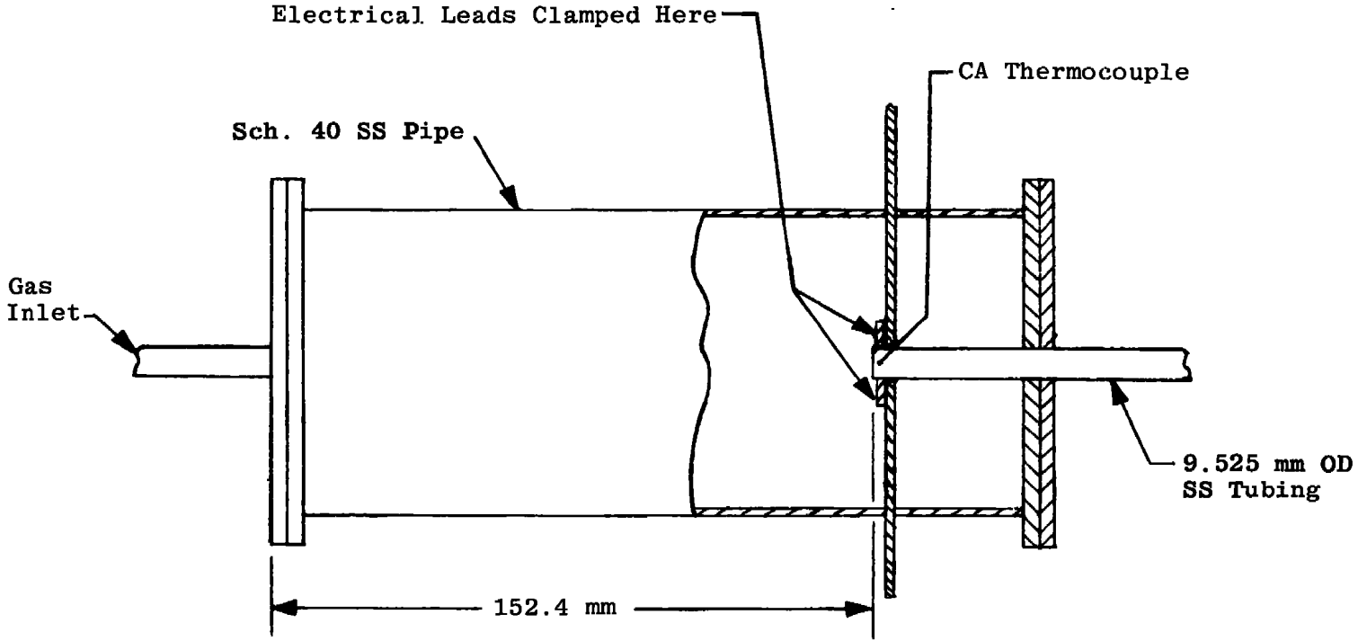
Figure 24. Probe simulator.
