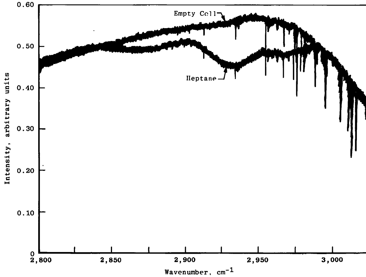
Figure 16. Absorption spectrum of heptane in nitrogen and empty cell spectrum at 573°K, heptane concentration 516.8 ppmv, pressure 97.9 kPa, pathlength 50.7 cm.
