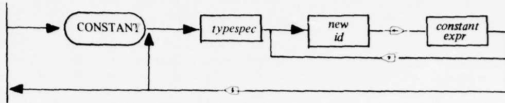
Figure 1. Example Syntax Chart.
