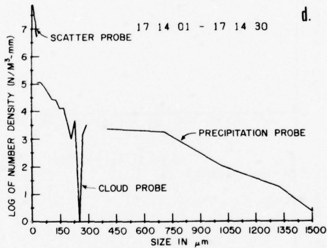
Figure 16. Particle Concentration as a Function of Particle Size for Two Sampling Times. (c) Time when visibility further reduced, (d) time when LWC and median diameter reached peak for the sample period
