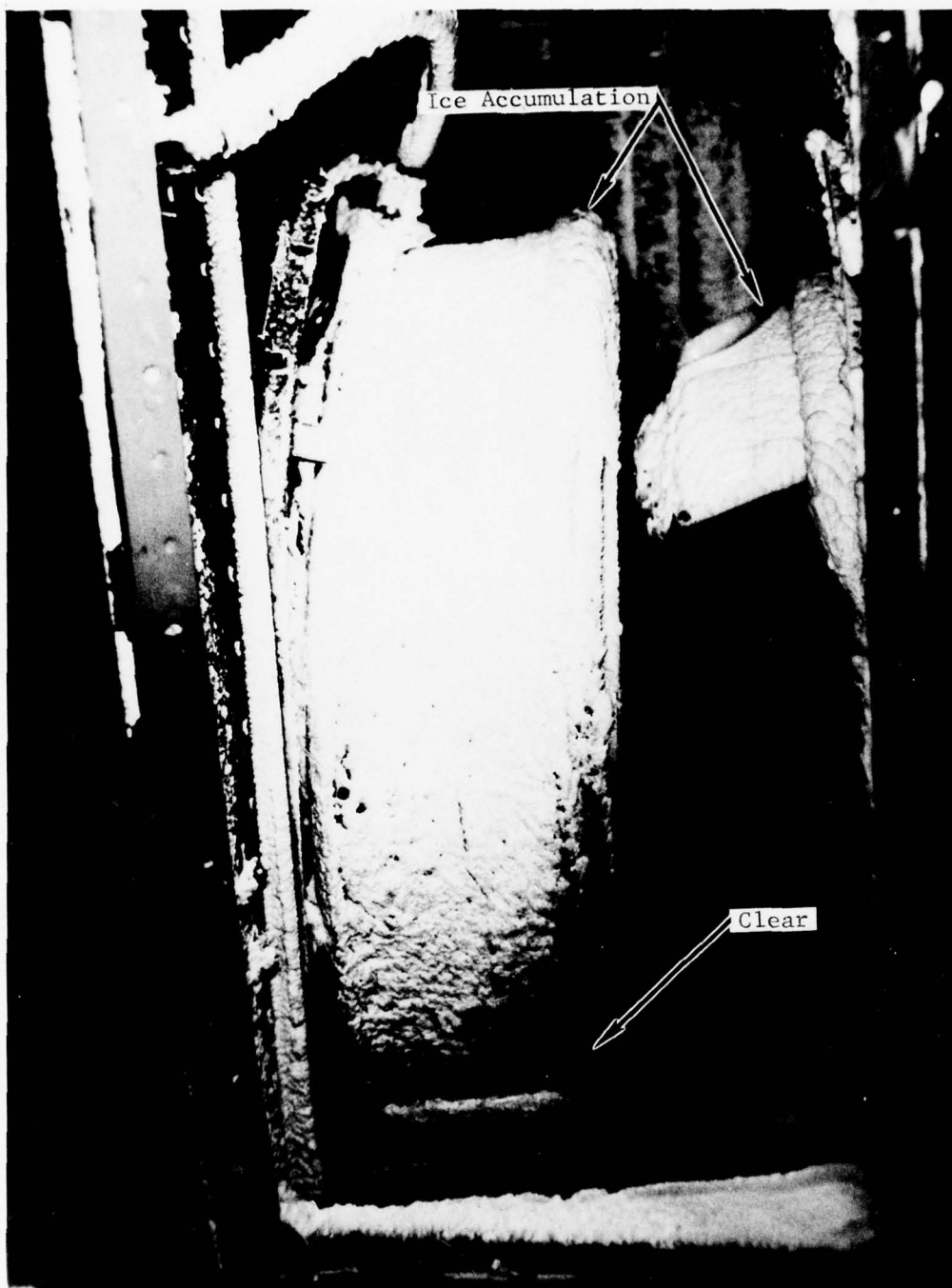
ICE ACCUMULATION ON THE COMPRESSOR INLET SCREEN AFTER 58 MINUTES IN THE SPRAY RIG AT -20.4^{\circ}\text{C}
