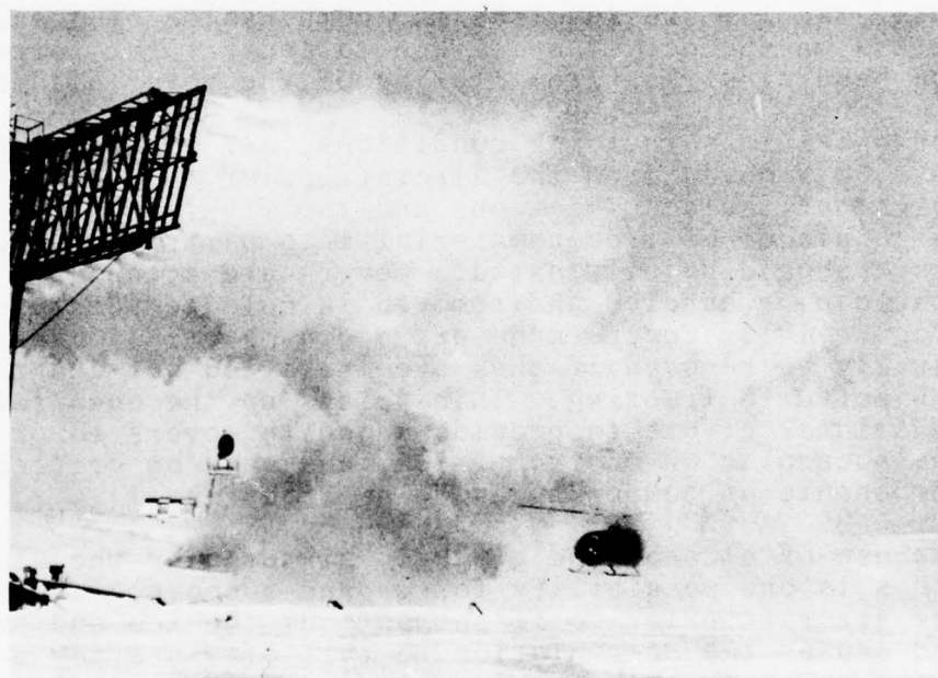
Figure 9. BO 105 Helicopter in the Icing Spray Rig at Uplands, Ottawa, Canada
