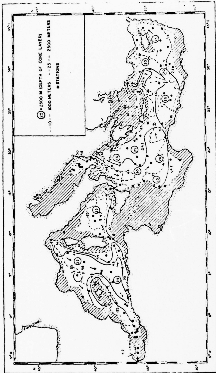
Figure 8. Distribution of oxygen within the core layer of the deep water (Müst, 1961).
