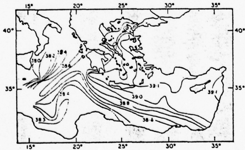
Figure 14. Surface isohalines in winter (Armanda, 1969).
