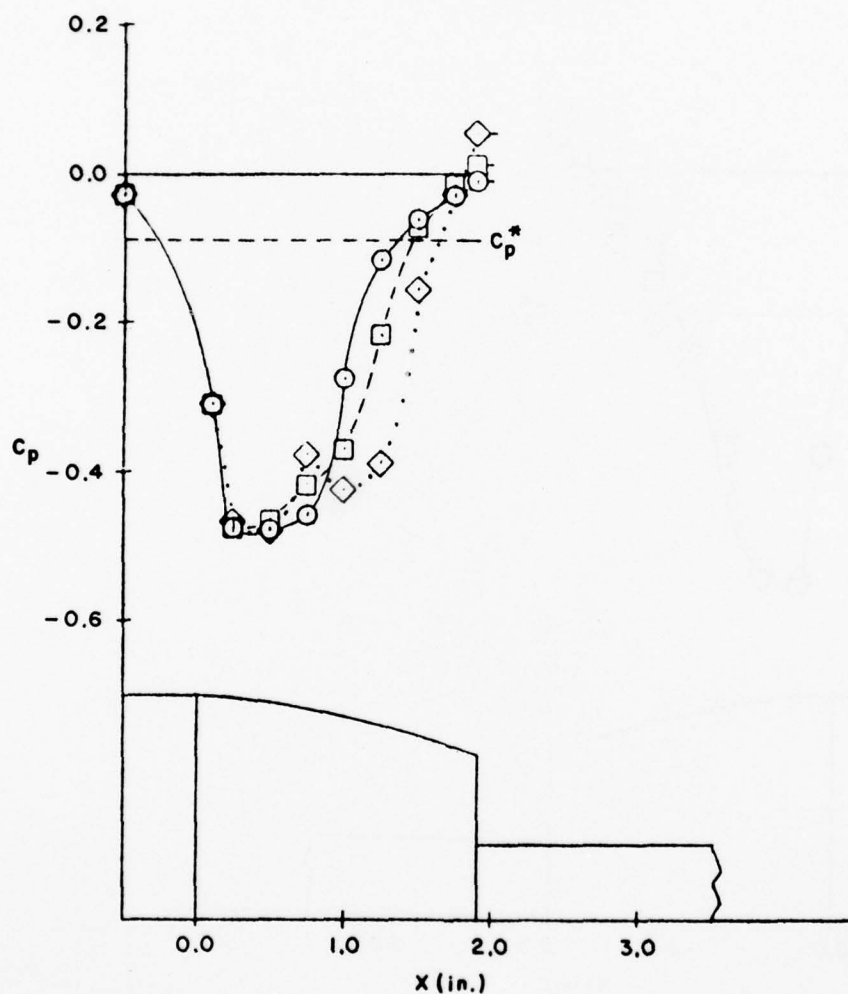
Figure 52. Mass Injection Effect on Boattail and Base Pressure Coefficients for NPR=2.0, D_S=1"
