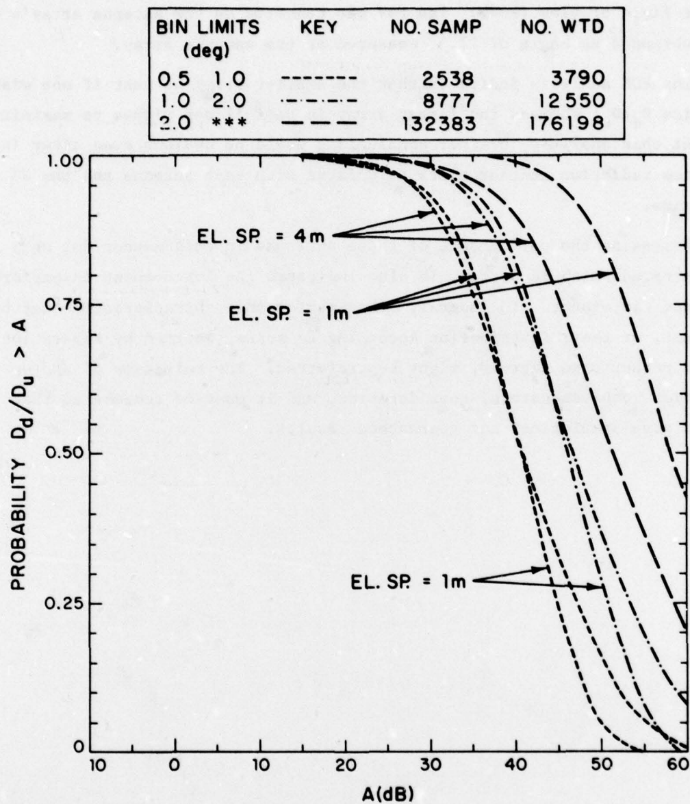
Fig. 8. D_u/D_d FOM.
