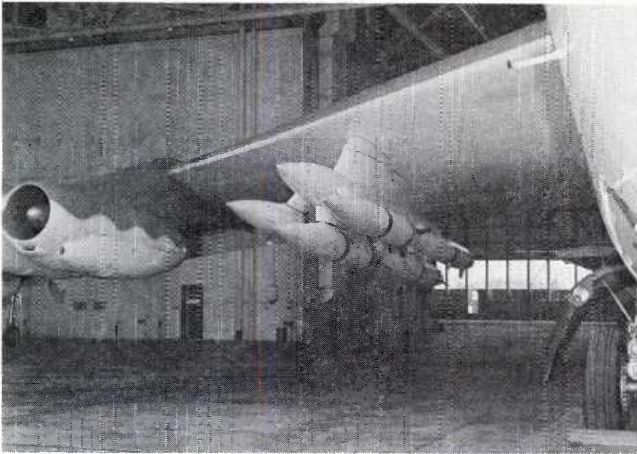
SRAM on B-52 pylon at Loring AFB, Maine
