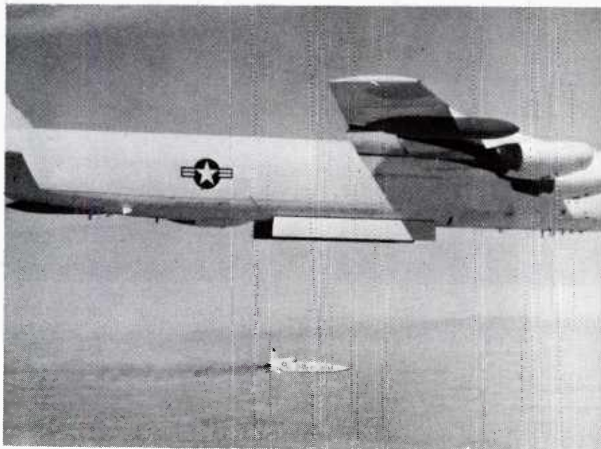
ALCM launched from a B-52, March 1976
