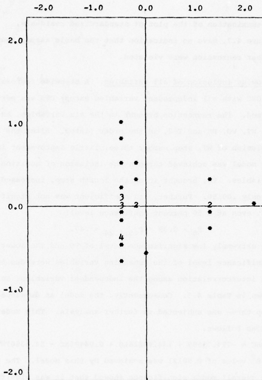
Figure 4.7 Residual Plot for AC/TG
