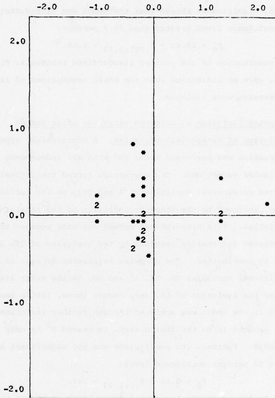
Figure 4.8 Residual Plot for LH/AC/WT
