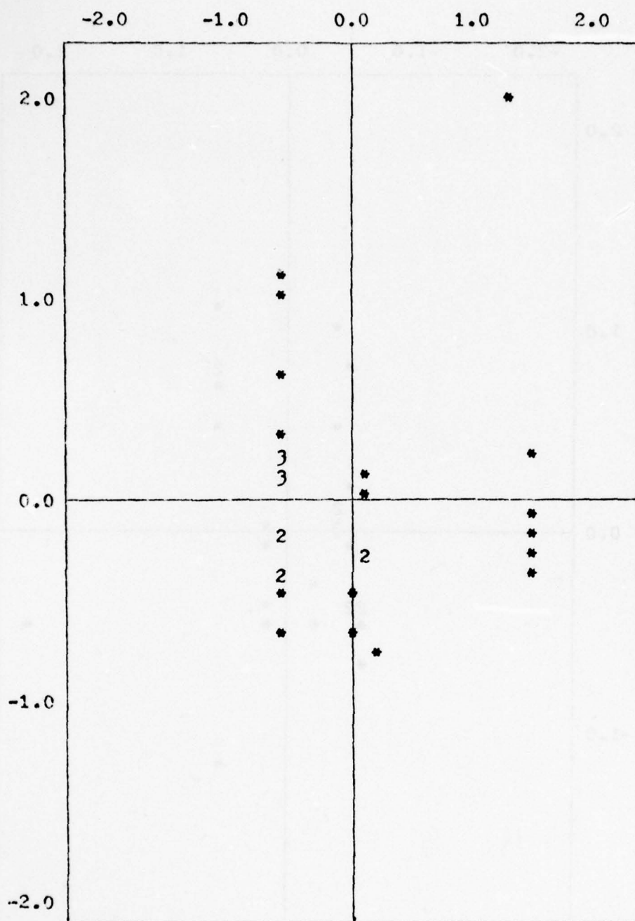
Figure 4.2 Residual Plot for WT
