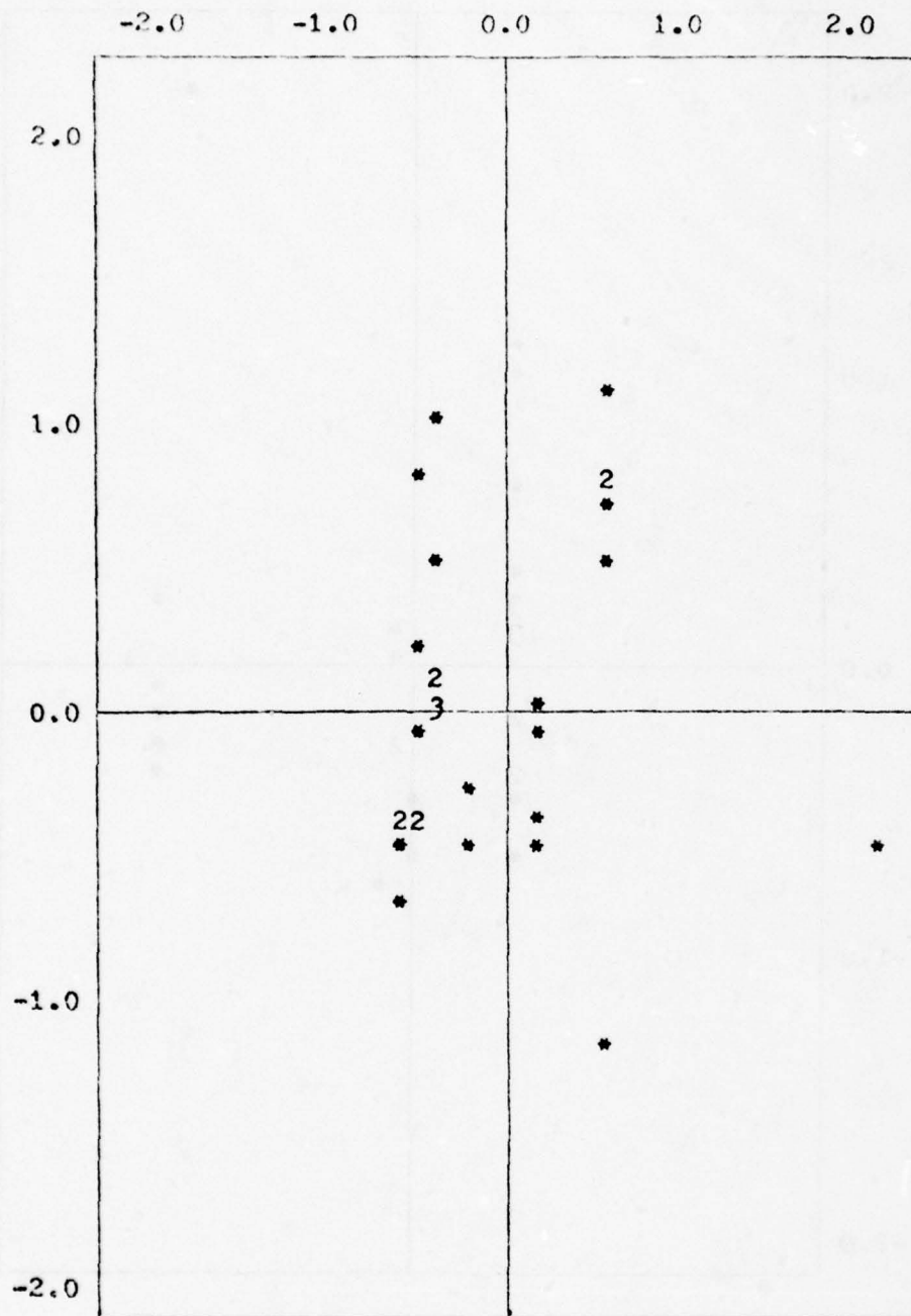
Figure 4.1 Residual Plot for AC
