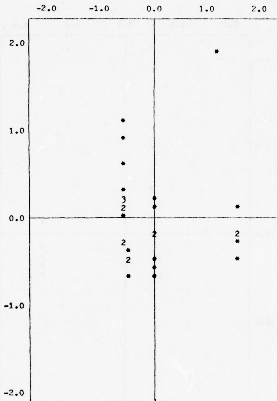
Figure 4.4 Residual Plot for VO
