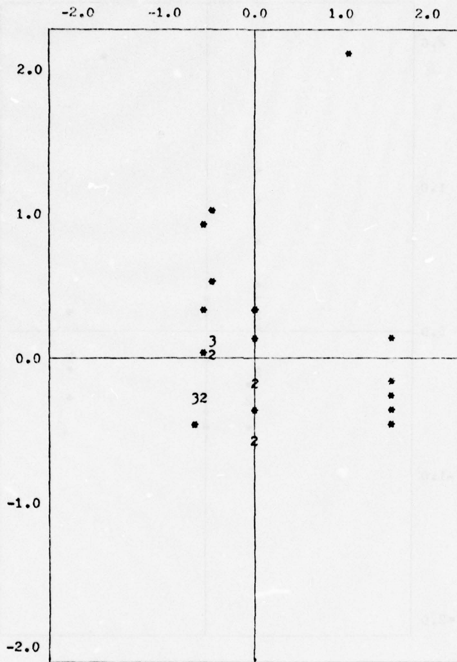
Figure 4.3 Residual Plot for LH
