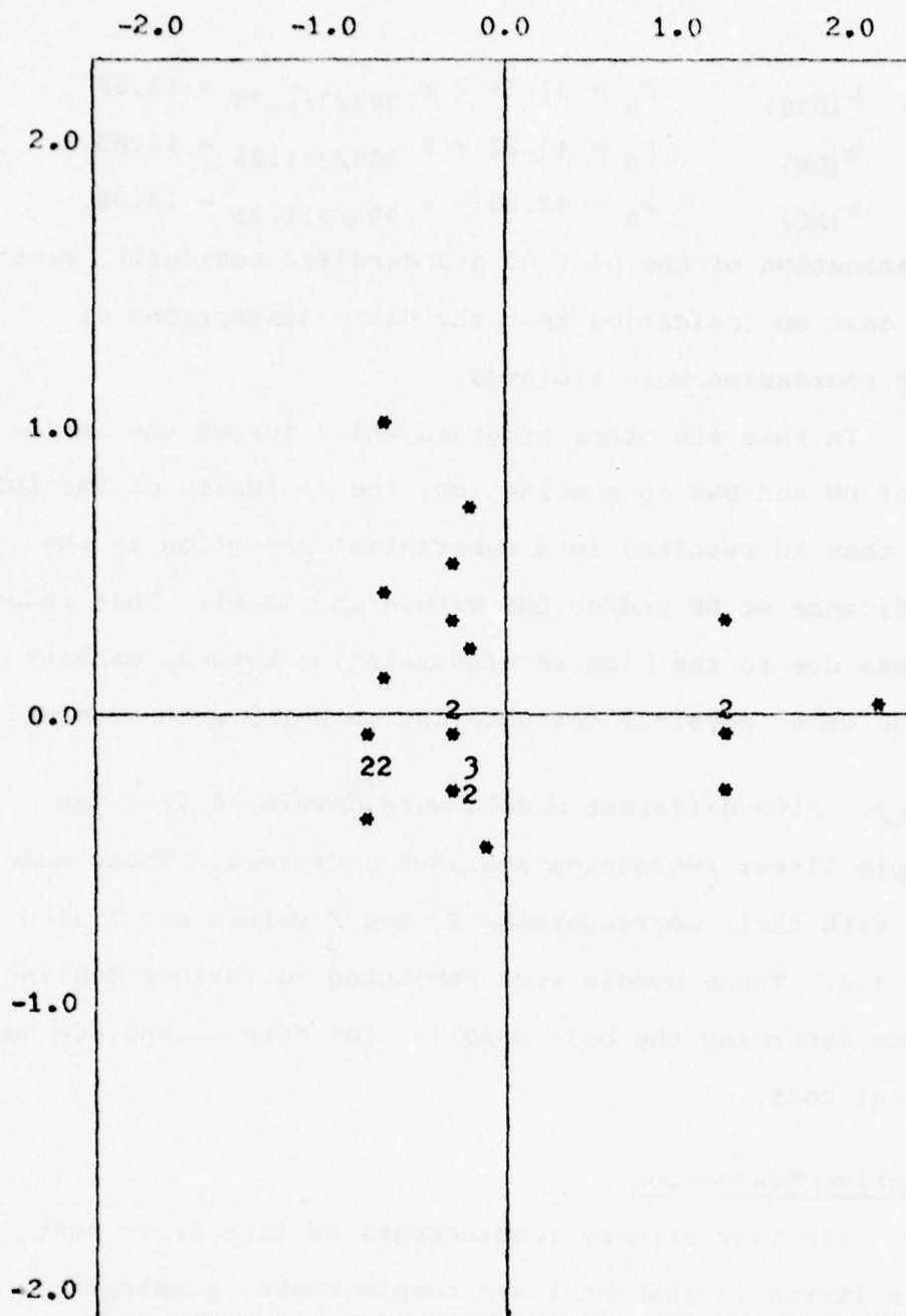
Figure 4.11 Residual Plot for DNS/DN/AC
