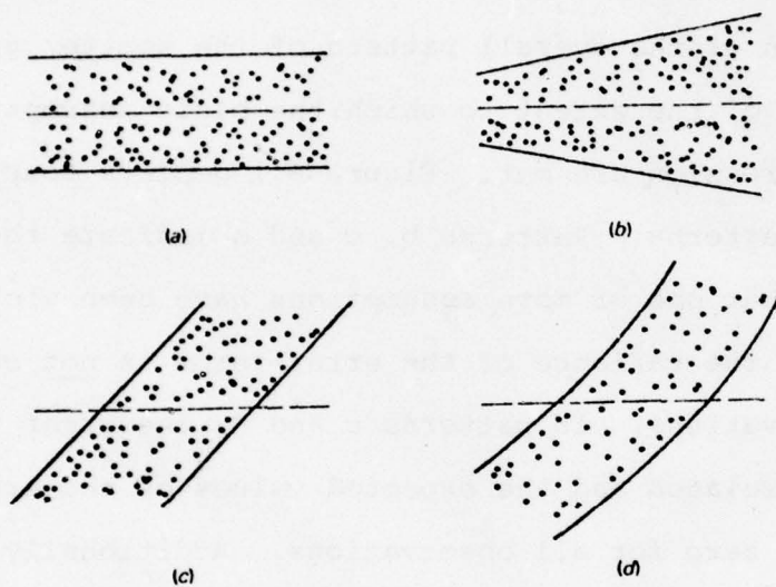
Figure B.1 Basic Scatterplot Patterns
