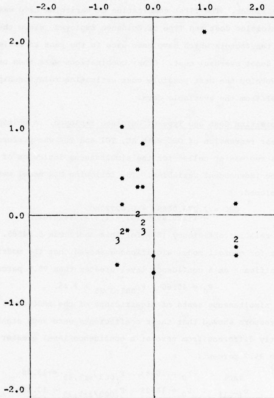
Figure 4.6 Residual Plot for DN/DNS
