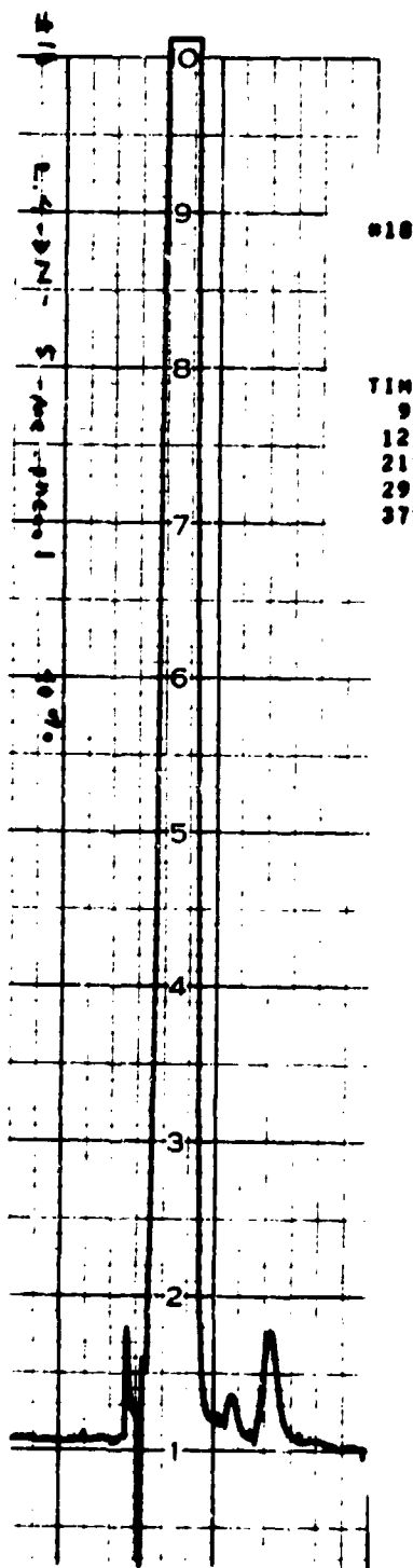
FIGURE 143 HPLC CHROMATOGRAM OF 2,4-DINITRO-5-METHYLPHENOL
