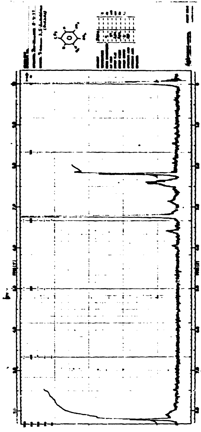
FIGURE 105 NMR SPECTRUM OF 4-AMINO-3,5-DINITROTOLUENE
