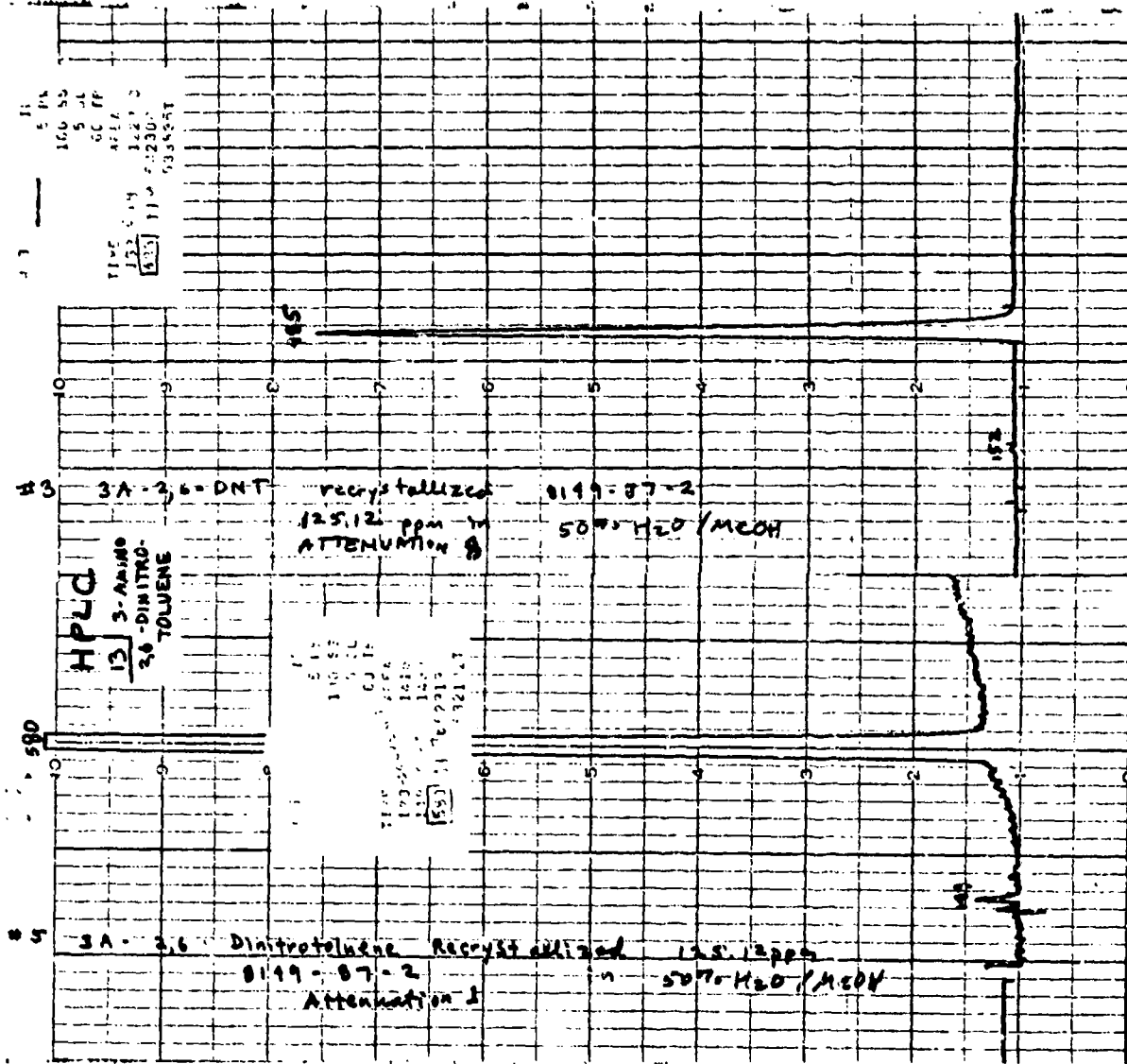
FIGURE 113 HPLC CHROMATOGRAMS OF 3-AMINO-2,6-DINITROTOLUENE
