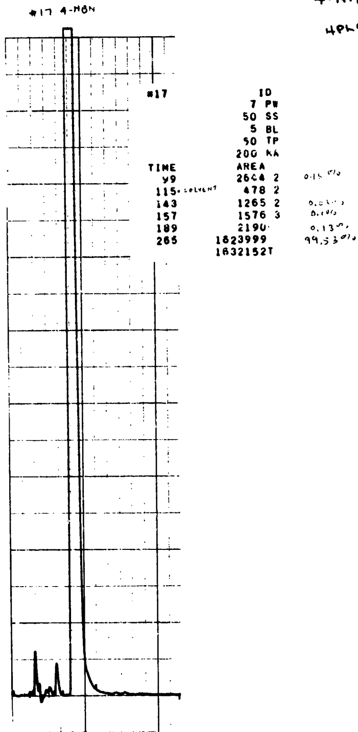
FIGURE 150 HPLC CHROMATOGRAM OF 4-NITROBENZONITRILE
