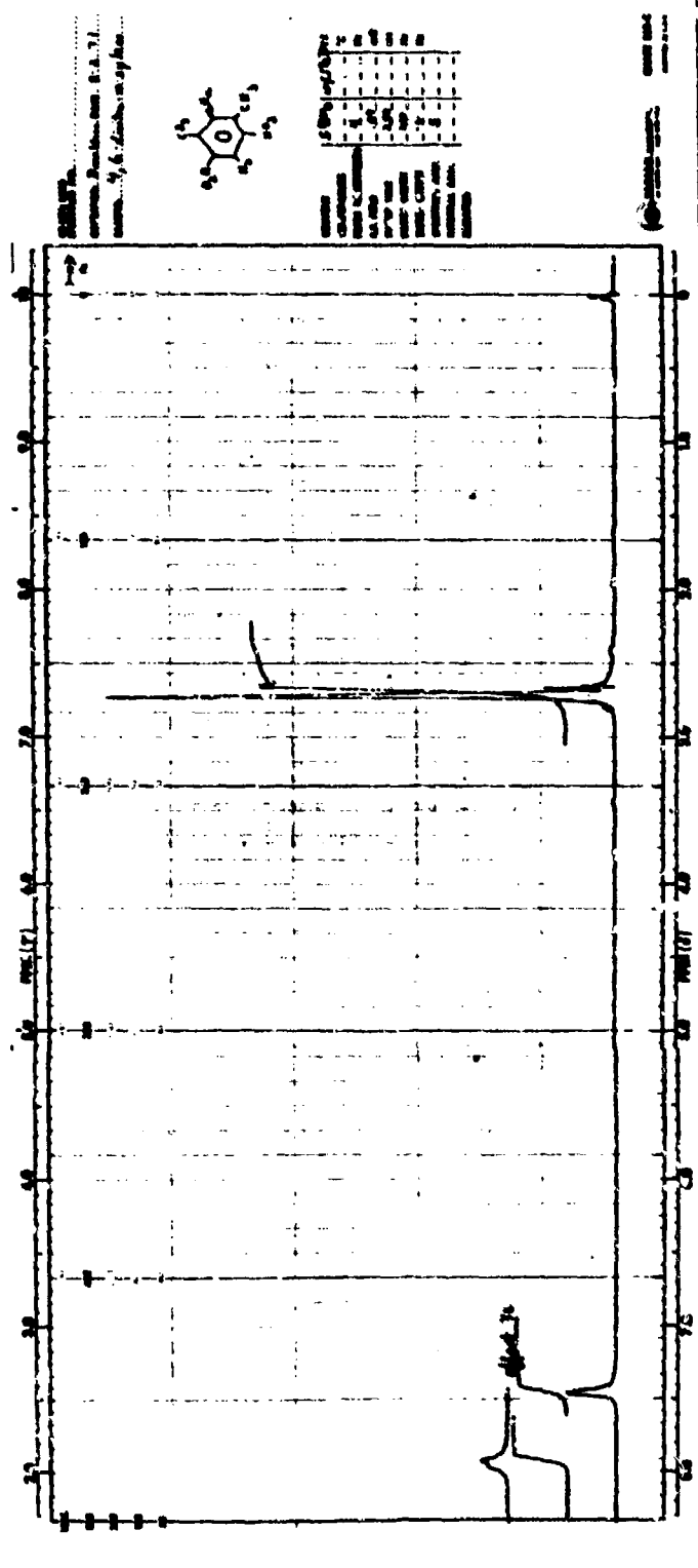
FIGURE 60 NMR SPECTRUM OF 4,6-DINITRO-m-XYLENE
