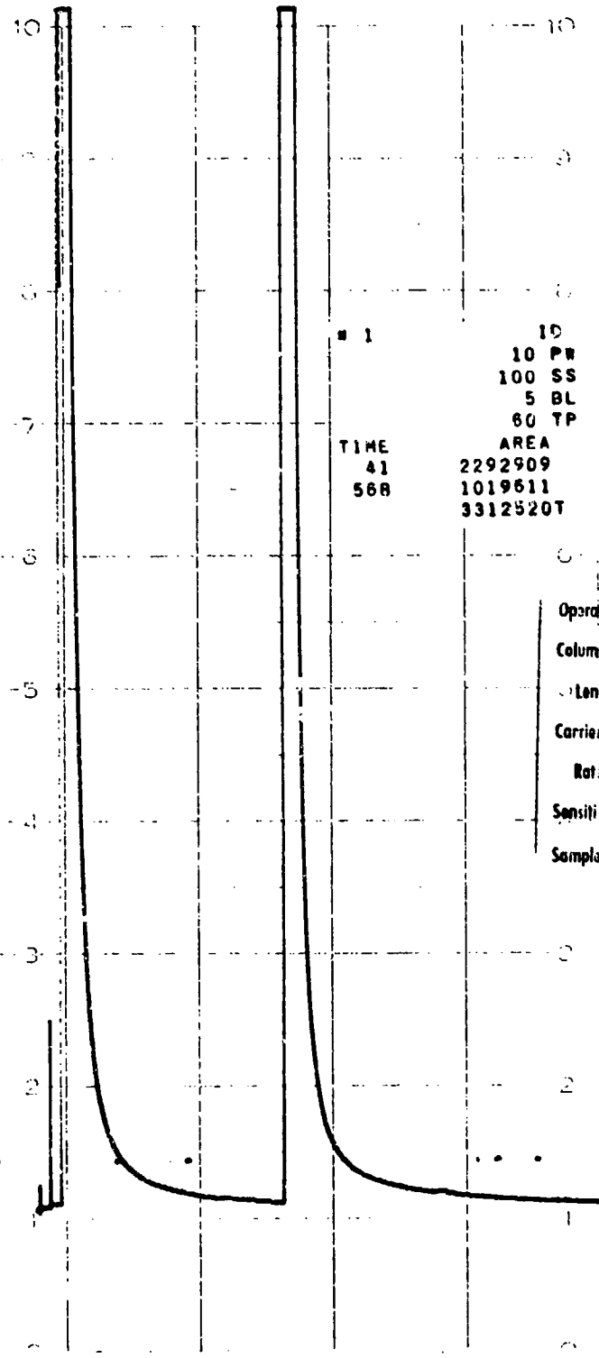
FIGURE 29 GC SPECTRUM OF 3-METHYL-2-NITROPHENOL
