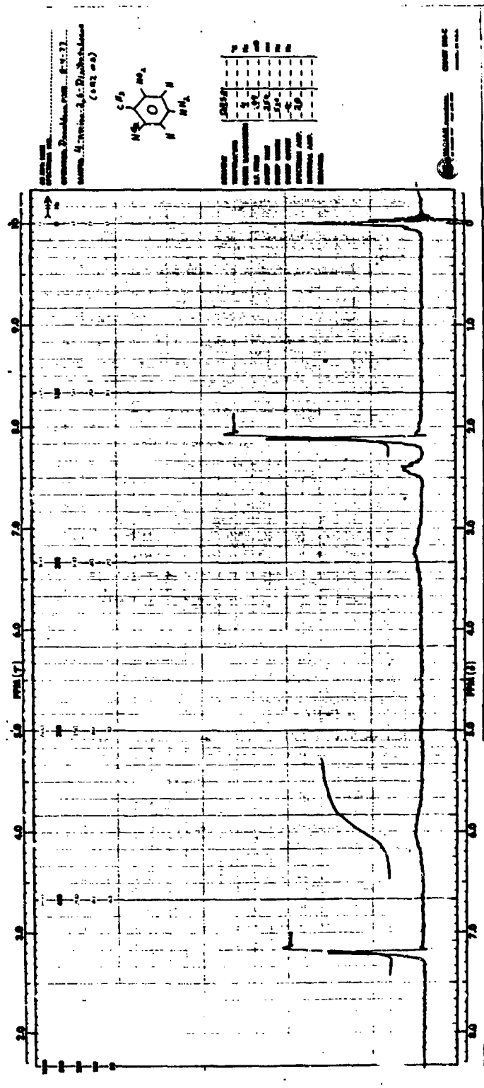
FIGURE 117 NMR SPECTRUM OF 4-AMINO-2,6-DINITROTOLUENE
