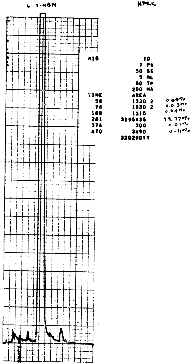
FIGURE 162 HPLC CHROMATOGRAM OF 3-NITROBENZONITRILE
