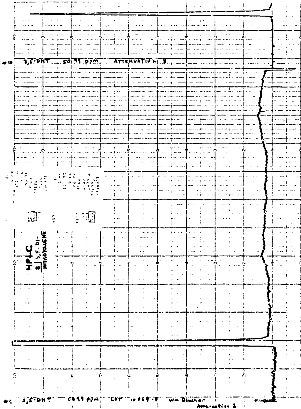
FIGURE 70 HPLC CHROMATOGRAM OF 3,5-DINITROTOLUENE
