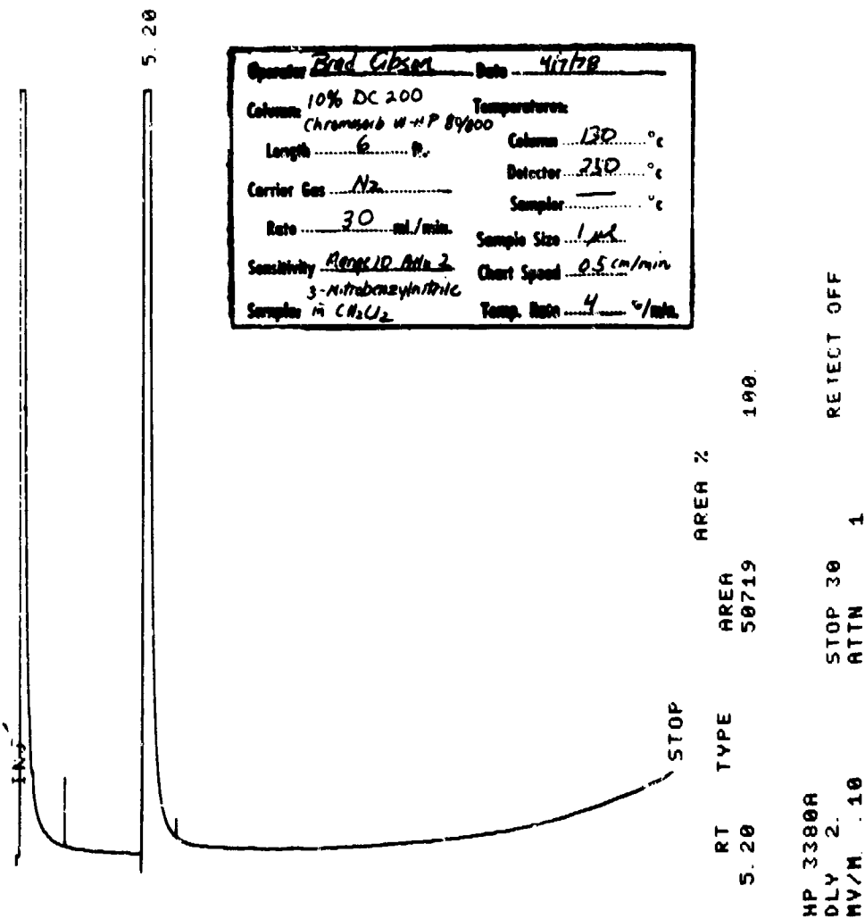
FIGURE 161 GC SPECTRUM OF 3-NITROBENZONITRILE
