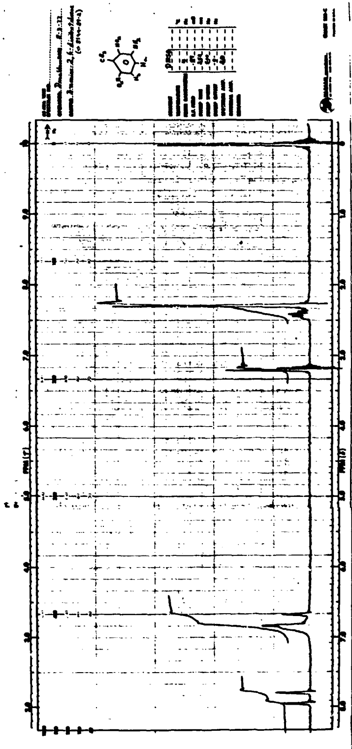
FIGURE 111 NMR SPECTRUM OF 3-AMINO-2,6-DINITROTOLUENE
