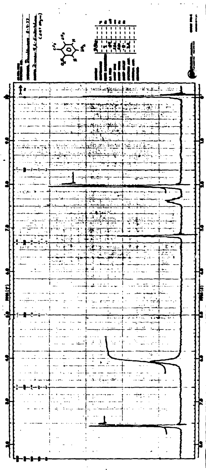
FIGURE 129 NMR SPECTRUM OF 2-AMINO-4,6-DINITROTOLUENE
