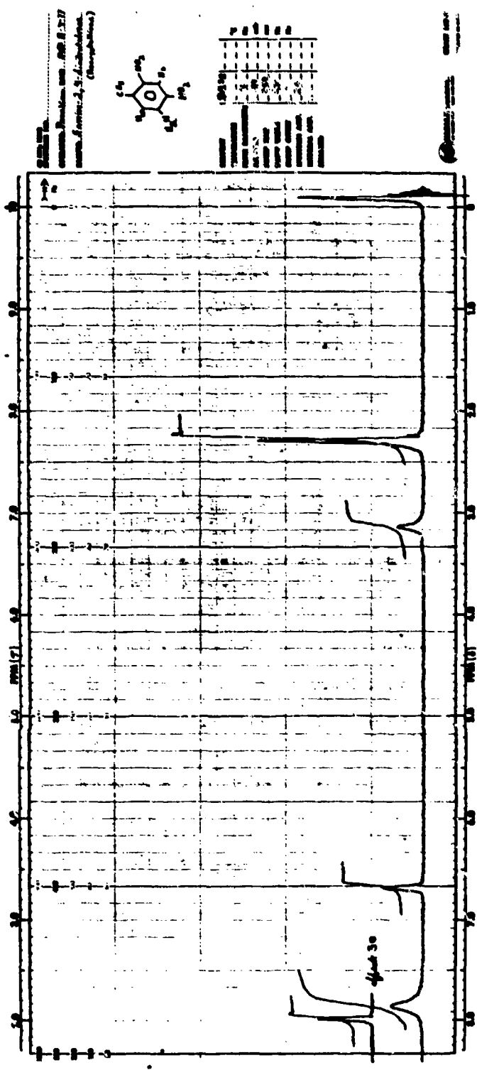
FIGURE 123 NMR SPECTRUM OF 5-AMINO-2,4-DINITROTOLUENE
