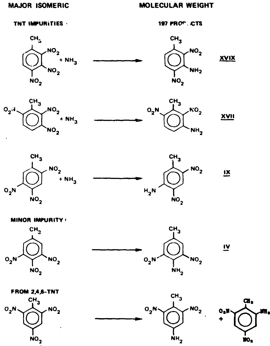
FIGURE 6 POSSIBLE ROUTE OF FORMATION OF AMINODINITROTOLUENES IN CONDENSATE WASTEWATER
