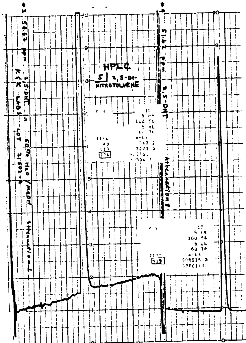
FIGURE 52 HPLC CHROMATOGRAM OF 2,5-DINITROTOLUENE
