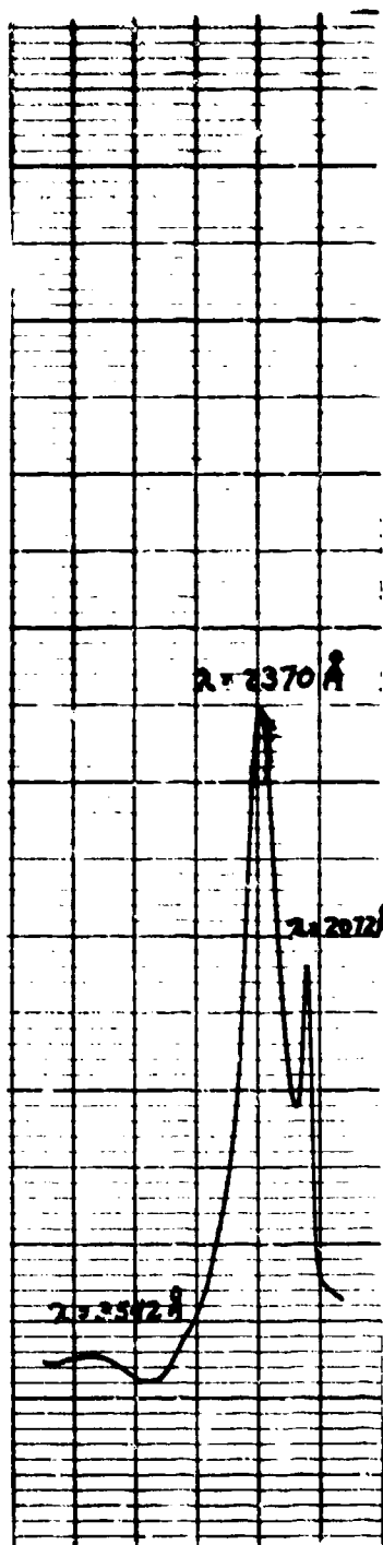
FIGURE 167 UV SPECTRUM OF 2-AMINO-6-NITROTOLUENE
