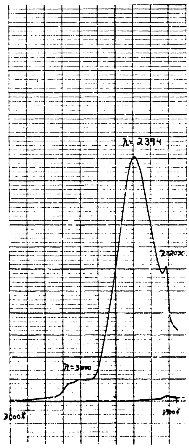
FIGURE 69 UV SPECTRUM OF 3,5-DINITROTOLUENE
