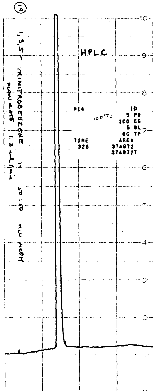
FIGURE 88 HPLC CHROMATOGRAM OF 1,3,5-TRINITROBENZENE
