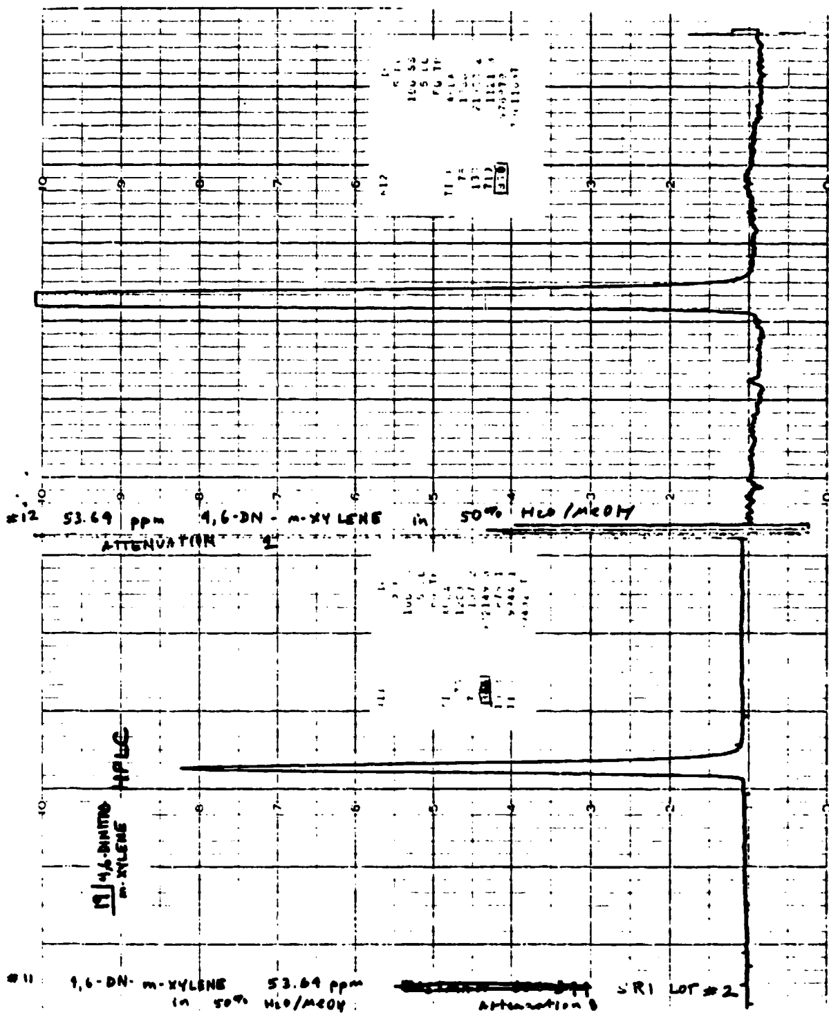
FIGURE 82 HPLC CHROMATOGRAM OF 4,6-DINITRO-m-XYLENE 8/21/82
