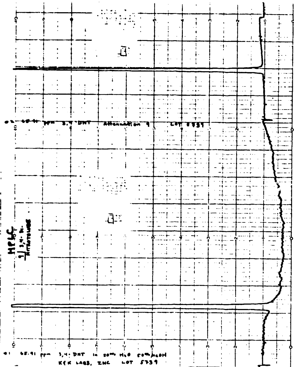
FIGURE 76 HPLC CHROMATOGRAM OF 3,4-DINITROTOLUENE
