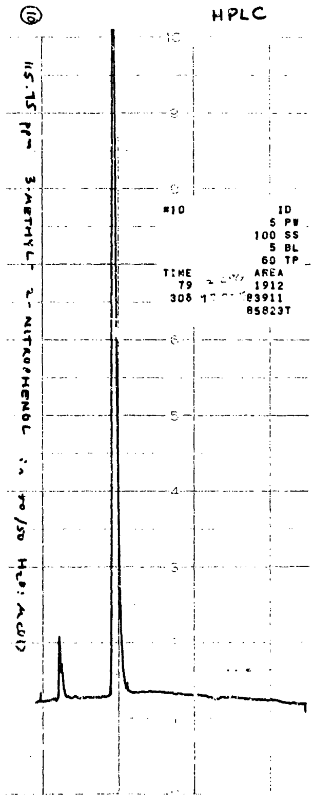
FIGURE 28 HPLC CHROMATOGRAM OF 3-METHYL-2-NITROPHENOL
