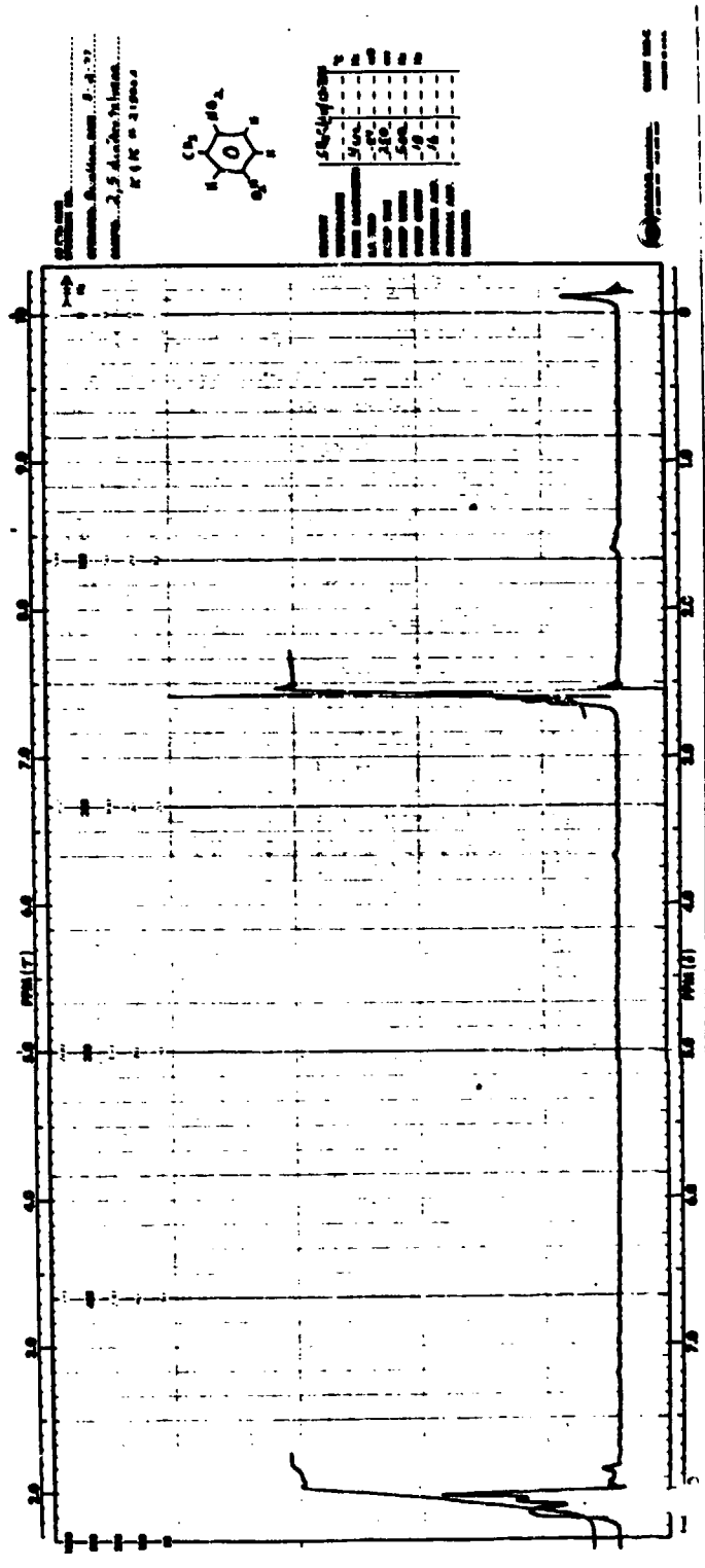
FIGURE 50 NMR SPECTRUM OF 2,5-DINITROTOLUENE
