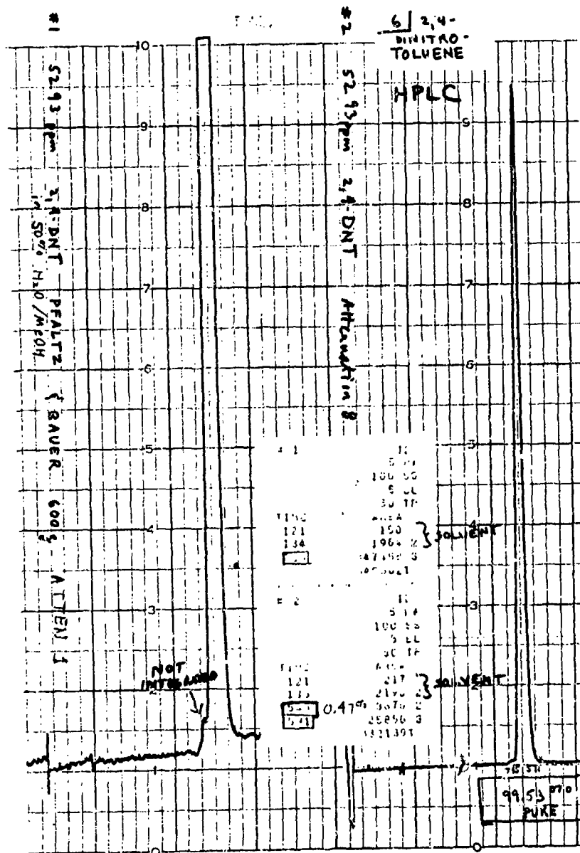
FIGURE 58 HPLC CHROMATOGRAM OF 2,4-DINITROTOLUENE
