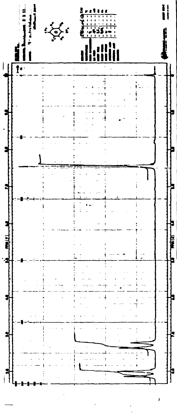
FIGURE 20 INFRARED SPECTRUM OF 4-NITROTOLUENE
