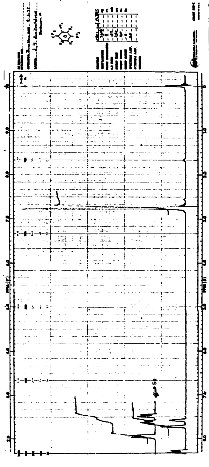
FIGURE 56 NMR SPECTRUM OF 2,4-DINITROTOLUENE
