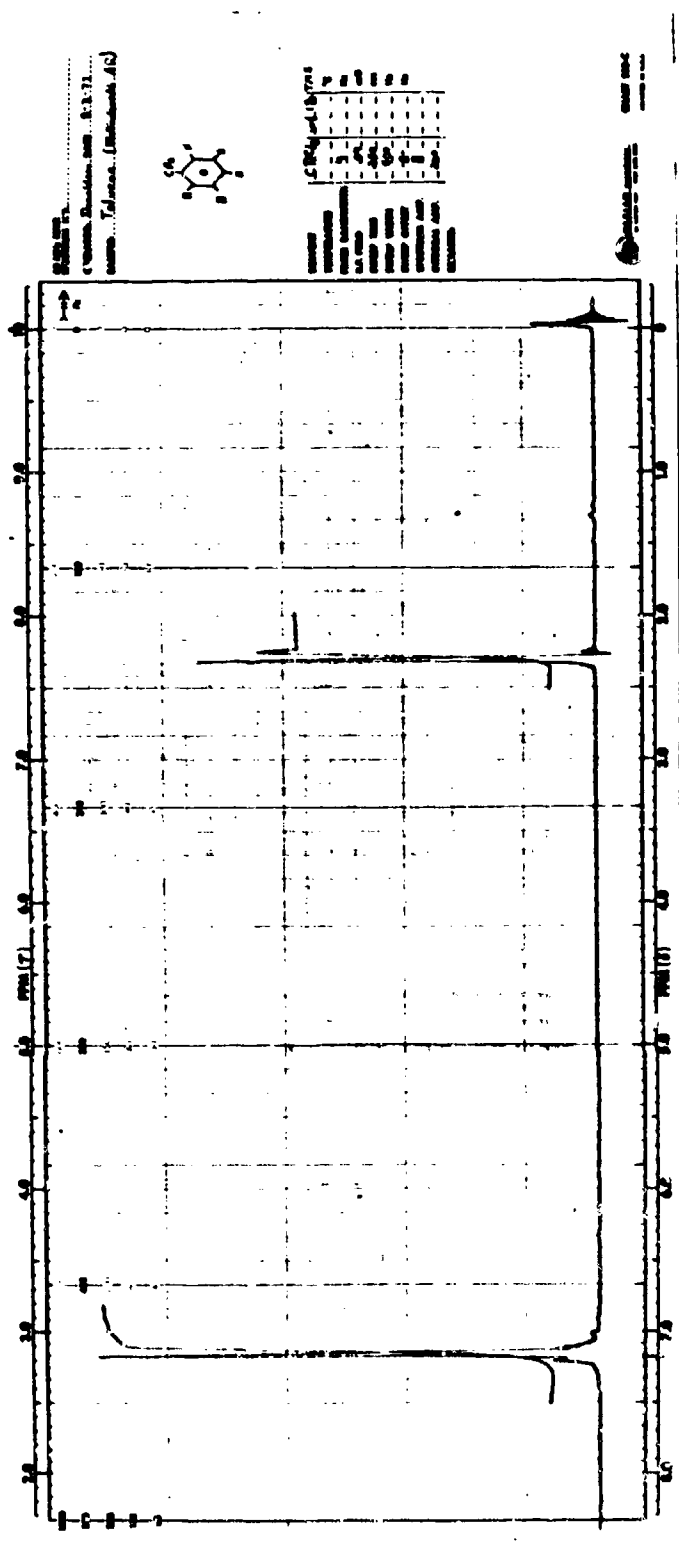
FIGURE 6 NMR SPECTRUM OF TOLUENE
