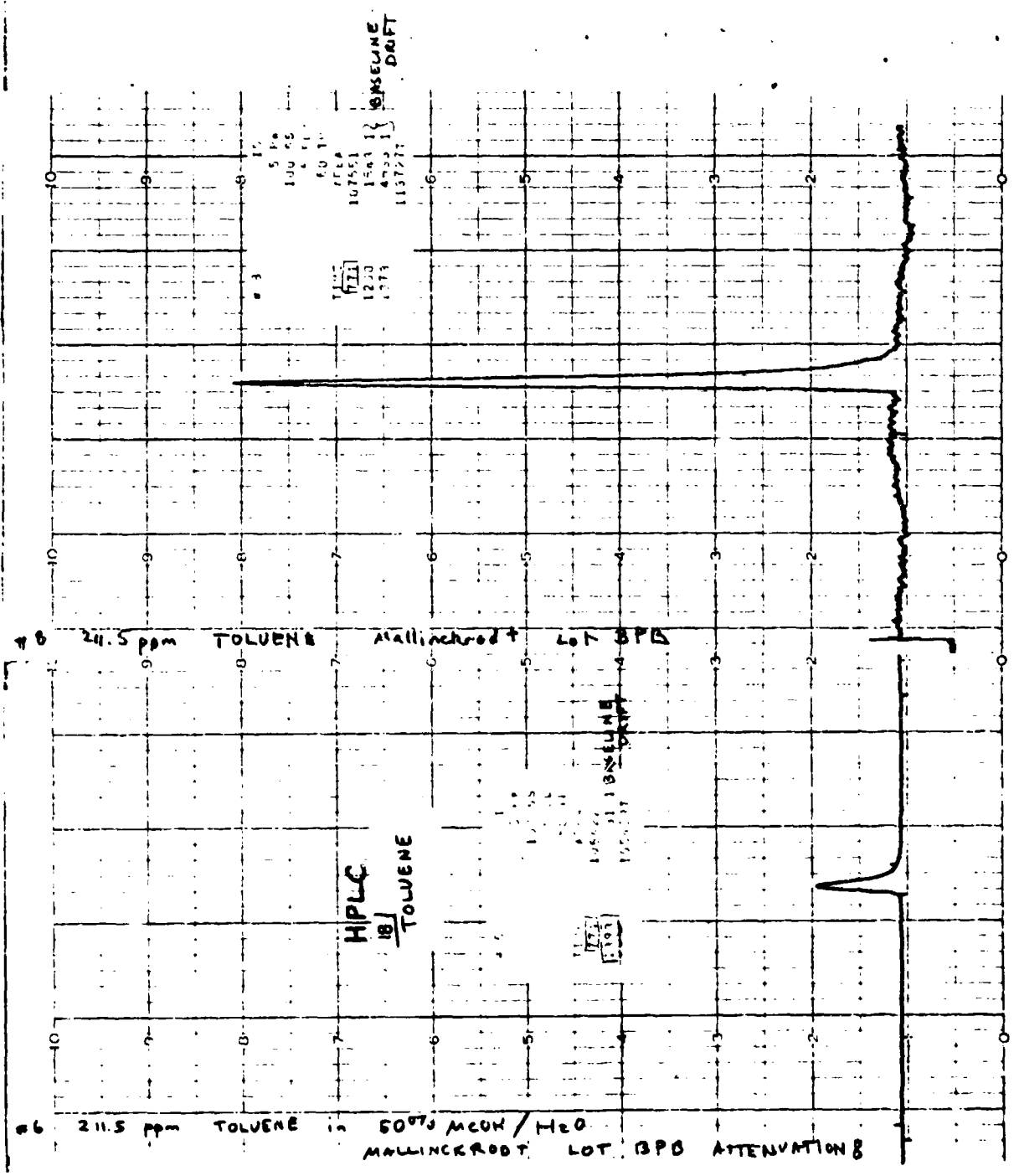
FIGURE 10 RPIC CHROMATOGRAM OF TOLUENE
