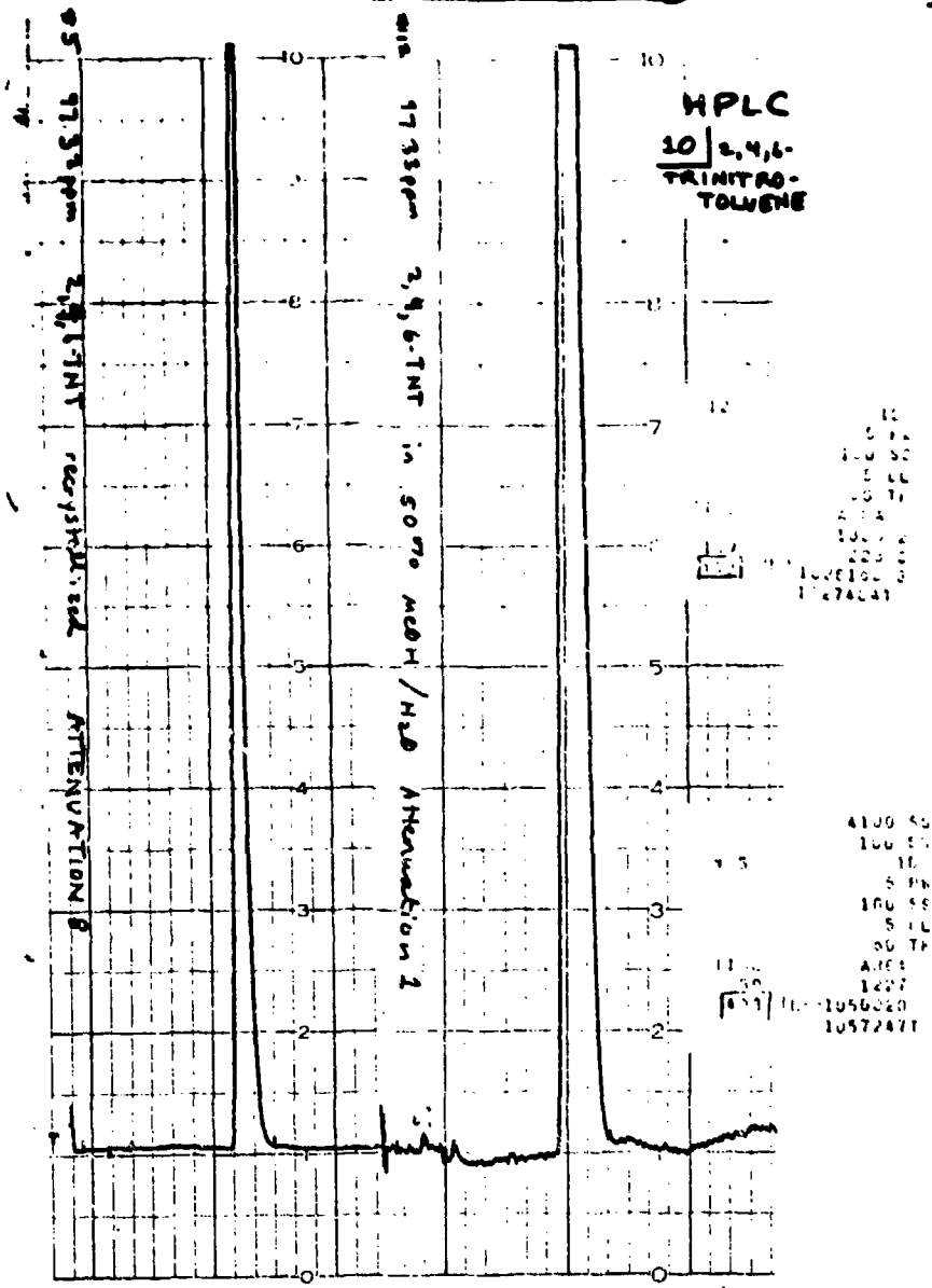
FIGURE 94 HPLC CHROMATOGRAM OF 2,4,6-TRINITROTOLUENE
