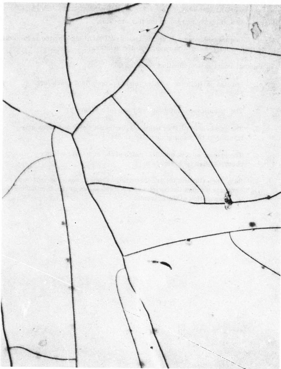
Figure 5. Microcracking of Panel No. 75 Modified 119 Coating with \text{SiO}_2 and Partially Hydrolyzed PVA on Stretched Plex 55 with Methyl Butynol/Ethanol/Polyvinyl Formal
