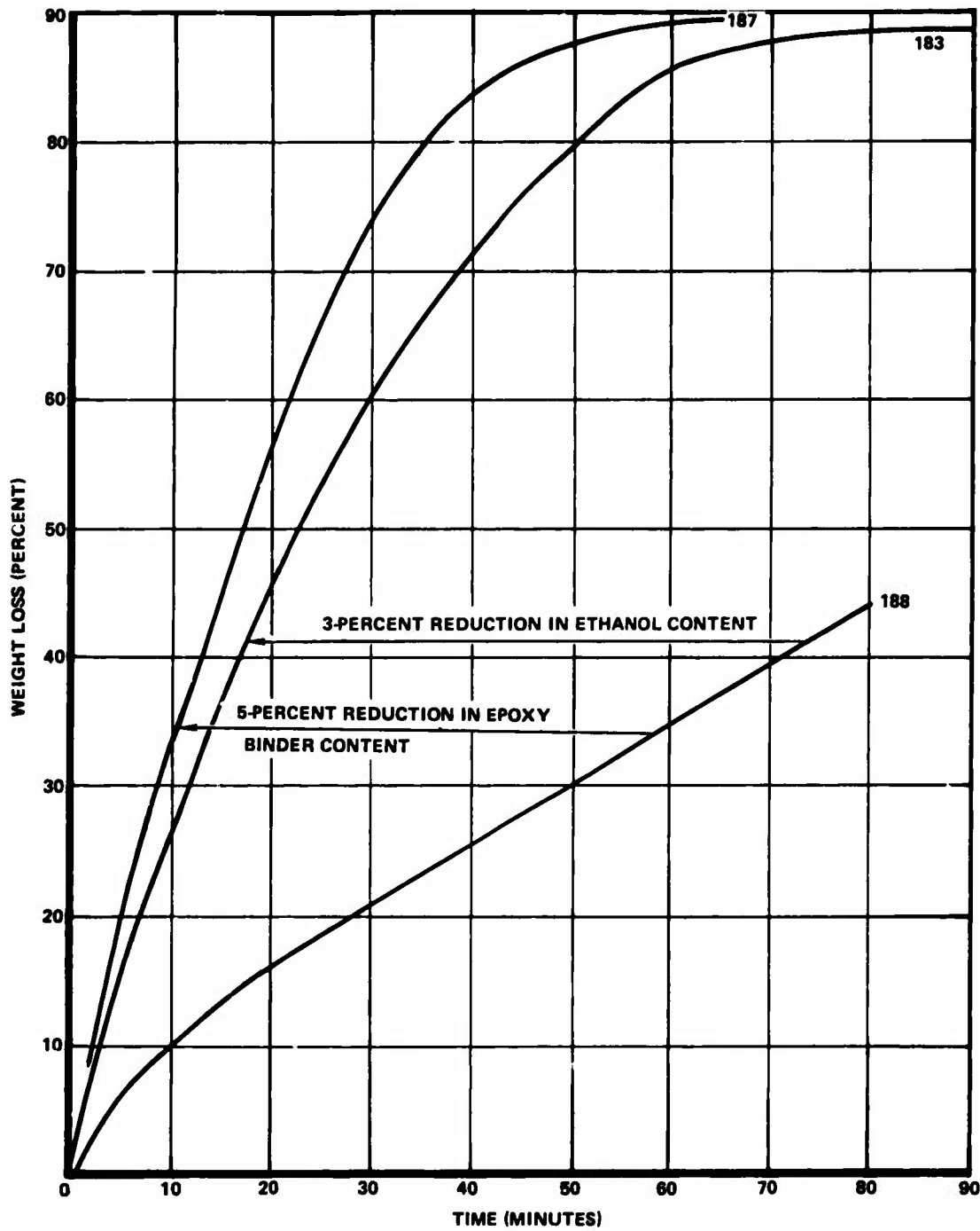
Figure C-1. Typical Evaporation Curves of Three Ratioed Mixes of the Same Constituents
