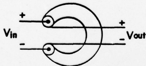
Fig. 1. Co-axial pulse transformer.
