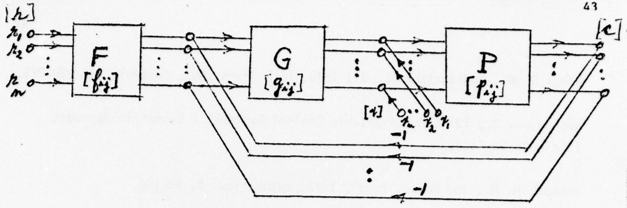
Fig. 1 Multiple input-output two matrix degree-of-freedom feedback structure c = Tr , T = [t_{ij}] , c = [c_1 \dots c_n]' , r = [r_1 \dots r_n]' .
