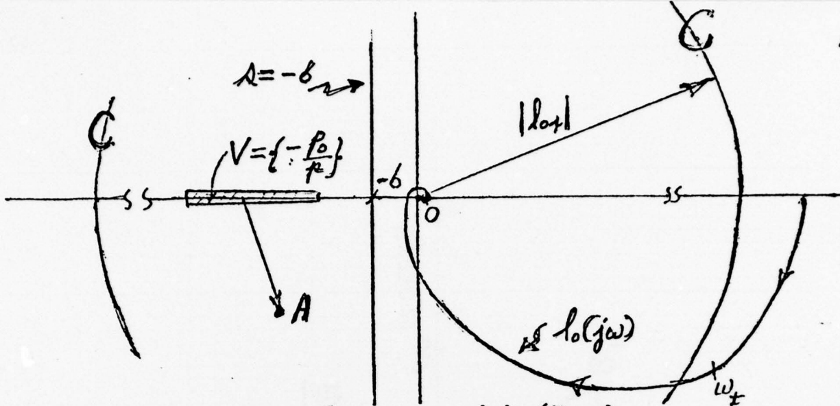
Fig. A1. Bounds on \epsilon_0 : C in [0, \omega_t] , \epsilon = -\delta in (\omega_t, \infty) ; and a satisfactory \epsilon_0(j\omega) .
