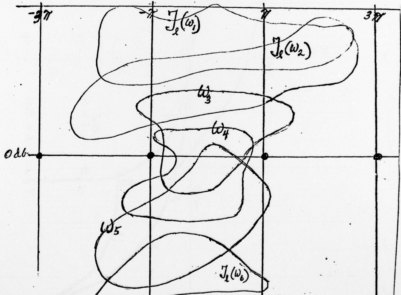
Fig. A2. The logarithmic complex plane (Nichols Chart) with templates of l(j\omega) : J_2(\omega) .
