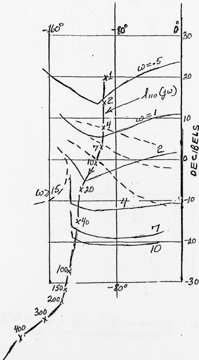
Fig. 7. Bounds on \alpha_{110}(j\omega) . Solid lines are due to |\gamma_{11}| , broken lines due to |\gamma_{12} d_{12e}|
