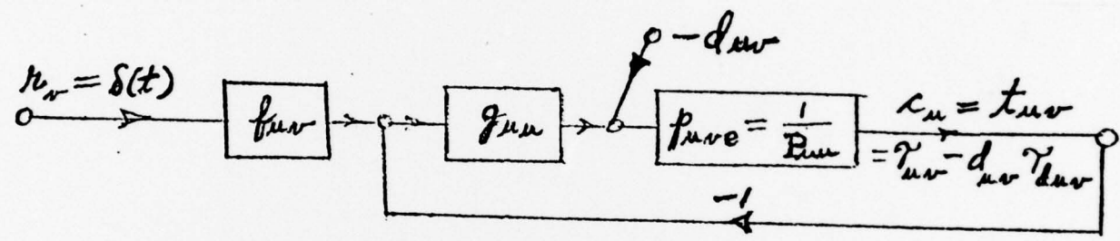
Fig. 2 Single-loop structure equivalent, for synthesis of t_{uv} ;
