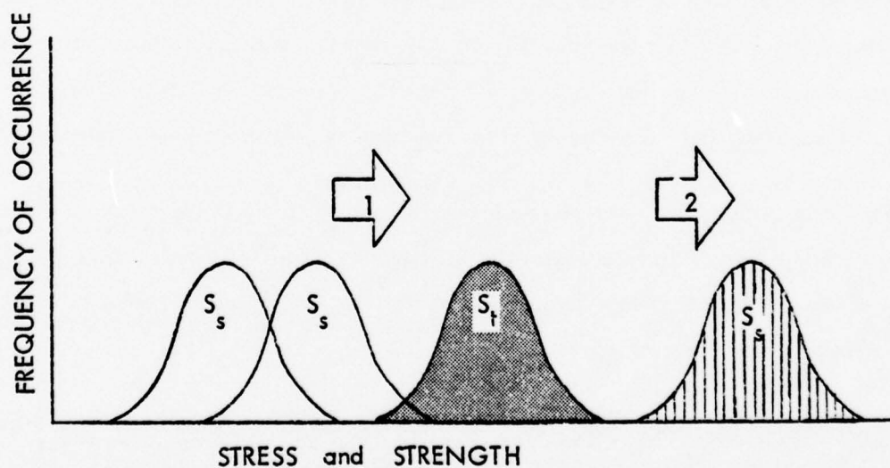
FIGURE 17. STRESS AND STRENGTH DENSITY FUNCTIONS WHERE STRESS EXCEEDS STRENGTH
