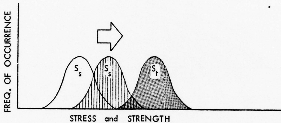
FIGURE 16. STRESS AND STRENGTH DENSITY FUNCTIONS UNDER CONDITIONS OF INCREASING STRESS
