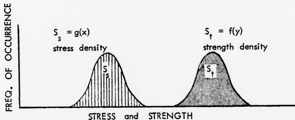
FIGURE 15 , STRESS AND STRENGTH DENSITY FUNCTIONS UNDER NORMAL STRESS CONDITIONS
