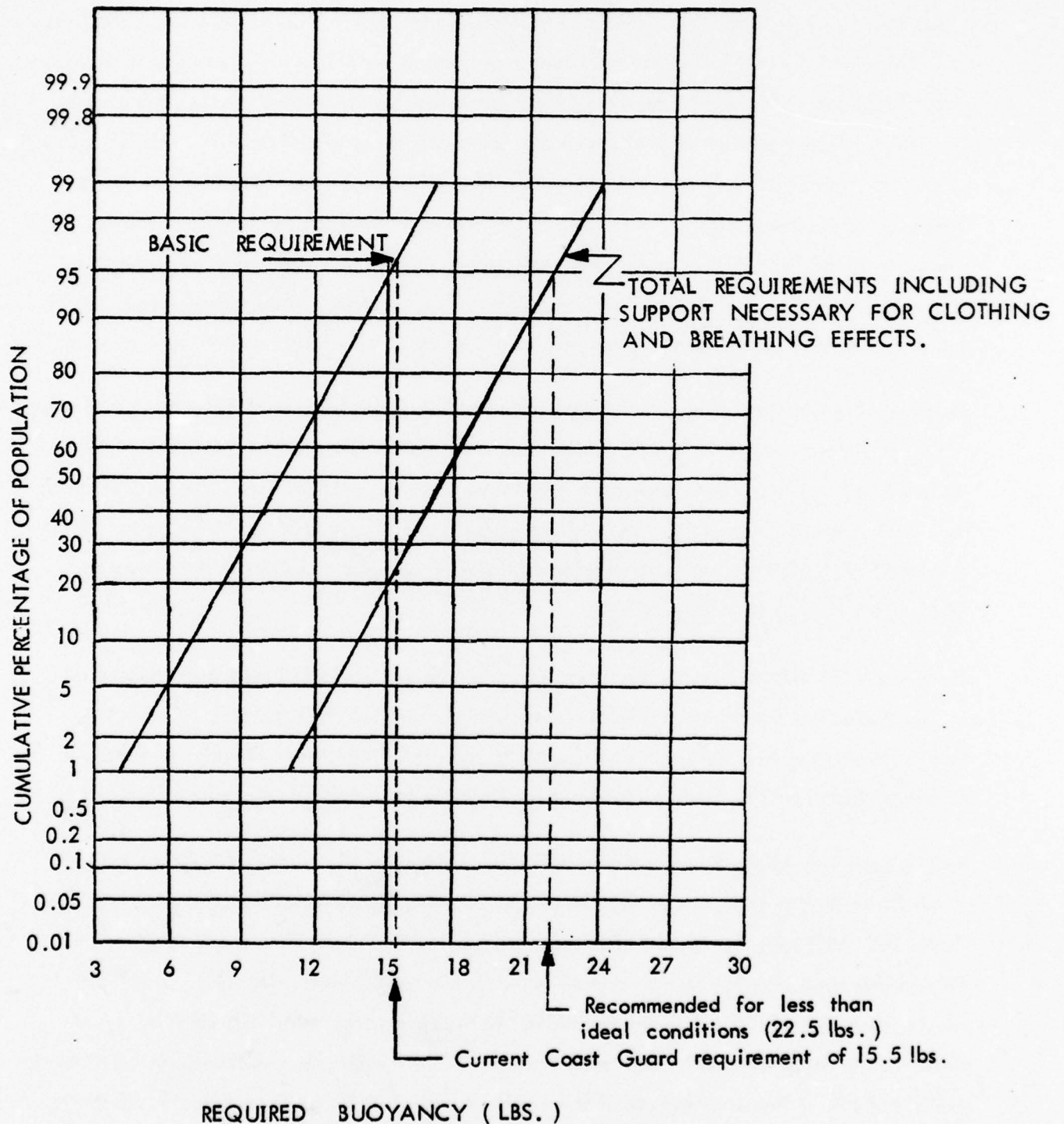
FIGURE 2. BUOYANCY REQUIREMENTS FOR PFD RELIABILITY
