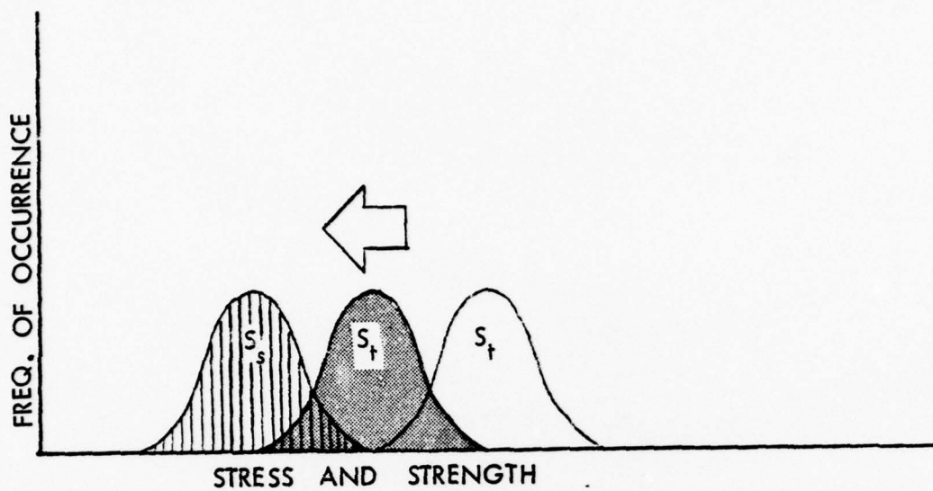
FIGURE 18. STRESS AND STRENGTH DENSITY FUNCTIONS WHERE STRENGTH IS DEGRADING
