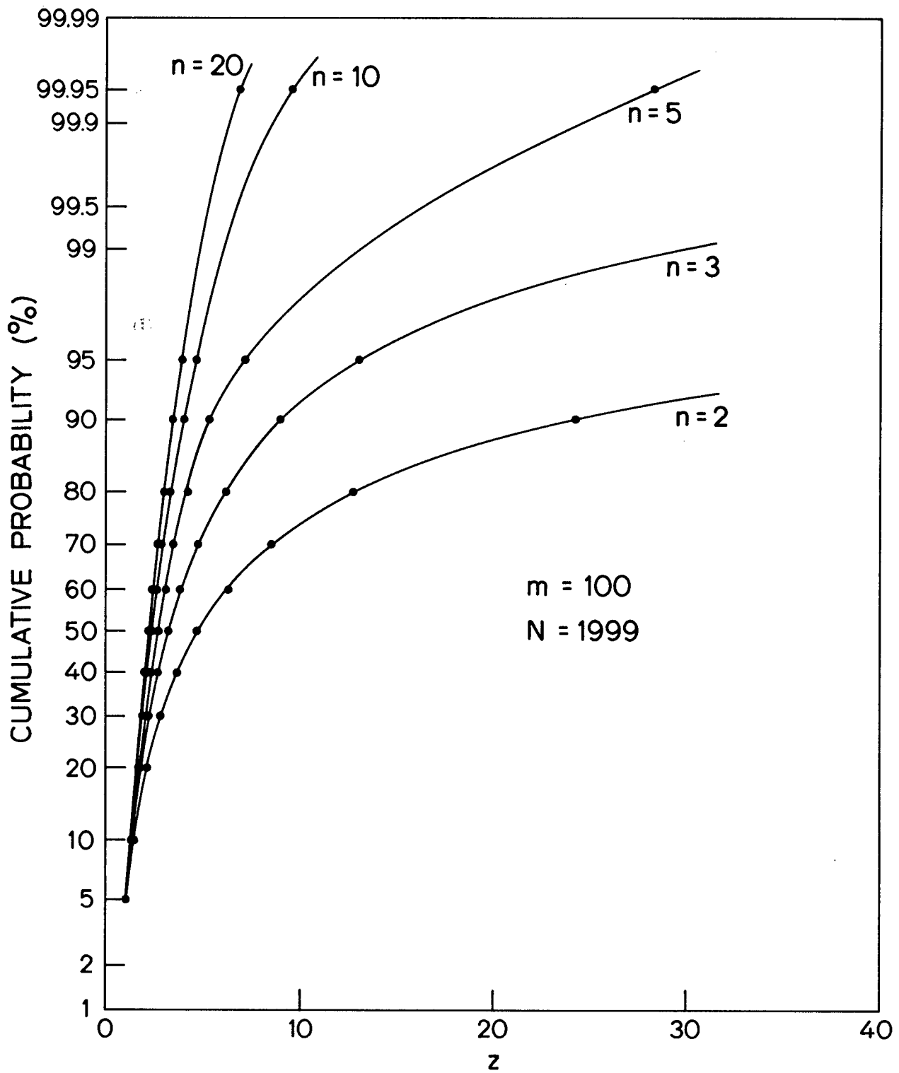
Fig. 29. Empirical distribution of Z (m=100)
