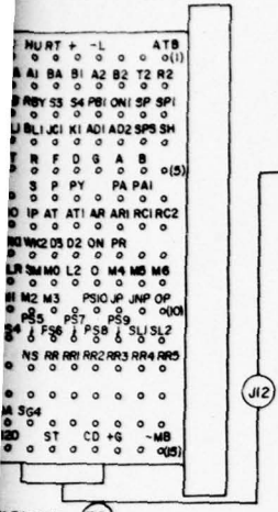
FIGURE 3D TERMINAL BLOCK (10 X 15) (FIG. 2A, H-75650-A) (NOTES 201 & 203)
