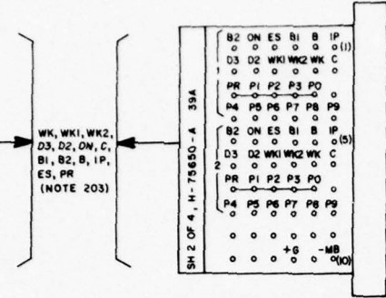
FIGURE 3E TERMINAL BLOCK (6 X 10) (FIG. 2A, H-75650-A) (NOTES 201 & 203)
