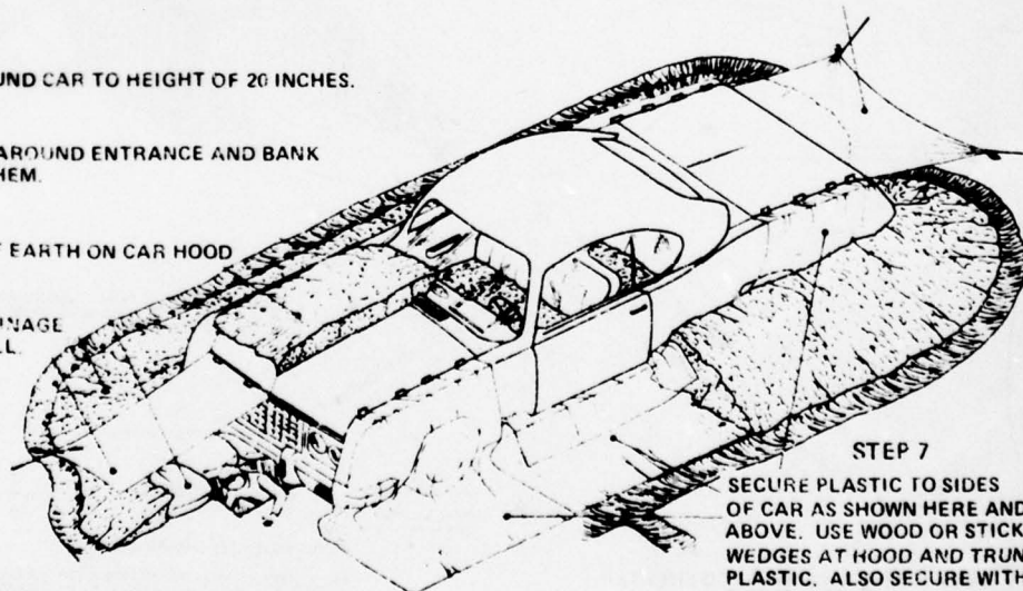
TRENCH AND ENTRYWAY DETAIL
