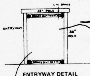
ENTRYWAY DETAIL
