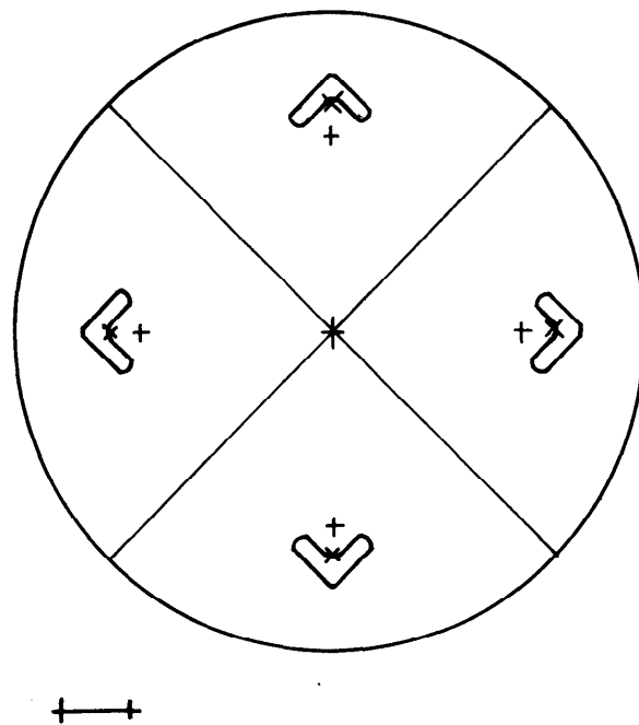
FIGURE 11. FULL DIE LAYOUT BY REPEATING SINGLE SEGMENT ARRANGEMENT FROM FIGURE 10
