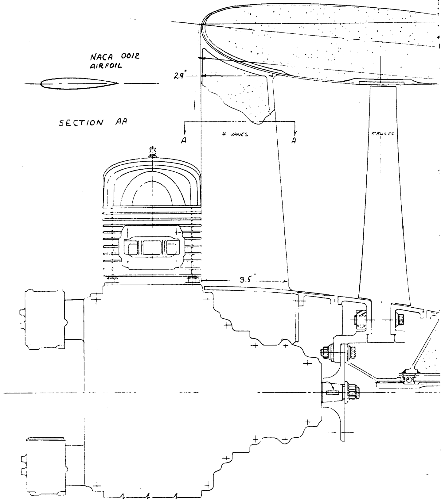
Figure 18. Conceptual Design of a Ducted Propeller Installation for Advanced RPV With 5860 RPM Engine.
