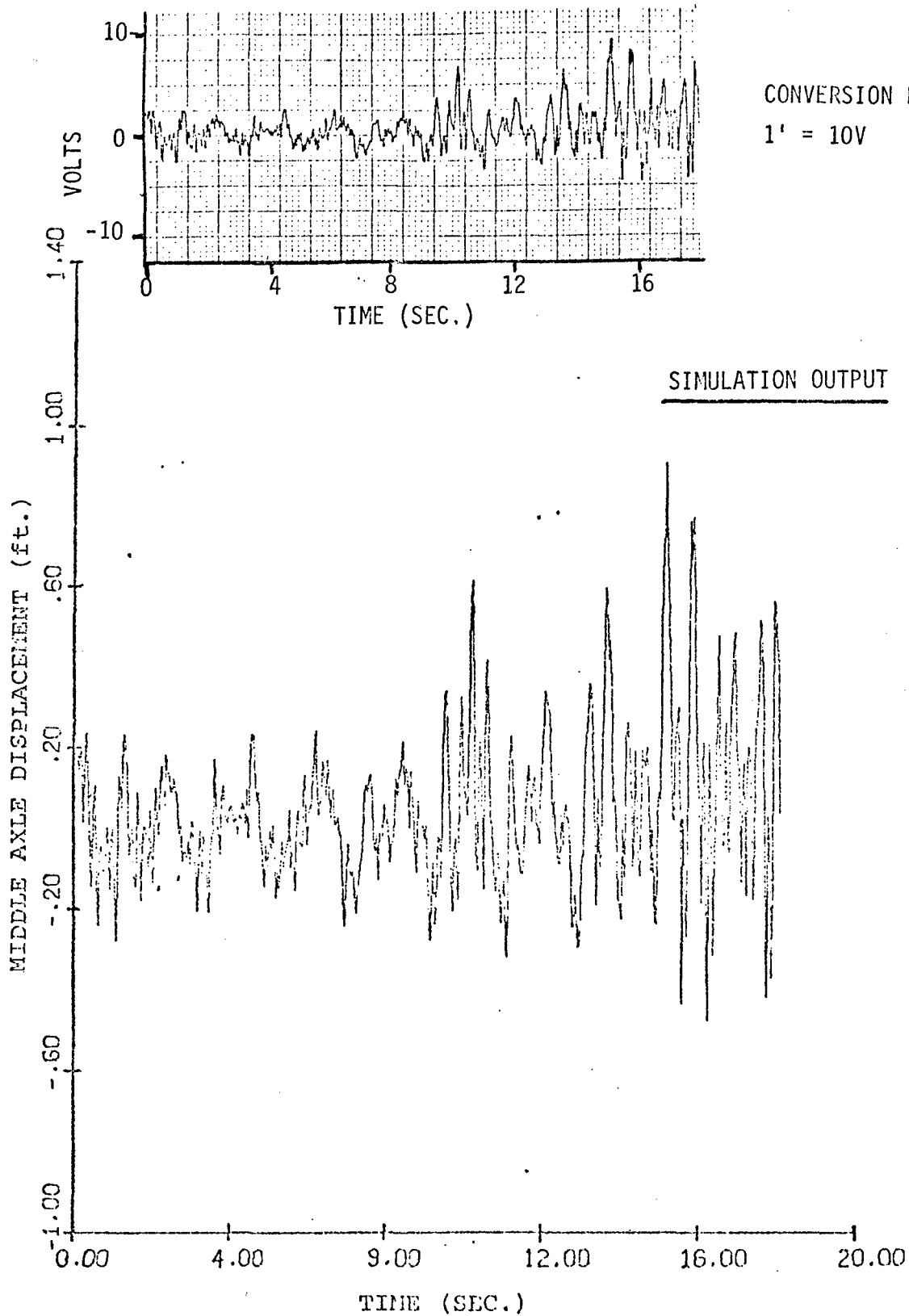
Figure 13. Comparison of the Simulation and the Controller Outputs for the Middle Axle Displacement
