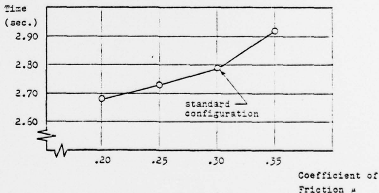
Figure 12 Influence of Coefficient of Friction of Coupled Motion on Fuze Delay Time
