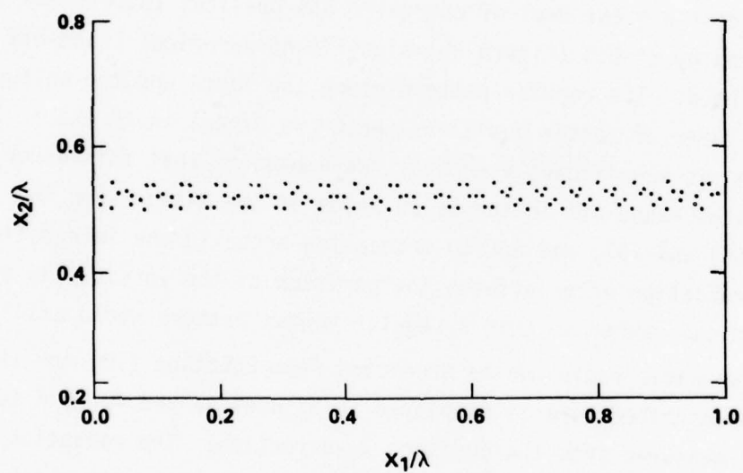
Figure 3 - Position of Vortices in Shear Layer With No Applied Disturbance (At t^*=0.0 , vortices are arranged in columns, seven per column)
