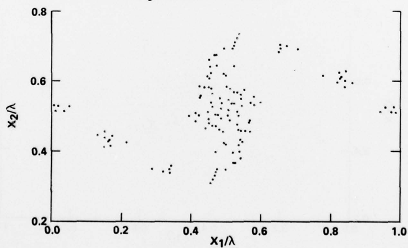
Figure 6 - Position of Vortices in Shear Layer Resulting From a Single-Wave Disturbance (At t^*=0.0 , vortices are arranged in columns, 4 vortices per column and 3 vortices per column)
