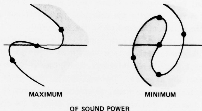
Figure 8 - The Point Vortices Closest to the Center of a Rolling-up Discontinuity Sheet Generate Most of the Sound. The Shaded Area Represents the Upper Side of an Initially Horizontal Discontinuity Sheet. (From H.J. Lugt)
