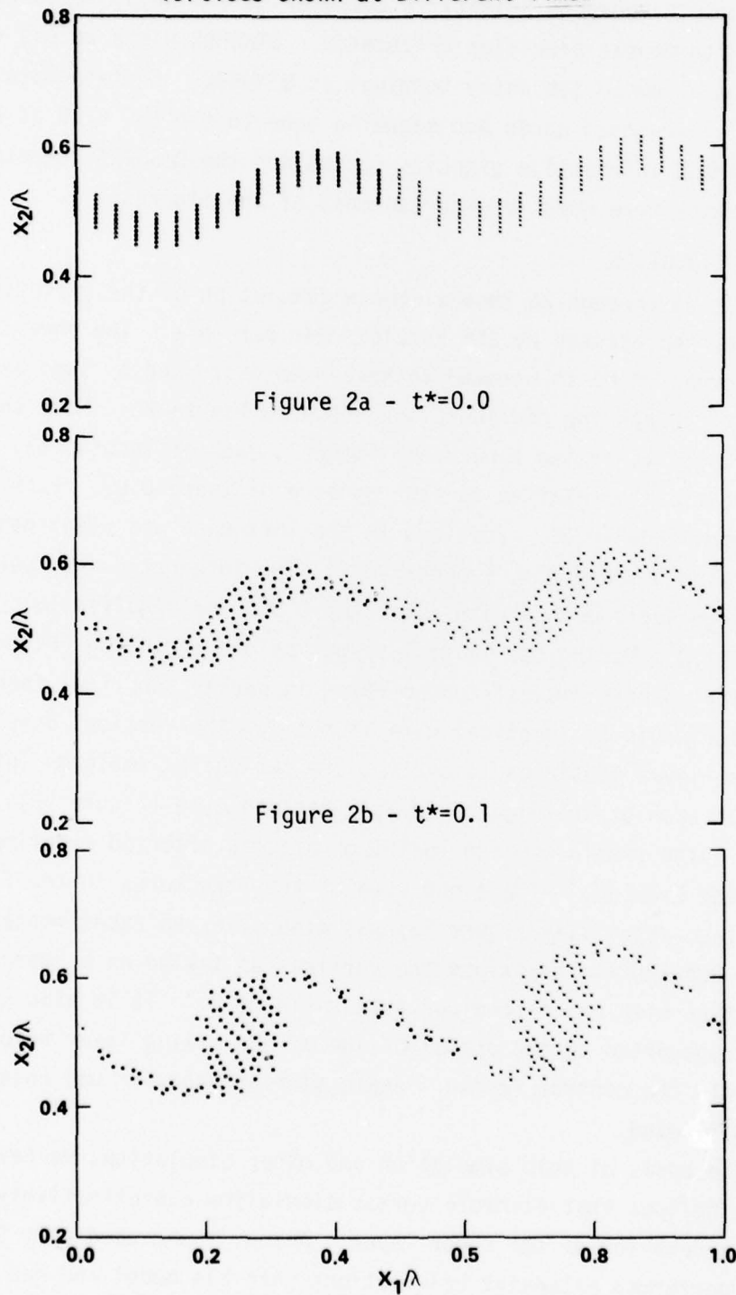
Figure 2 - Evolution of a Shear Layer Represented by Discrete Vortices Shown at Different Times
