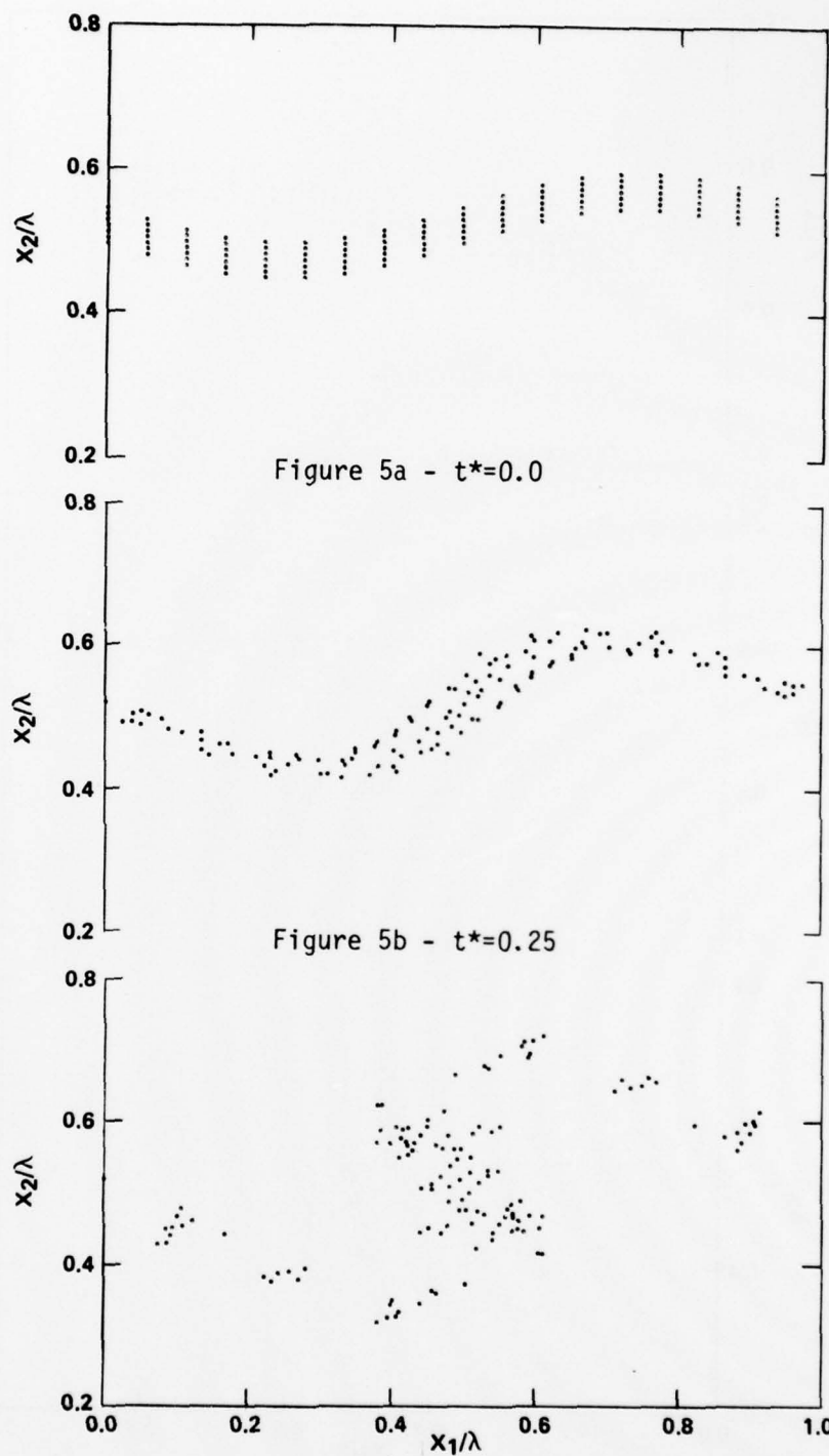
Figure 5 - Position of Vortices in Shear Layer Resulting From a Single-Wave Disturbance (At t^*=0.0 , vortices are arranged in columns, seven per column)
