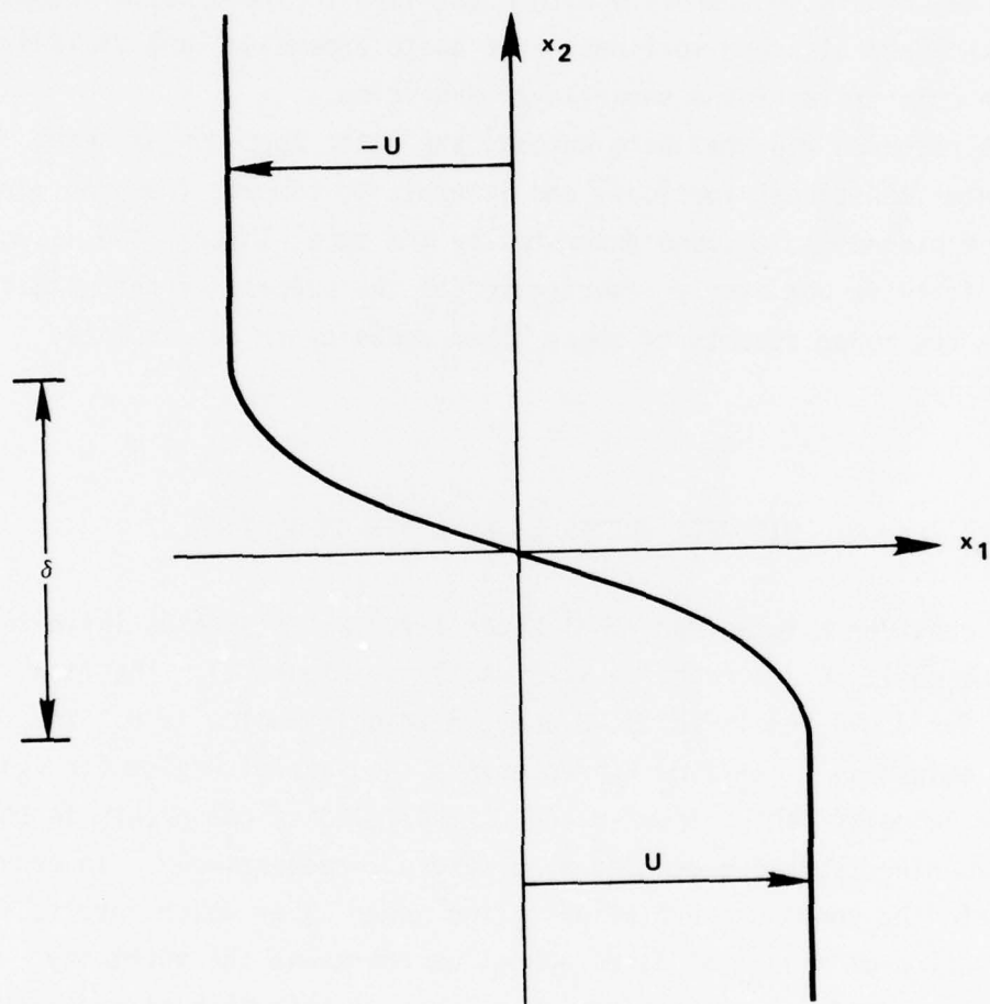
Figure 1 - Shear-Layer Geometry
