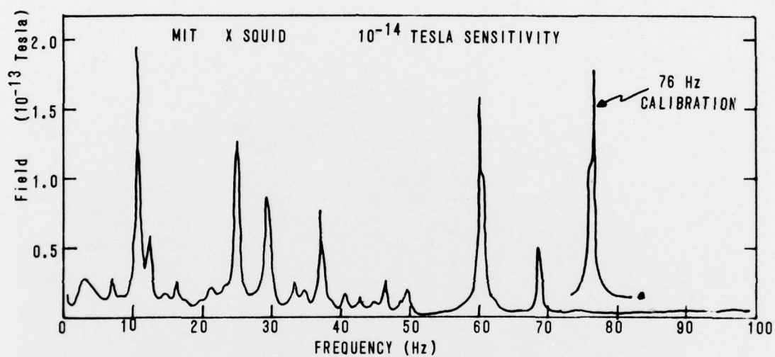
Fig. 6 — A typical noise spectrum obtained with the SQUID along one direction in the MIT shielded room. Data were tape recorded at MIT and spectrum analyzed at NRL. Magnetic field is plotted versus frequency.
