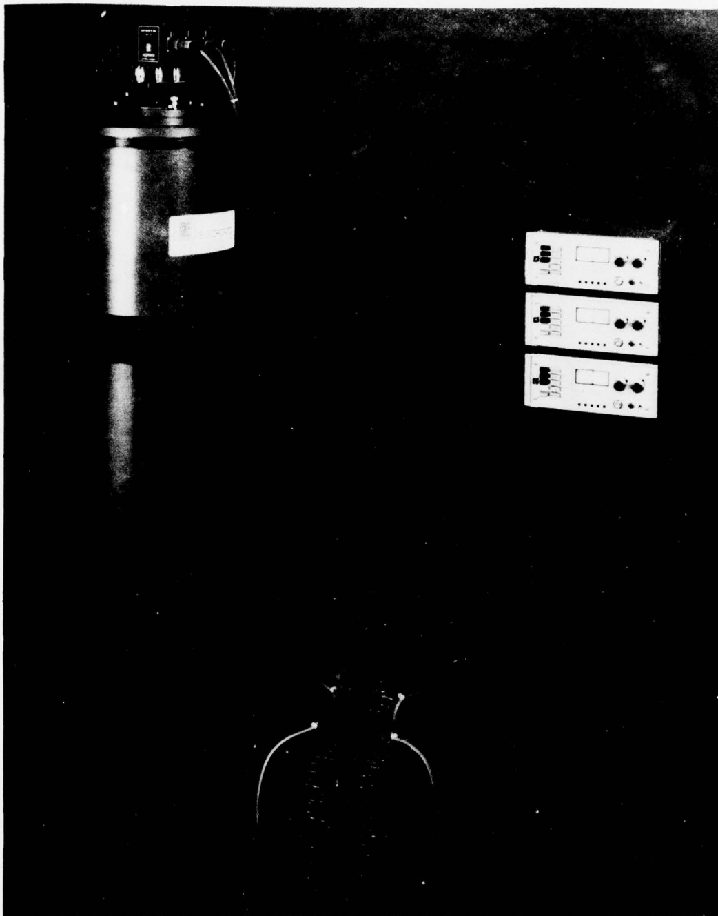
Fig. 1 — This figure is a photograph of the Triaxial SQUID Magnetometer that was tested. At the left is the cylindrical liquid helium dewar in which the magnetometer is mounted. The boxes on the right are the electronics.
