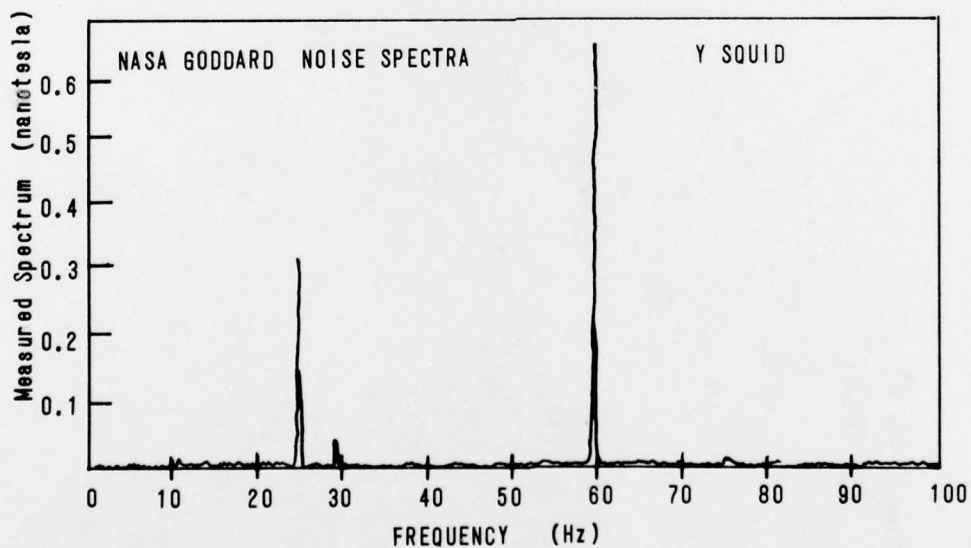
Fig. 4 — A typical noise spectrum along one axis of the Goddard facility. Tape recorded data was analyzed using a spectrum analyzer whose output in magnetic field units was plotted versus frequency.
