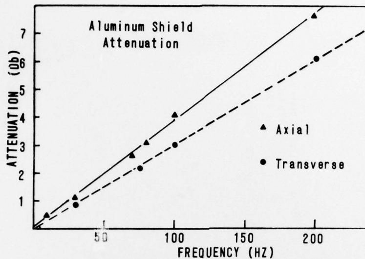
Fig. 3 — Attenuation versus frequency for the cylindrical aluminum shield. Triangles are the data for the field along the axis of the shield for perpendicular fields.
