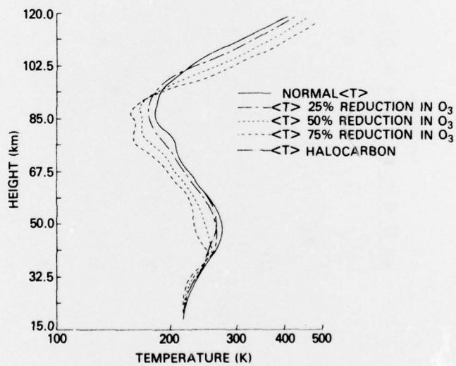
Fig. 2 - The globally averaged temperature in K
