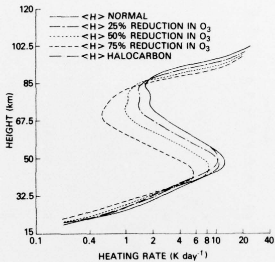
Fig. 1 - The globally averaged heating rate in \text{K day}^{-1}
