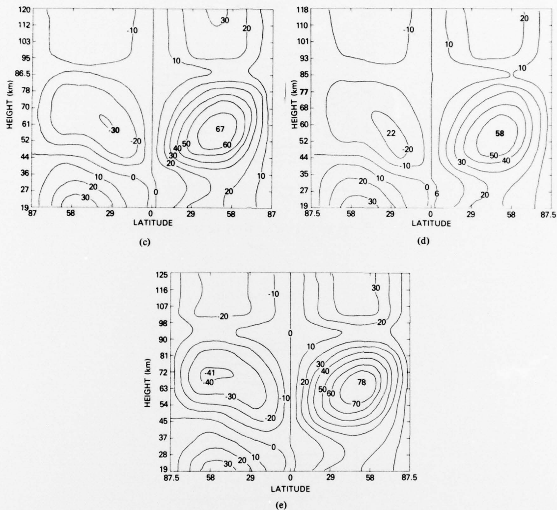
Fig. 3 (Continued) – The steady state mean zonal wide structure of the upper atmosphere in \text{ms}^{-1} . Part a is the "normal" structure. Parts b , c , and d show the structure for 25%, 50%, and 75% reduction in the ozone mixing ratio, respectively. Part e shows the results for the halocarbon case.
