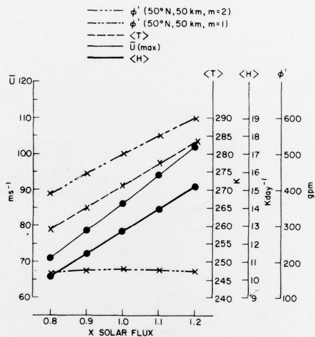
Fig. 5 - The response of the stratosphere and mesosphere to solar flux changes. \langle T \rangle is the stratopause temperature, \langle H \rangle is the maximum stratospheric heating rate, \bar{u} gives the maximum polar night jet strength, and \phi' is the geopotential height associated with planetary wave numbers one and two at 50 km and 50°N.
