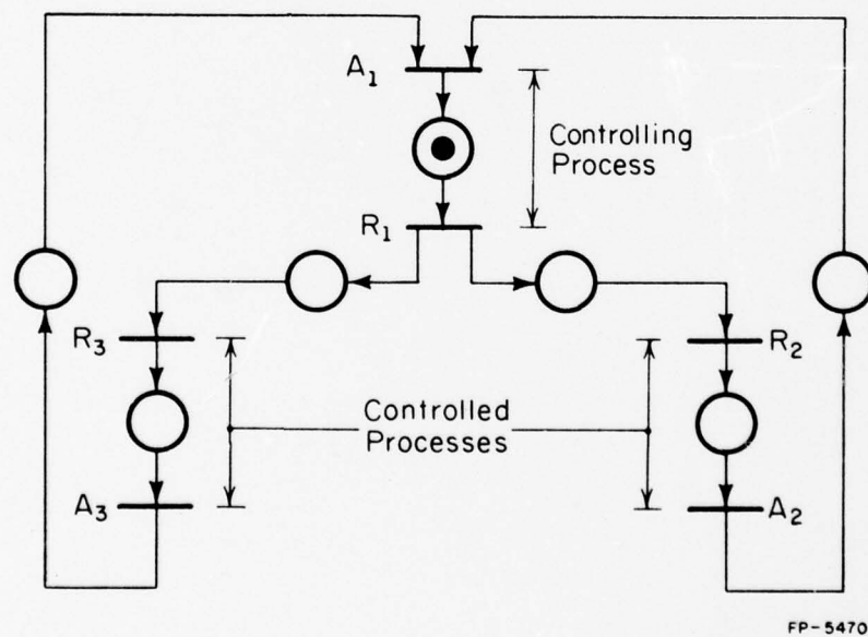
Figure 2.5. The Wye Module.
