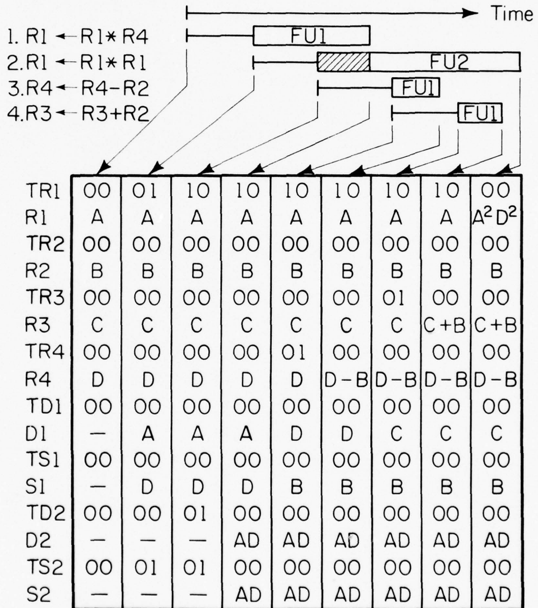
Figure 5.2. Illustration of the Forwarding Algorithm.
