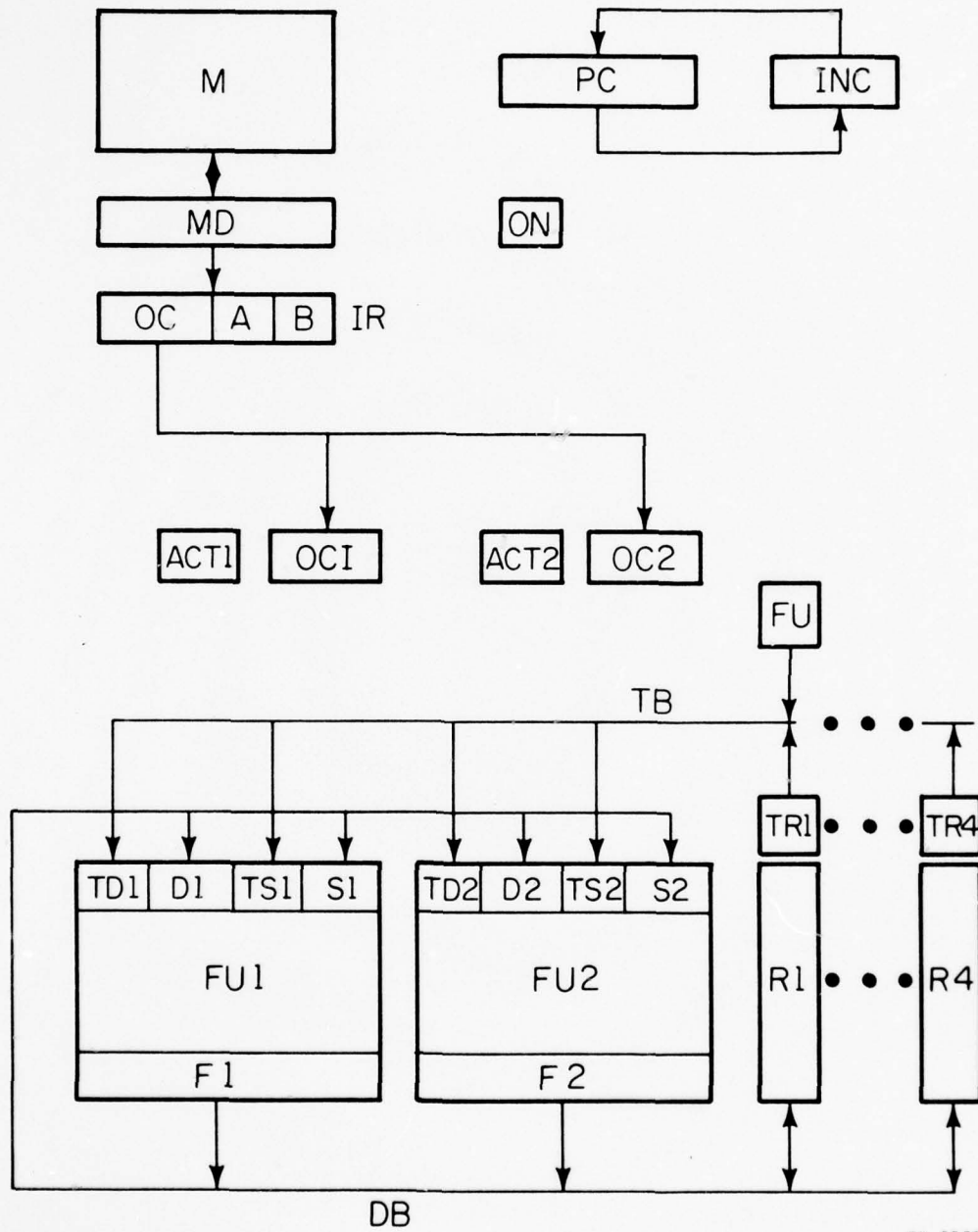
Figure 5.1. The DS of the Example Design.
