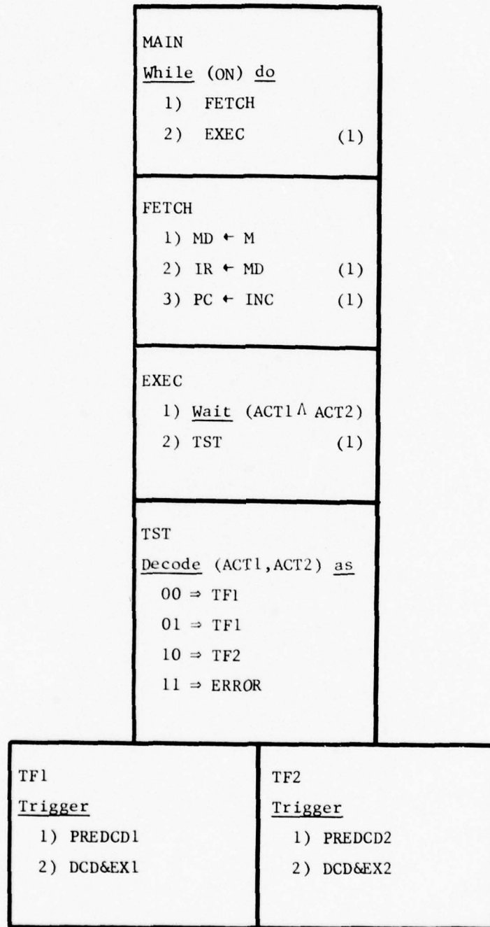
Figure 5.3(a). The Example Design.
