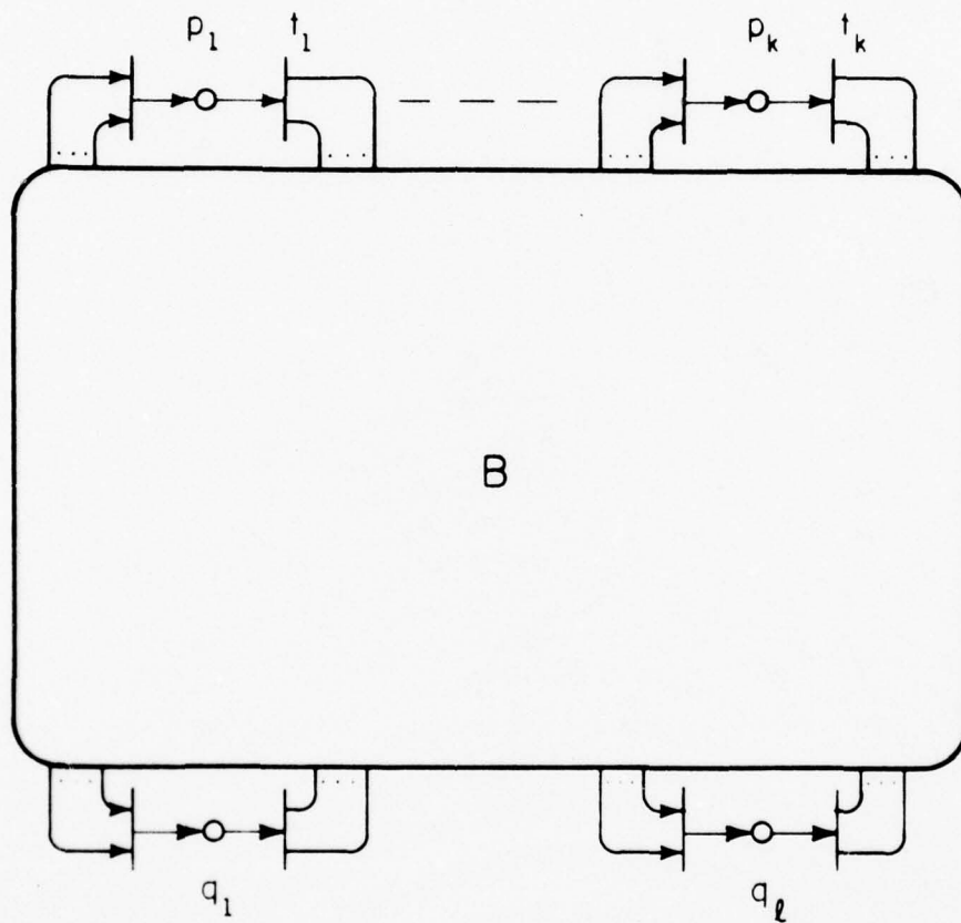
Figure 7.1. A CHDL Block's PN.
