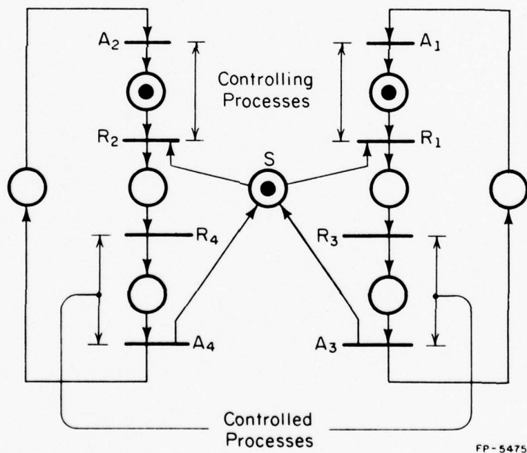
Figure 2.10. The Mutual Exclusion Module.
