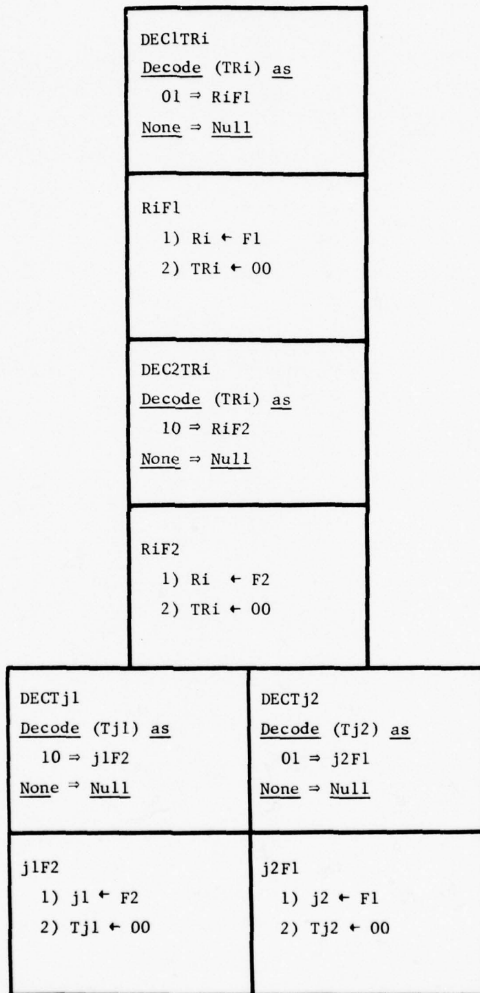
Figure 5.3(e). The Example Design.
