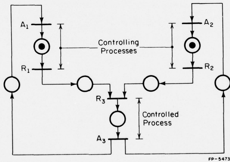
Figure 2.8. The Junction Module.
