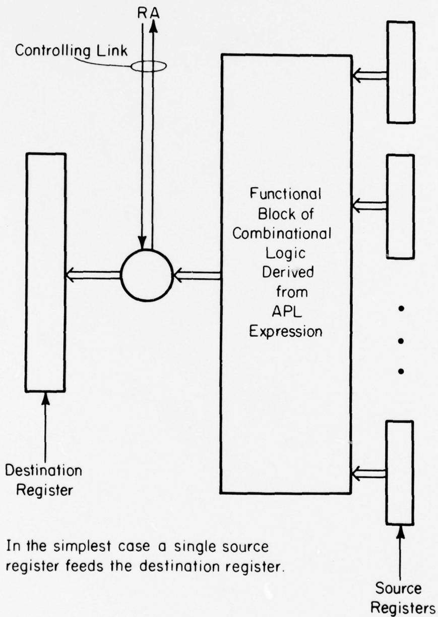
Figure 1.2. Register-transfer Logic.
