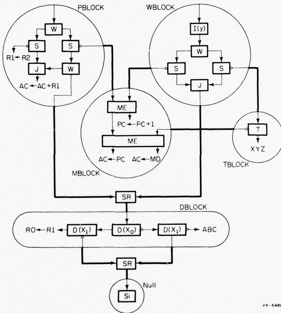
Figure 4.7. Inter Block Connections.
