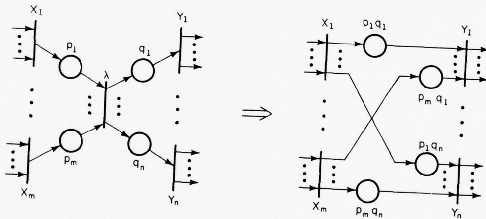
Simplification 2
