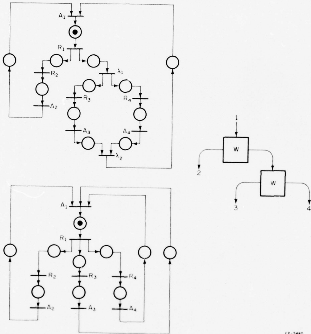
Figure 2.15. Construction 2.1 (case 1).
