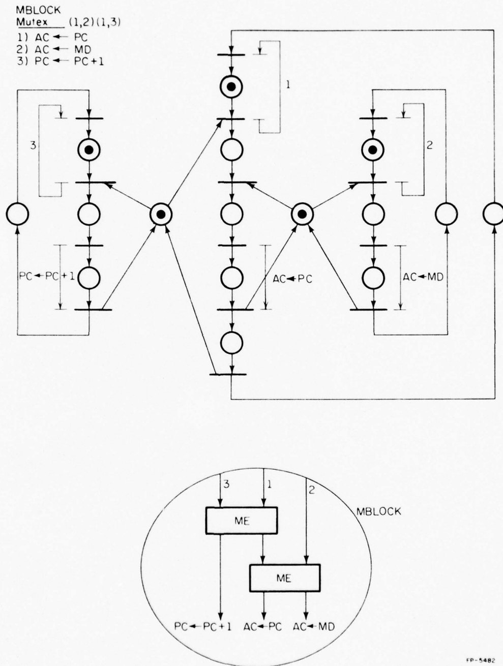
Figure 4.3. An Example Mutual Exclusion Process Block.
