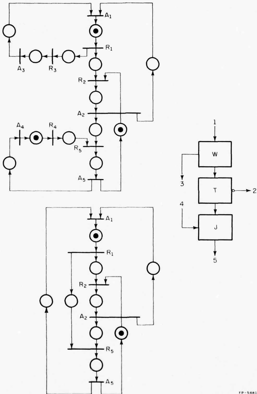
Figure 2.16. Construction 2.1 (case 2).
