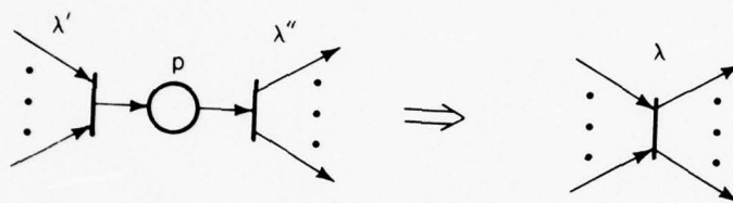
Simplification 1
