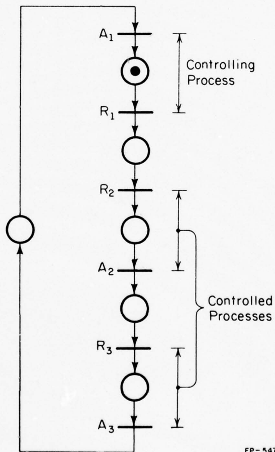
Figure 2.6. The Sequence Module.
