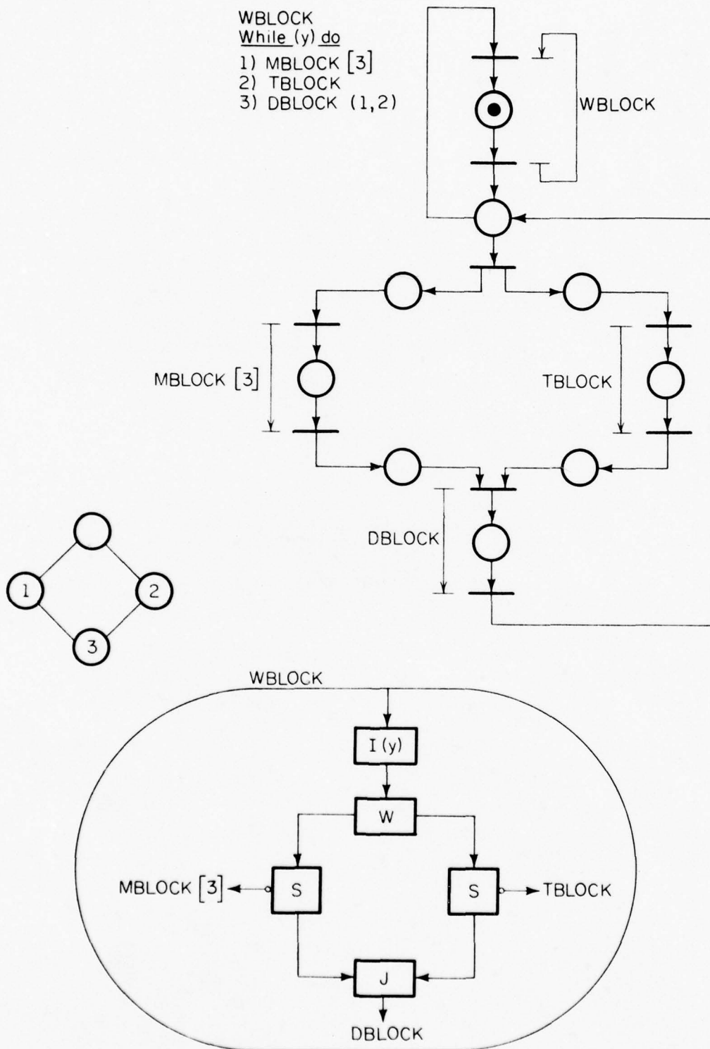
Figure 4.6. An Example While Process Block.
