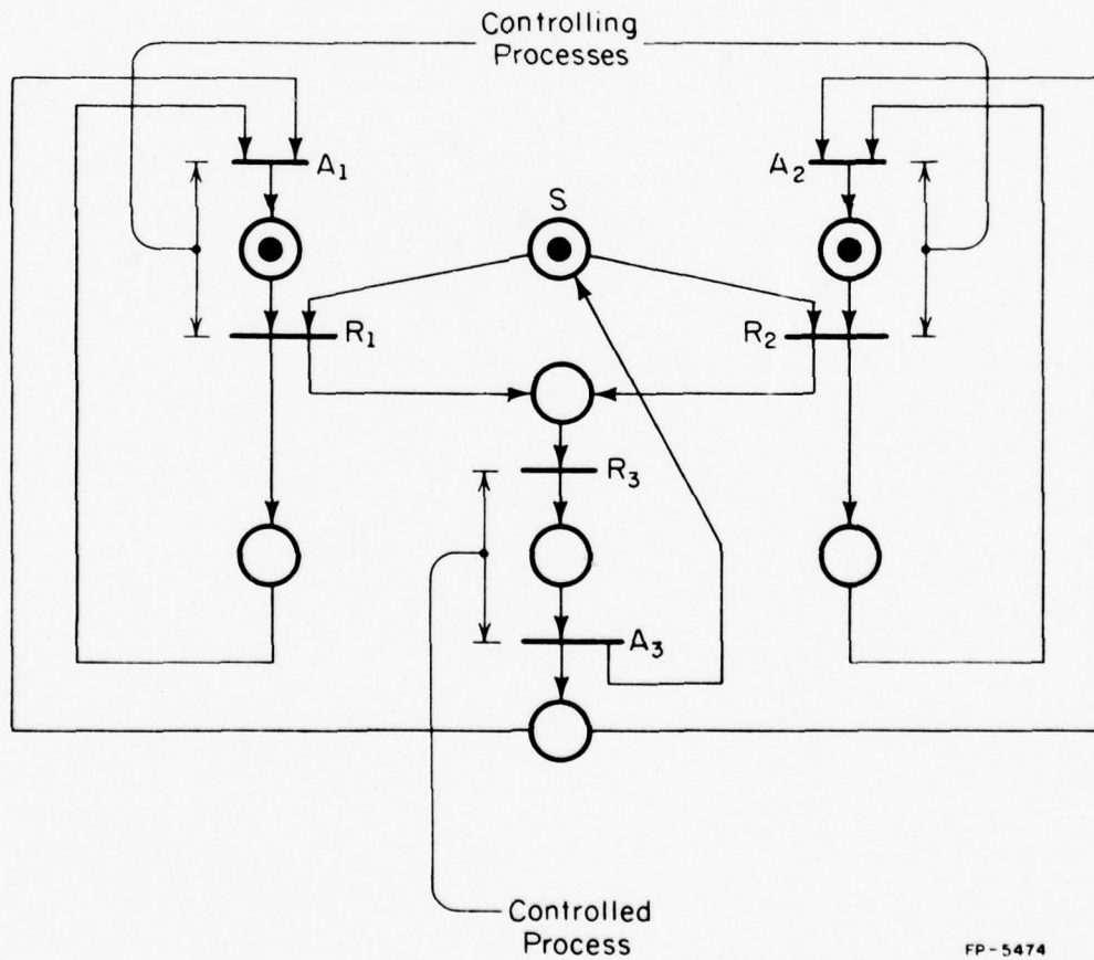
Figure 2.9. The Shared Resource Module.
