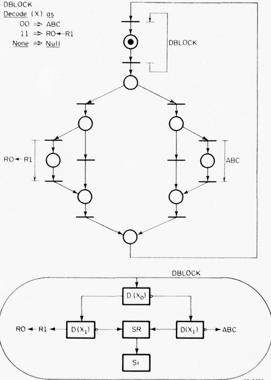
Figure 4.2. An Example Decode Process Block.
