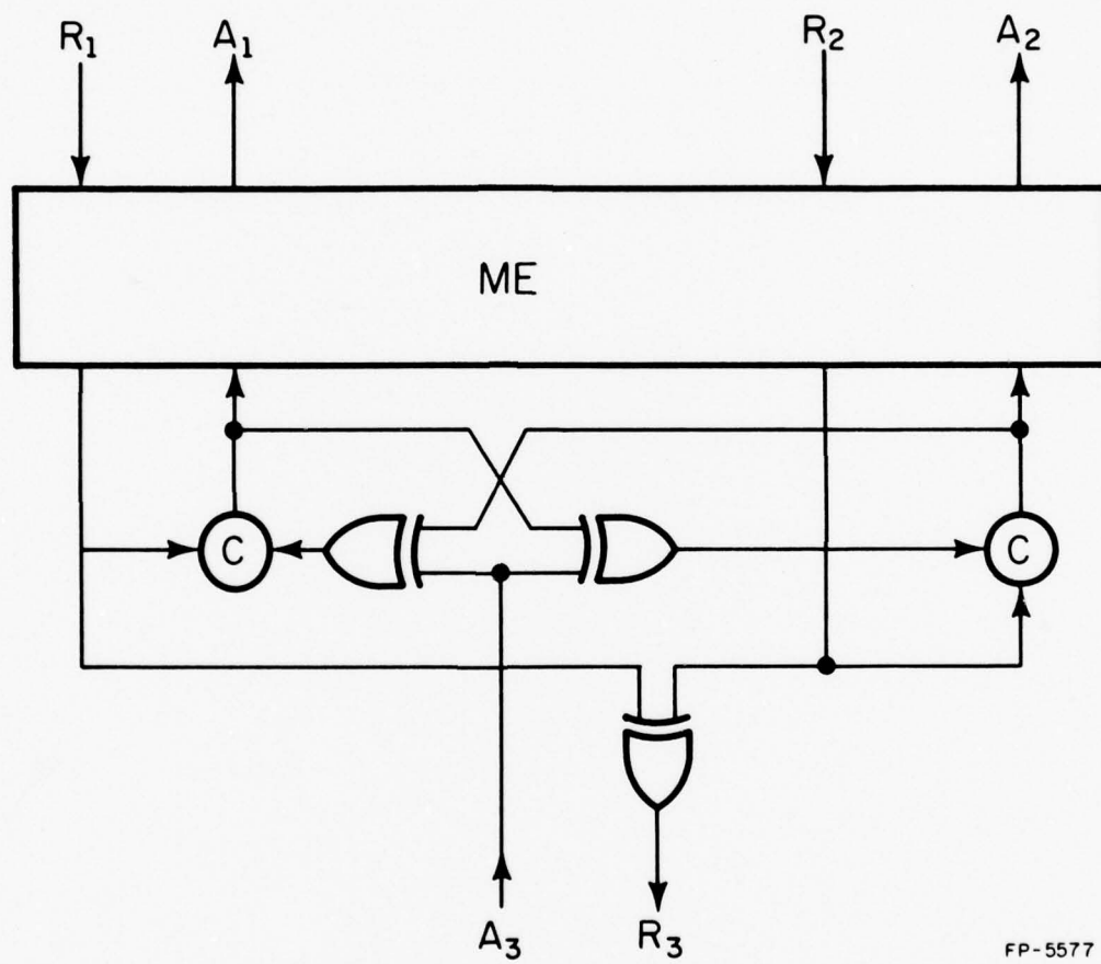
Figure 8.5. The SR Module (Simple Signalling).
