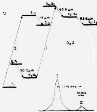
Fig. 2. Partial energy level diagram near the P(32) line. Insert shows the line positions and strengths based on conventional spectroscopic studies [4].
