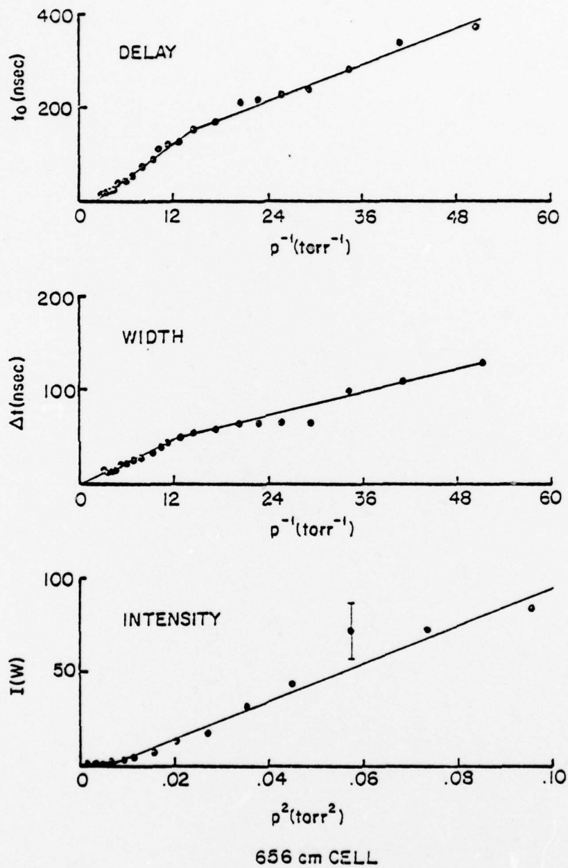
Fig. 4. Delay and pulsewidth vs. inverse pressure, and intensity vs. pressure squared for a 656 cm cell.
