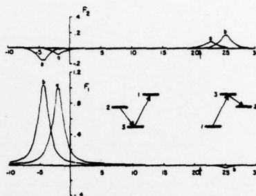
Fig. 6. Calculated values of F_1 and F_2 versus normalized FIR frequency 2(\nu_{32} - \nu_f)/\Delta\nu_H . Labels a and b refer to \beta values of 0.1 and 0.3, respectively, with \beta proportional to pump intensity as defined in the Appendix. The arrows show the pump location. Insert shows two possible Raman configurations.
