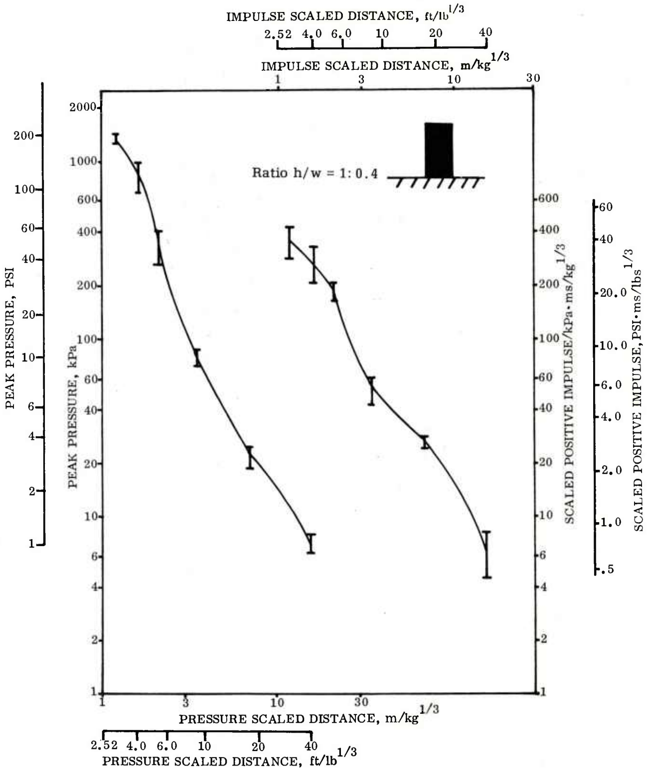
Figure 7. Pressure and Impulse vs. Scaled Distance, 45.4 kg Charge M-25 Stainless Steel Container Ratio h/w = 1:0.4 .
