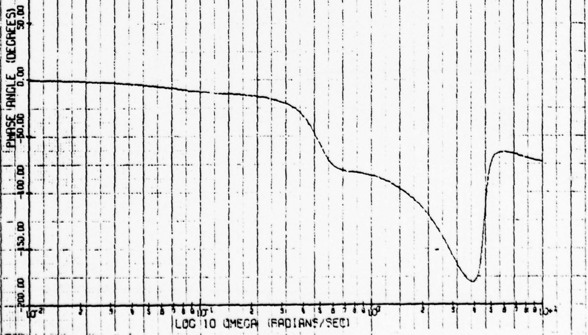
1. JW BODE PHASE PLOT
