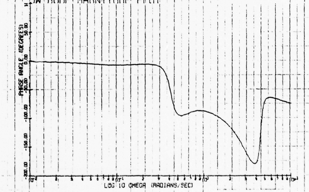
IW BODE PHASE PLOT
