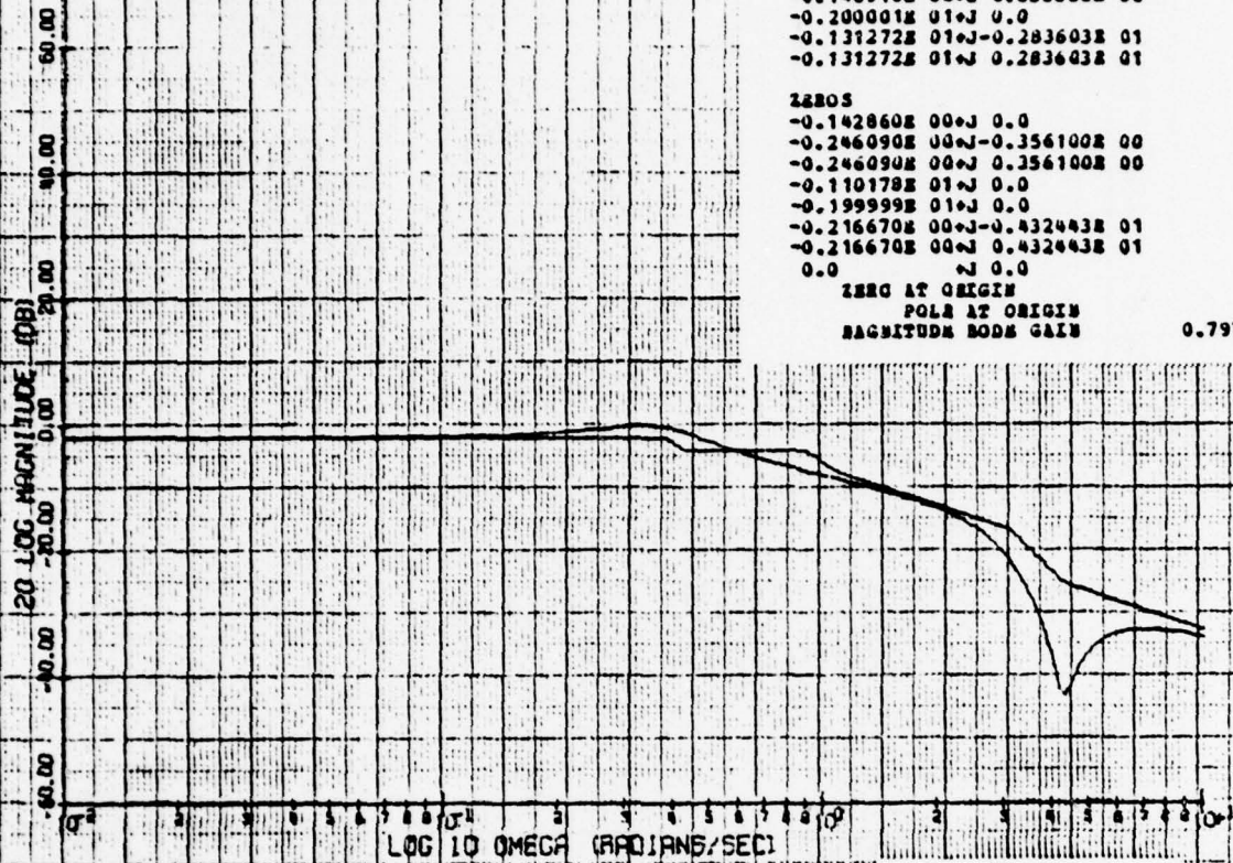
IN BODE MAGNITUDE PLOT
