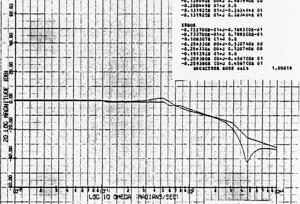
1. JW BODE MAGNITUDE PLOT
