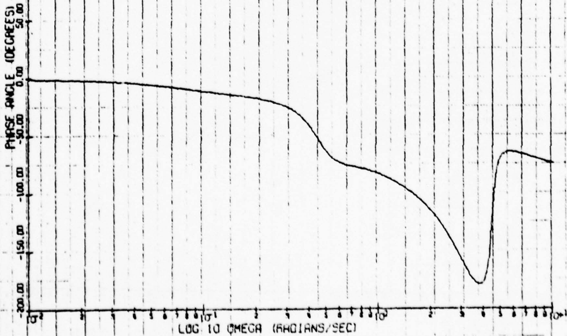
11 JW BODE PHASE PLOT
