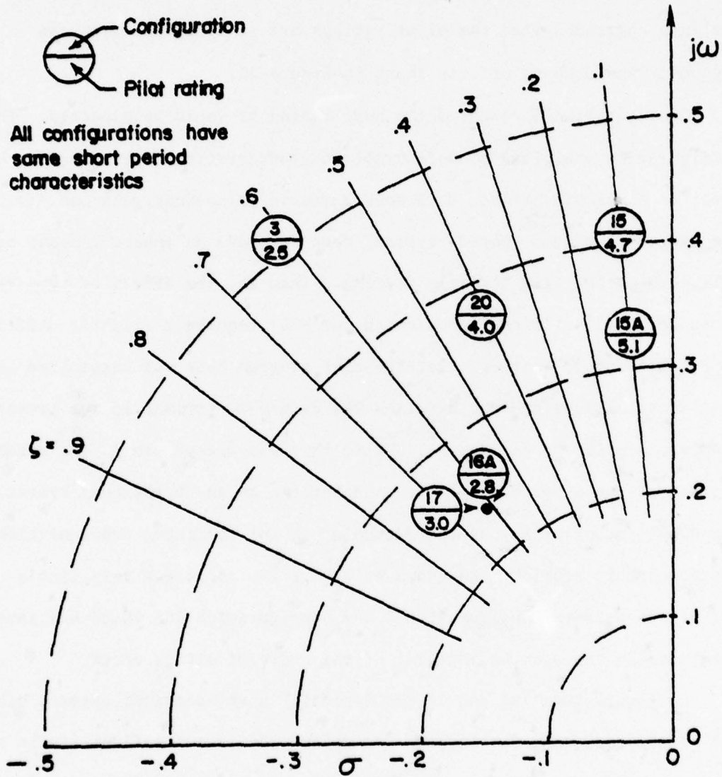
Figure 30. Predominant Mode Roots of Configurations and Their Pilot Ratings in Phase II In-Flight Simulation
