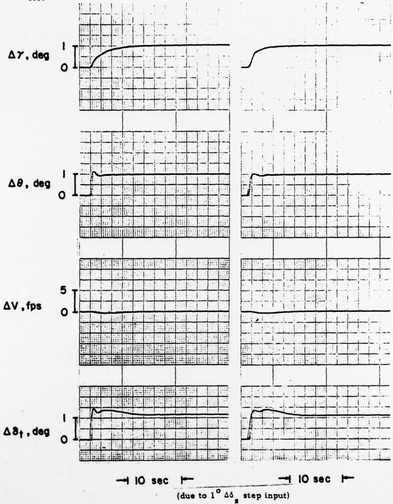
Figure B-5 Time History of Configurations 10 and 11
