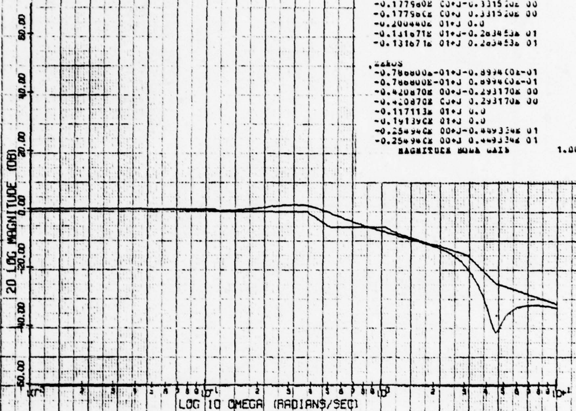
JW BODE MAGNITUDE PLOT
