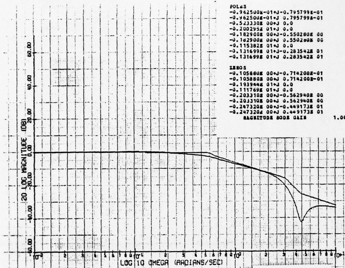
IN BODE MAGNITUDE PLOT
