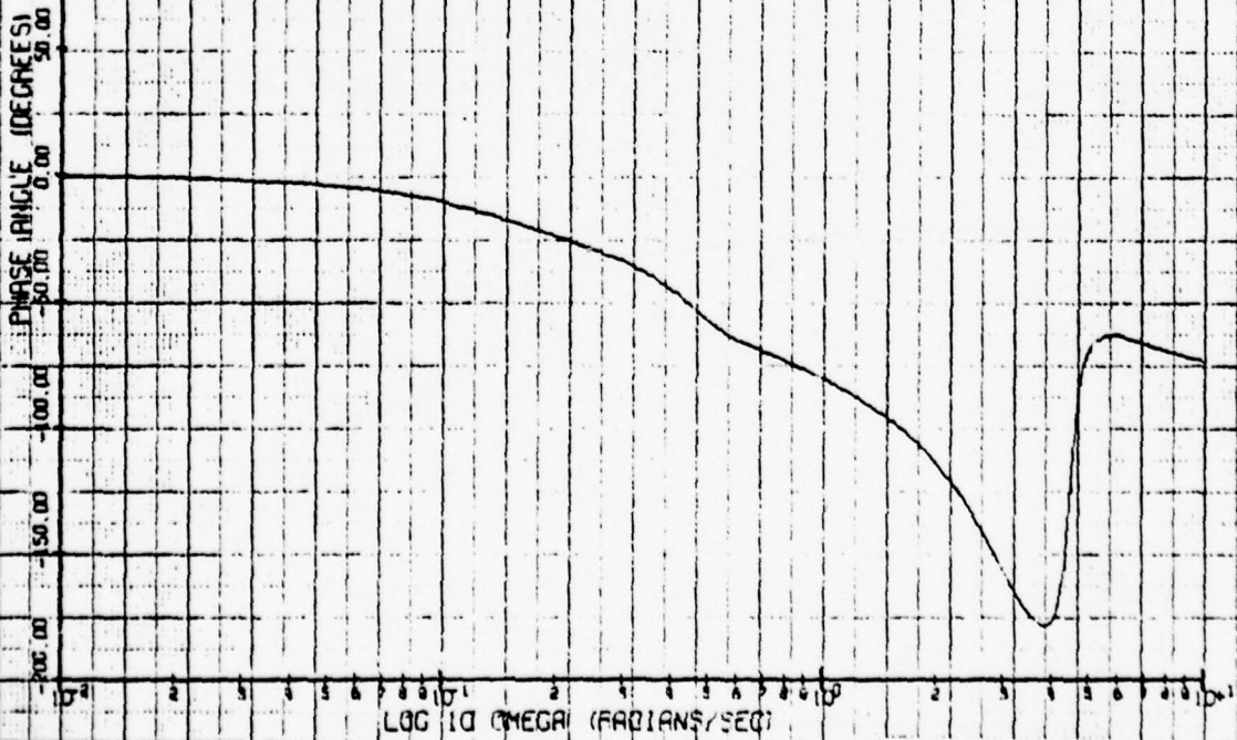
JW BODE PHASE PLOT
