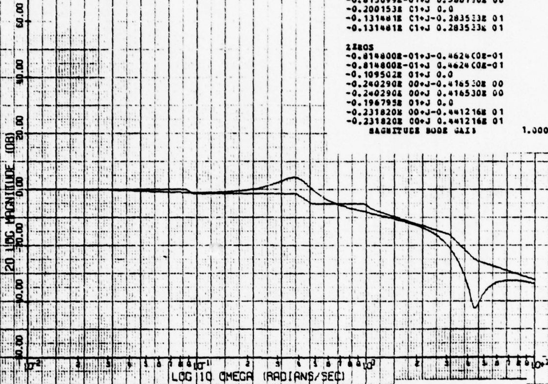
IW BODE MAGNITUDE PLOT
