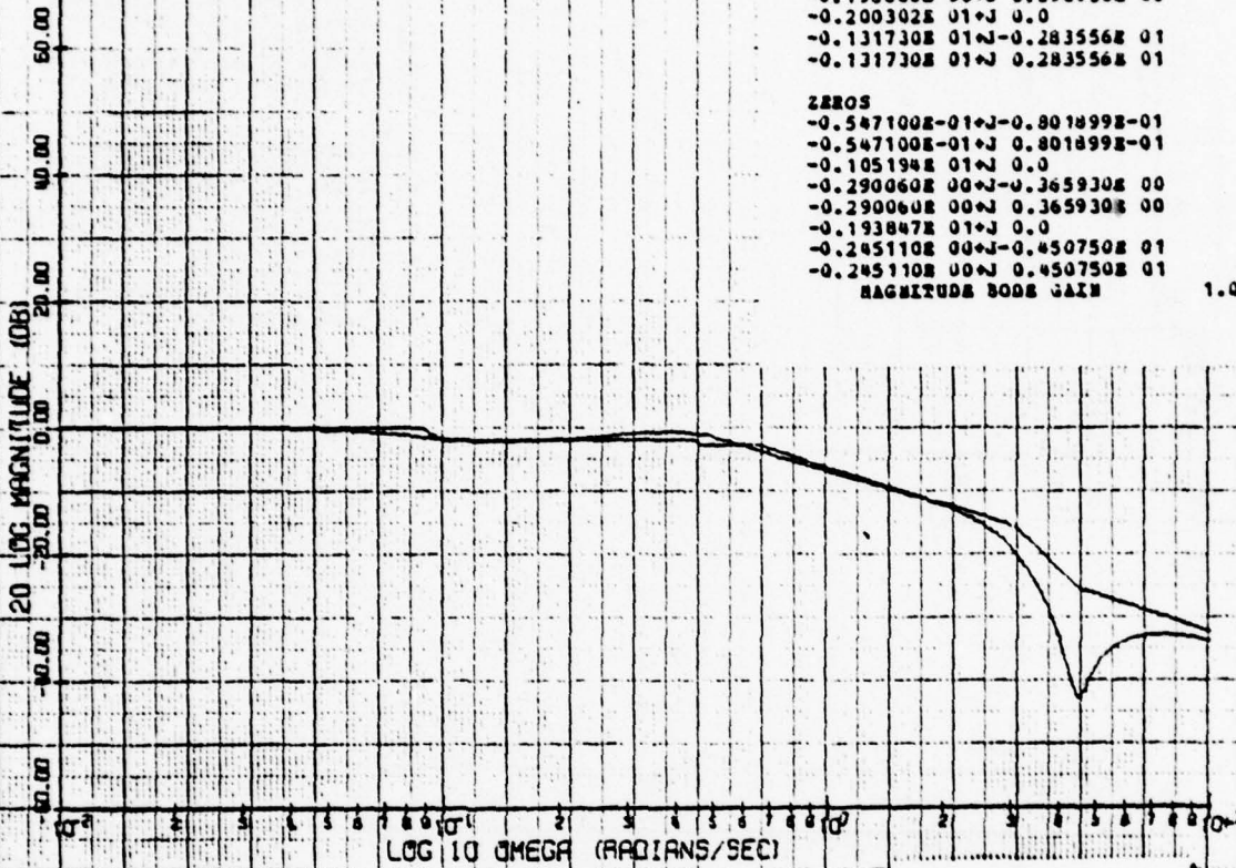
11 BW BODE MAGNITUDE PLOT
