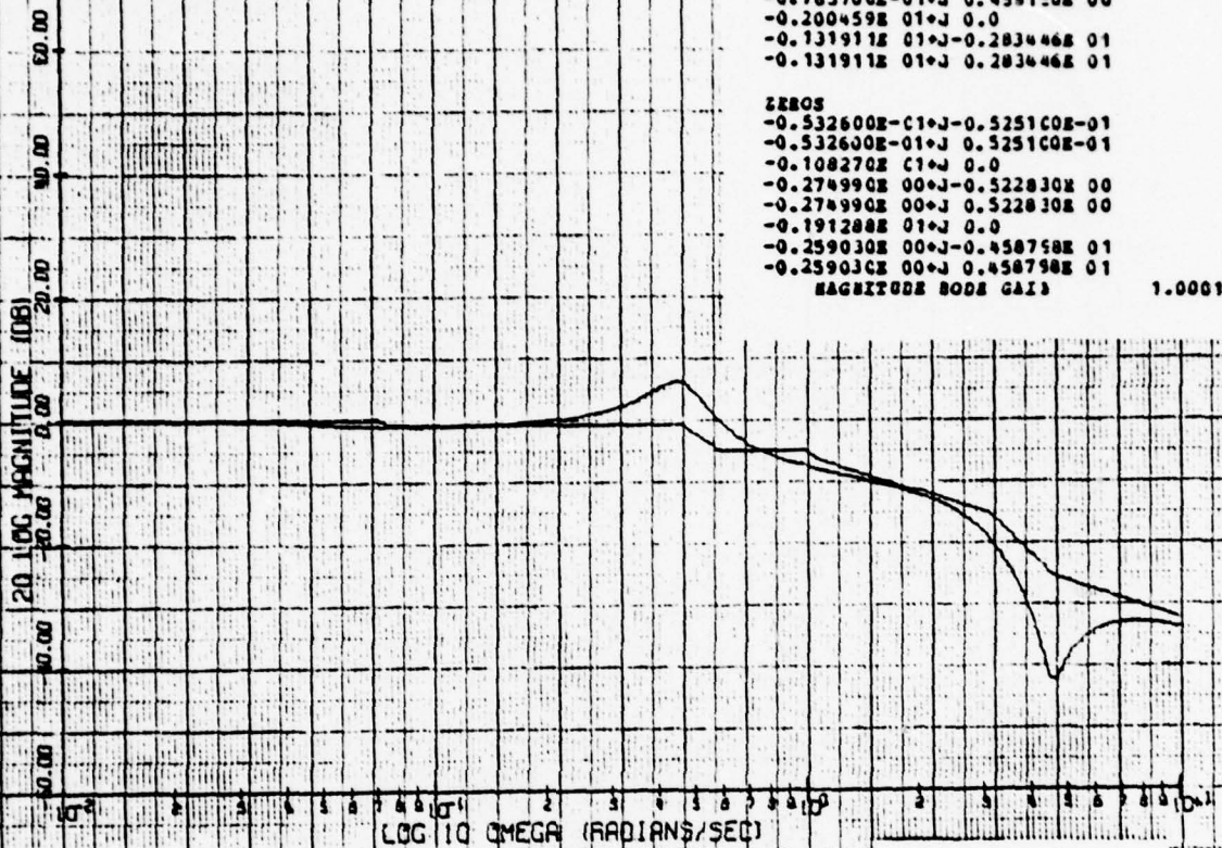
HW BODE MAGNITUDE PLOT
