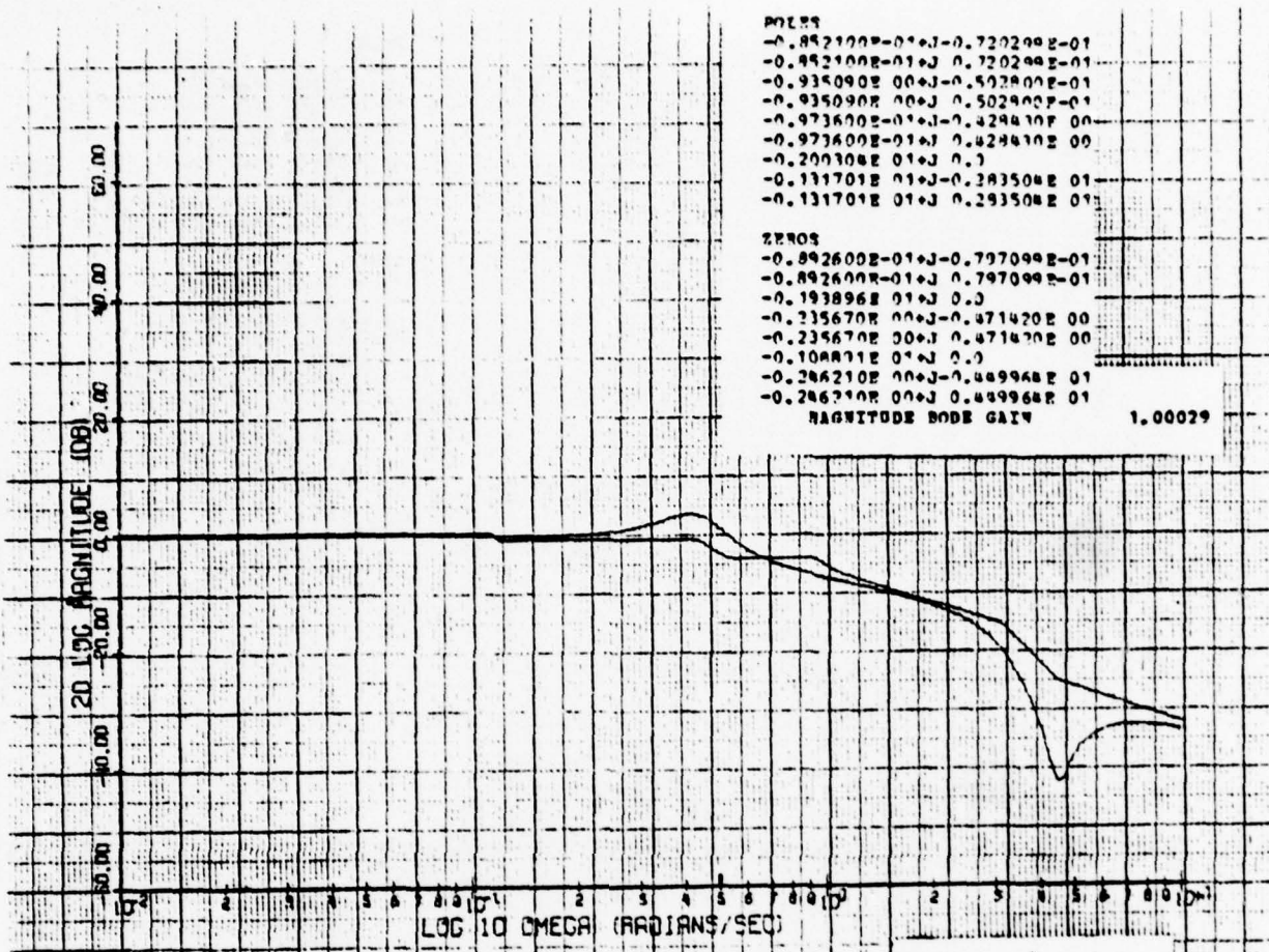
UW BODE MAGNITUDE PLOT
