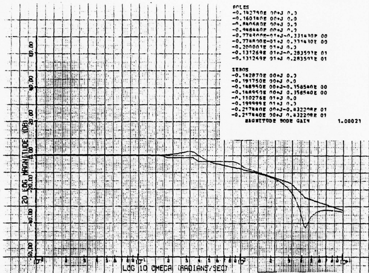
UW BODE MAGNITUDE PLOT
