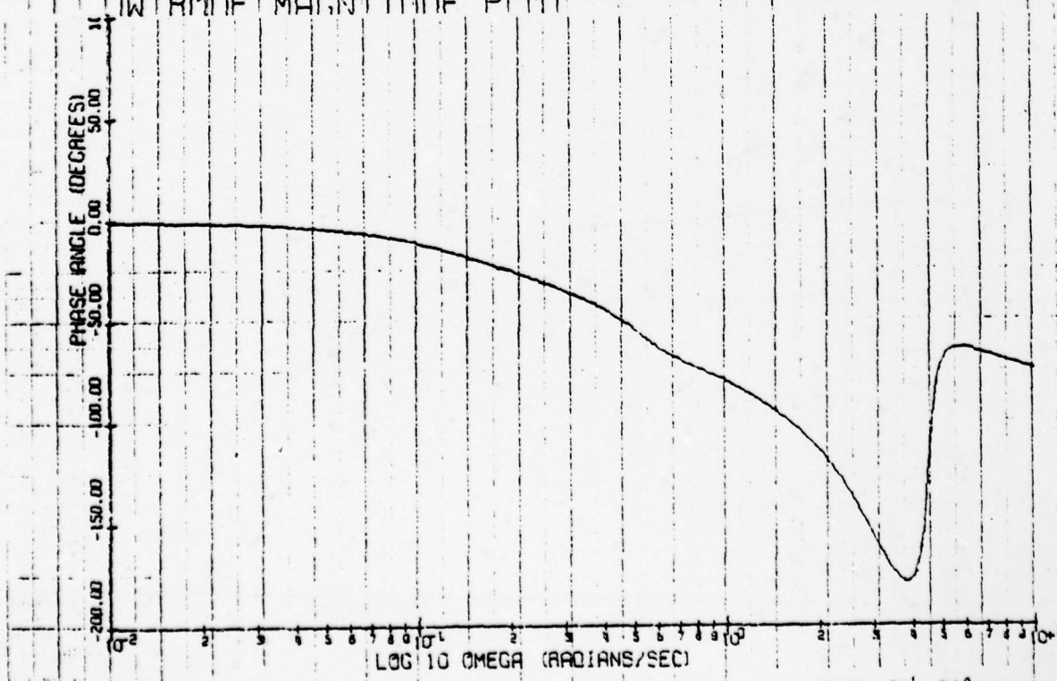
IN BODE PHASE PLOT
