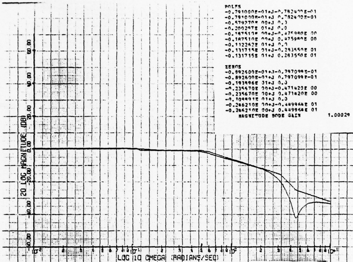
JW BODE MAGNITUDE PLOT
