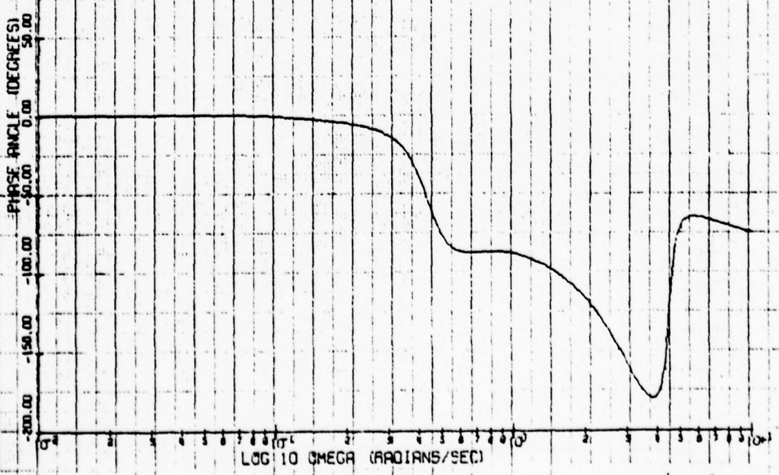
11 BODE PHASE PLOT
