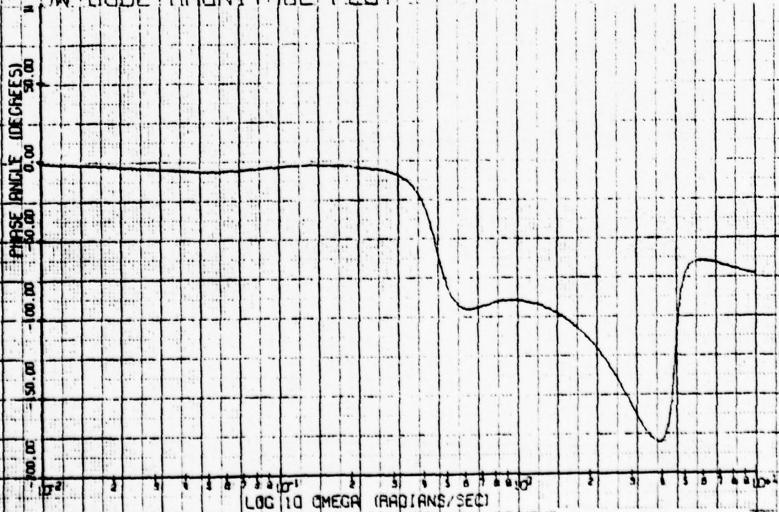
HW BODE PHASE PLOT
