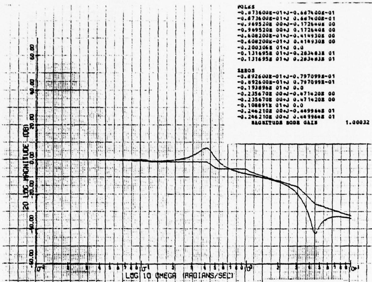
IW BODE MAGNITUDE PLOT
