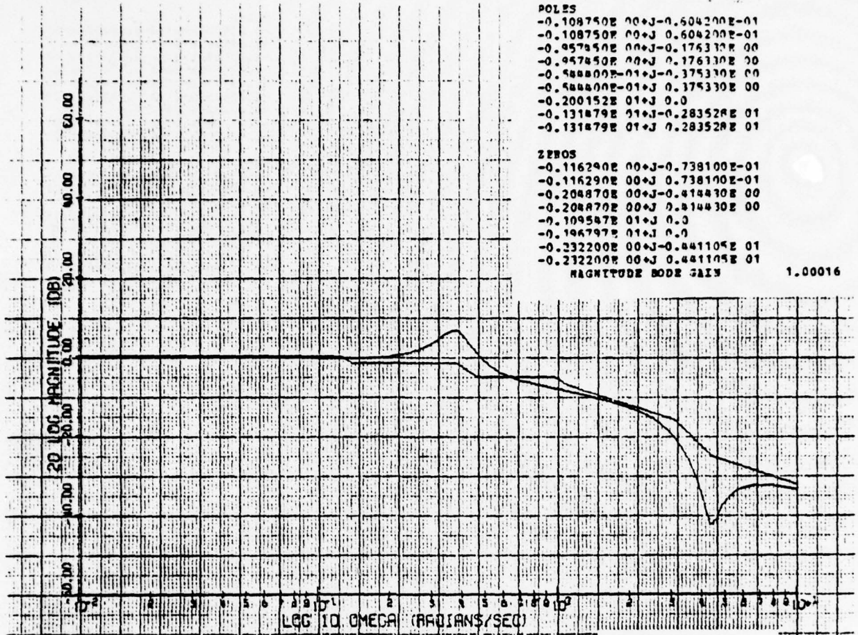
JW BODE MAGNITUDE PLOT
