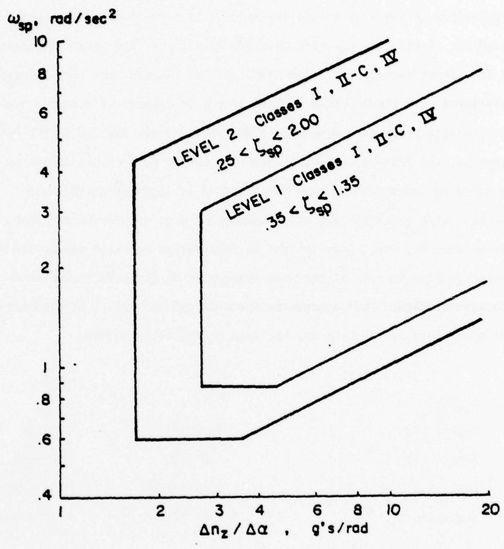
Figure 3. Short Period Frequency and Lift Curve Slope Requirements of Reference 9.
