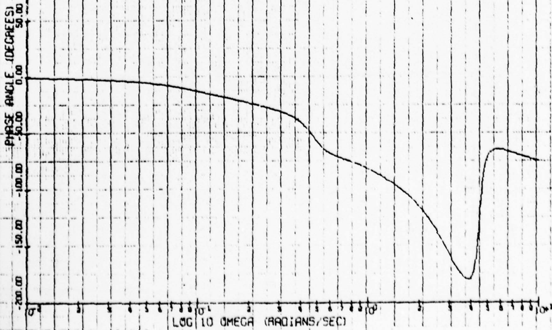
IW BODE PHASE PLOT
