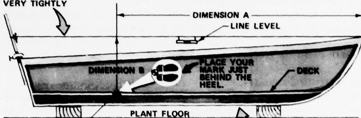
CUT-AWAY VIEW OF BOAT
