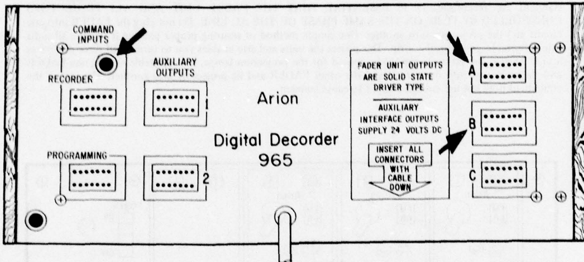
Figure B3. ARION 965 digital decoder - plug-in points.
