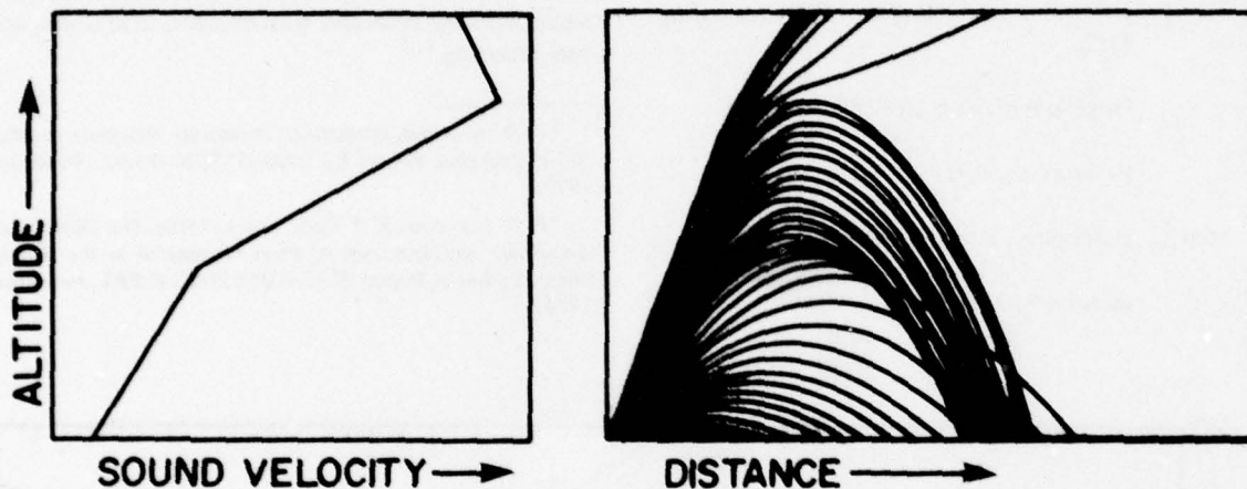
b. Vertical velocity gradient with two segments.
