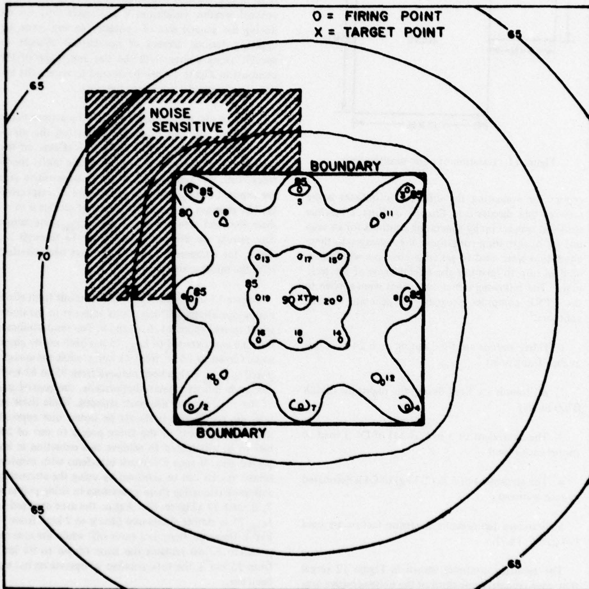
Figure 12. Noise contours of initial conditions (Case II).
