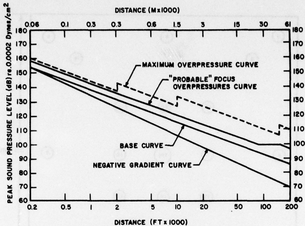
Figure 4. Effects of weather on blast amplitude.
