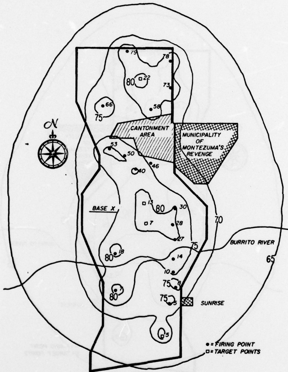
Figure 26. Effects of relocating operations from point 46.
