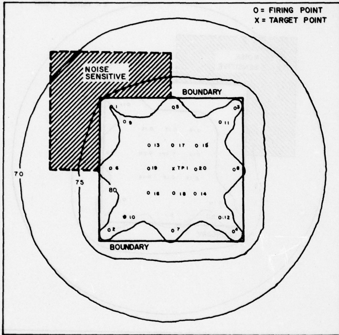
Figure 15. Effects of rescheduling operations at point 1.
