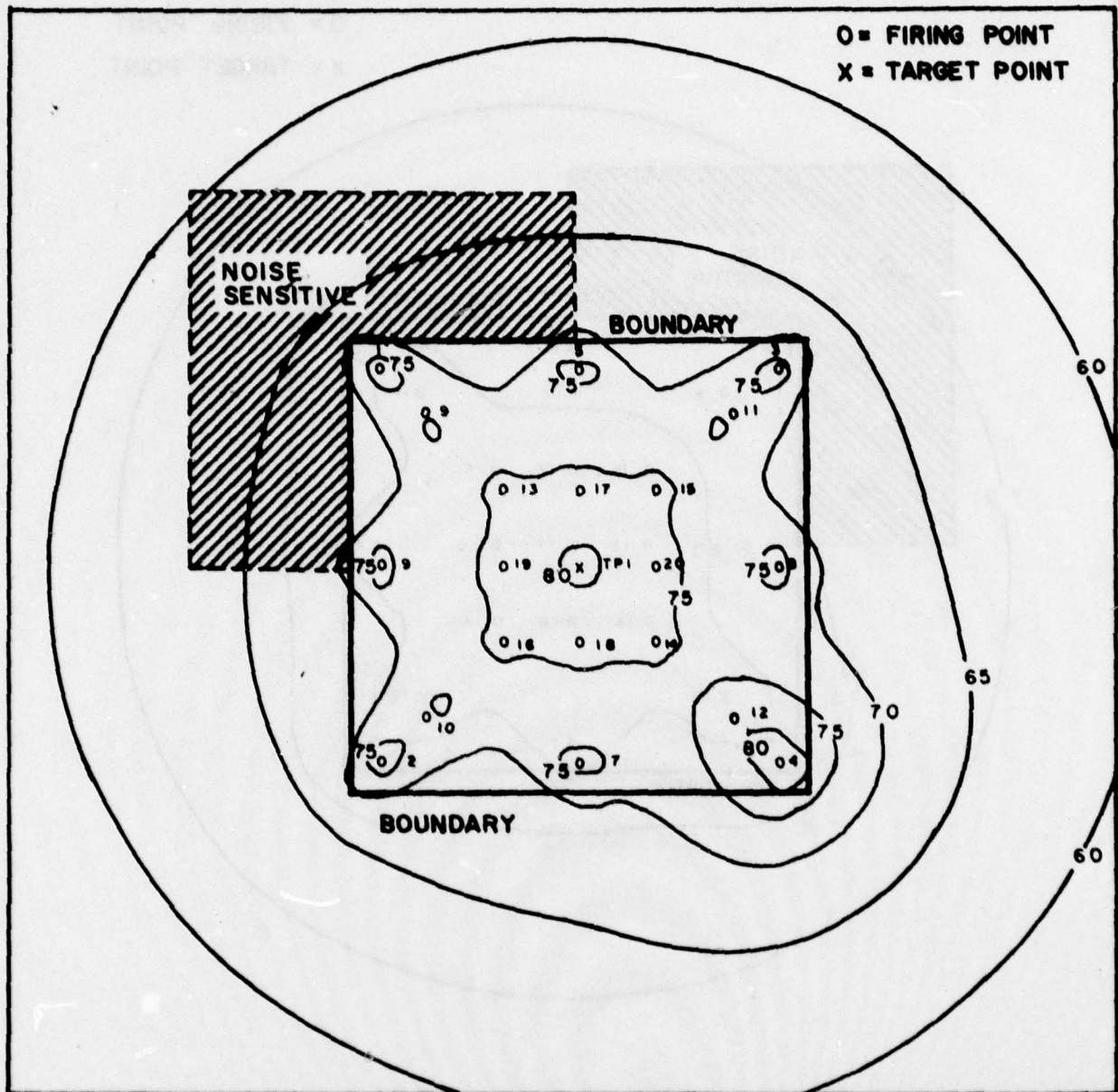
Figure 17. Effects of rescheduling most operations.
