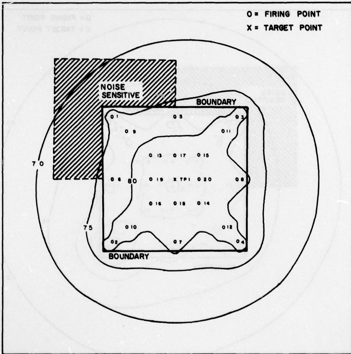
Figure 16. Effects of rescheduling operations at points 1, 5, 6, and 9.
