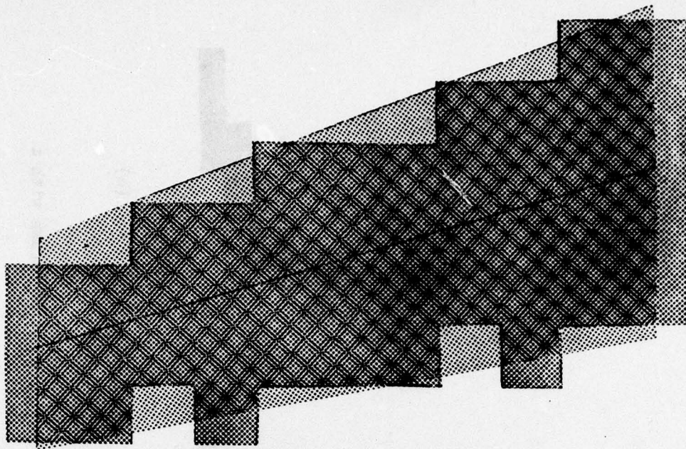
Figure 19. Failure of monotonicity due to independent rounding. (Rounding takes (w, x, y) into (\lfloor w \rfloor, \lfloor x - \delta(\lfloor w \rfloor) \rfloor, \lfloor y \rfloor) .)
